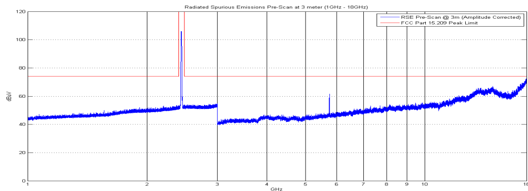
Plot 6-33. Radiated Spurious Plot above 1GHz (802.11b – Ch. 6, Ant. Pol. H)
