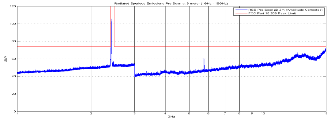
Plot 6-31. Radiated Spurious Plot above 1GHz (802.11b – Ch. 1, Ant. Pol. H)
