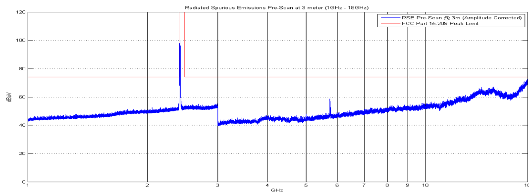
Plot 6-32. Radiated Spurious Plot above 1GHz (802.11b – Ch. 1, Ant. Pol. V)
