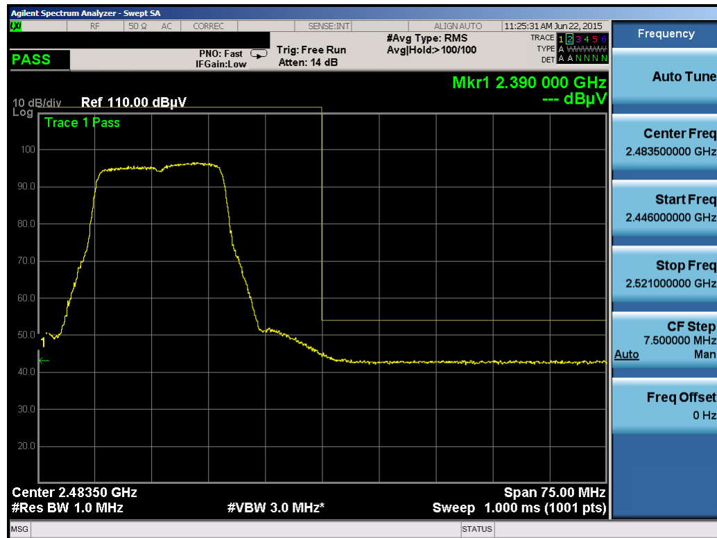
Plot 6-41. Radiated Restricted Upper Band Edge Measurement (Average)
