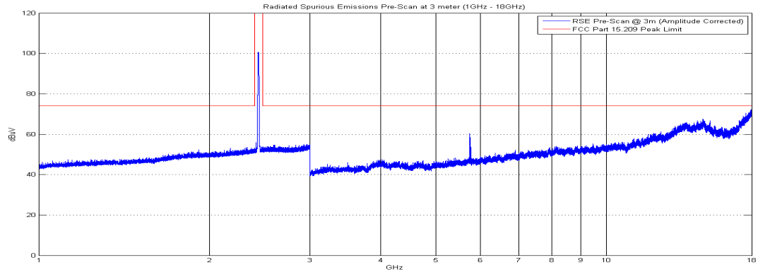
Plot 6-34. Radiated Spurious Plot above 1GHz (802.11b – Ch. 6, Ant. Pol. V)
