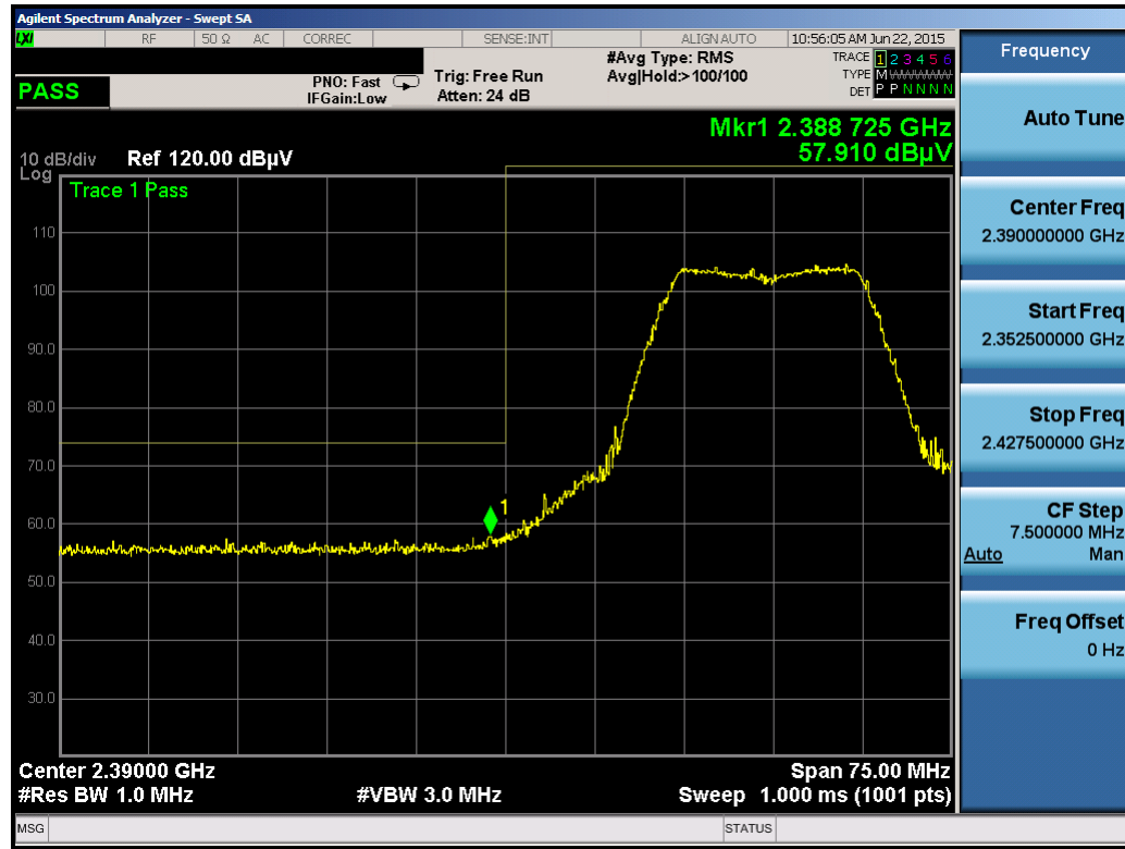
Plot 6-40. Radiated Restricted Lower Band Edge Measurement (Peak)
