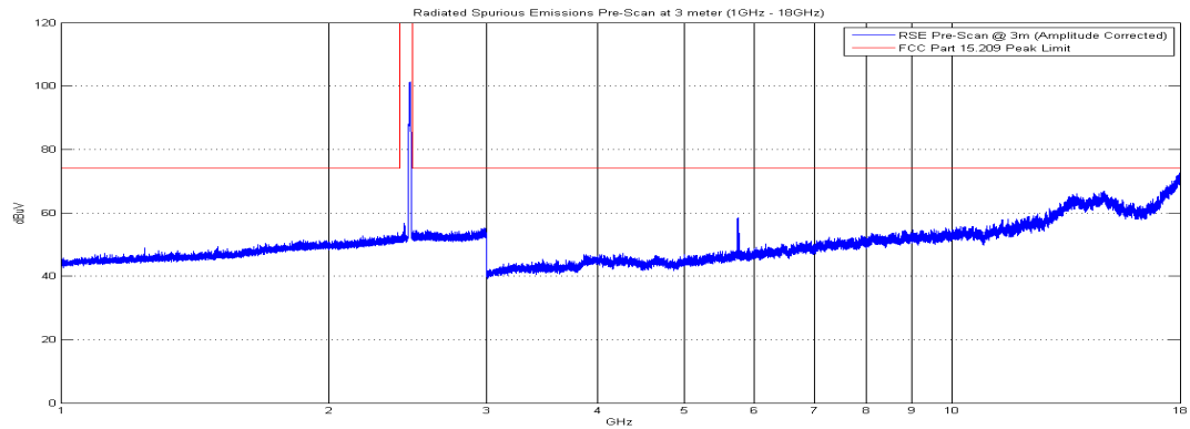
Plot 6-36. Radiated Spurious Plot above 1GHz (802.11b – Ch. 11, Ant. Pol. V)
