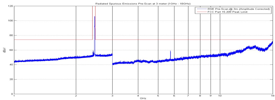
Plot 6-35. Radiated Spurious Plot above 1GHz (802.11b – Ch. 11, Ant. Pol. H)
