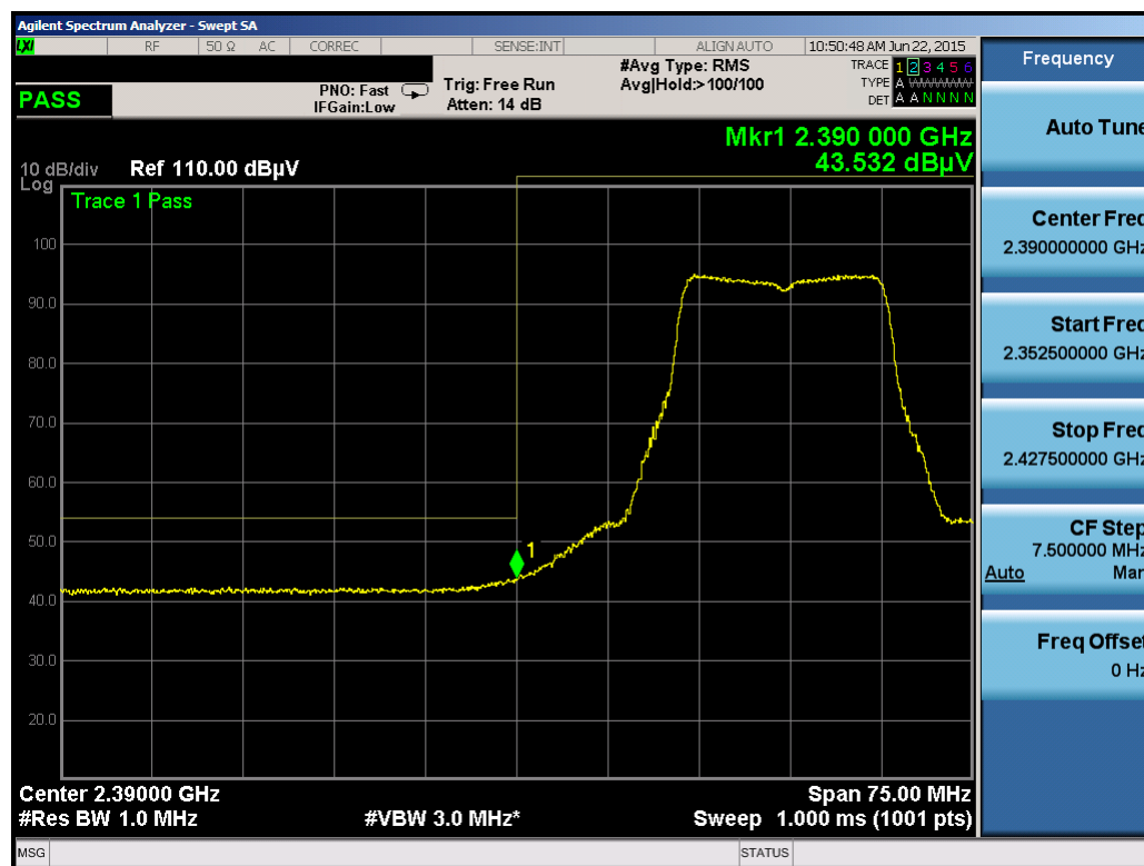
Plot 6-39. Radiated Restricted Lower Band Edge Measurement (Average)
