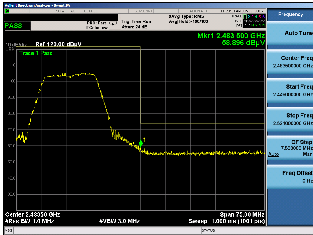
Plot 6-42. Radiated Restricted Upper Band Edge Measurement (Peak)
