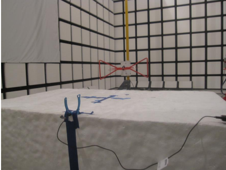
RADIATED BACK PHOTO (BELOW 1 GHz) – USB ADAPTER
