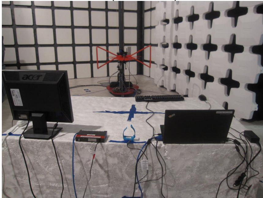
RADIATED BACK PHOTO (BELOW 1 GHz) – LAPTOP
