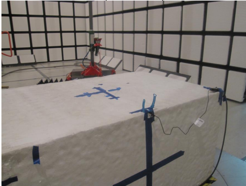
RADIATED BACK PHOTO (ABOVE 1 GHz) – USB ADAPTER
