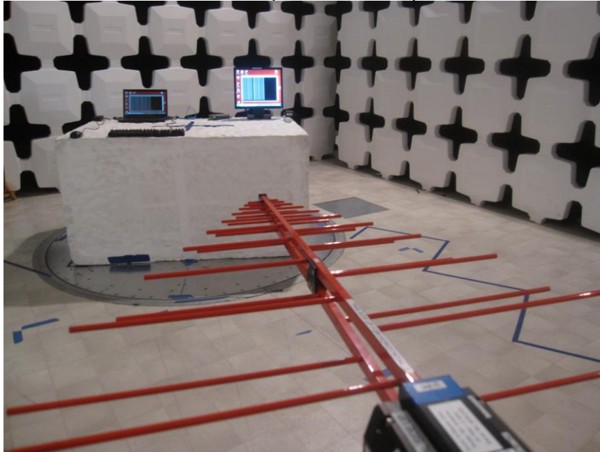
RADIATED FRONT PHOTO (BELOW 1 GHz) – LAPTOP
