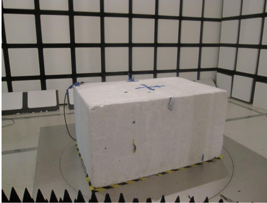
RADIATED FRONT PHOTO (ABOVE 1 GHz) – USB ADAPTER
