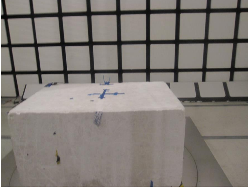
RADIATED FRONT PHOTO (BELOW 1 GHz) – USB ADAPTER
