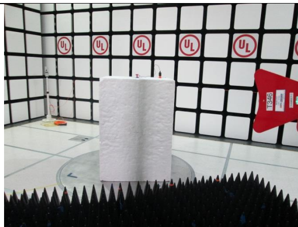
RADIATED PHOTO (ABOVE 1 GHz)
