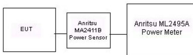
Figure 8-1 Power Measurement Setup
