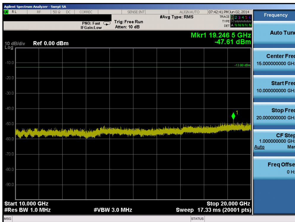
Plot 6-18. Conducted Spurious Plot (Band 4 – 5.0MHz QPSK – RB Size 1, RB Offset 0 – High Channel)
