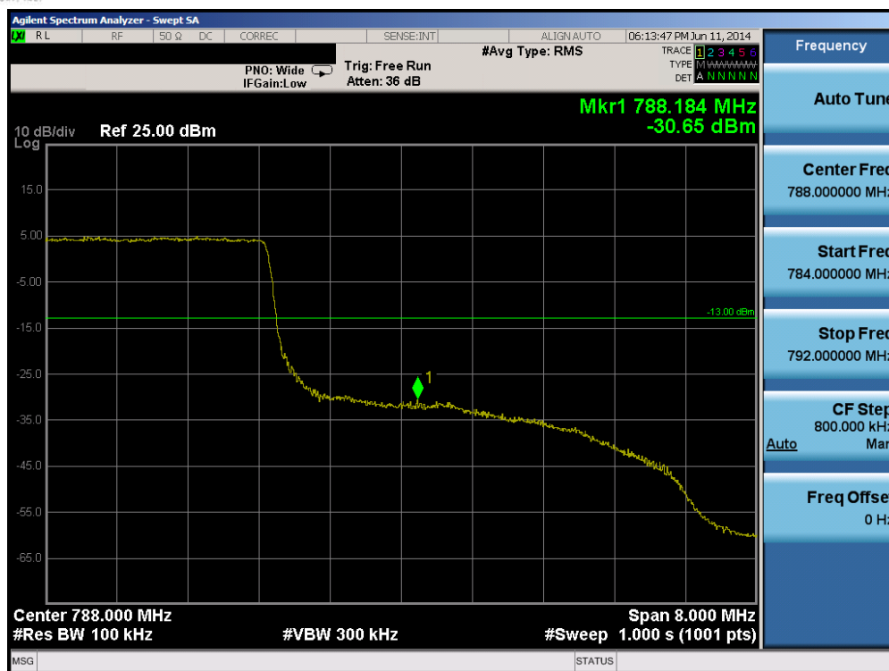
Plot 6-21. Upper Band Edge Plot (Band 13 – 10.0MHz QPSK – RB Size 50)
