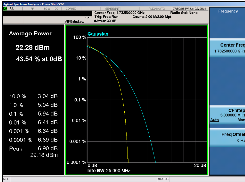
Plot 6-46. PAR Plot (Band 4 – 15.0MHz 16-QAM – RB Size 75)
