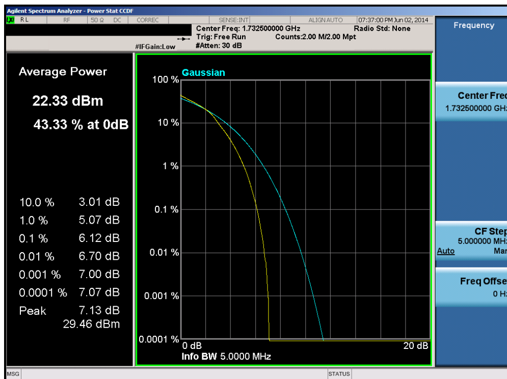
Plot 6-42. PAR Plot (Band 4 – 5.0MHz 16-QAM – RB Size 25)
