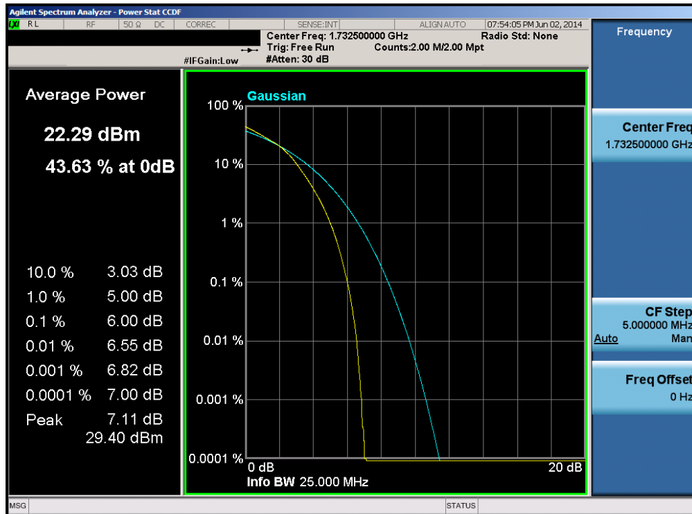
Plot 6-48. PAR Plot (Band 4 – 20.0MHz 16-QAM – RB Size 100)
