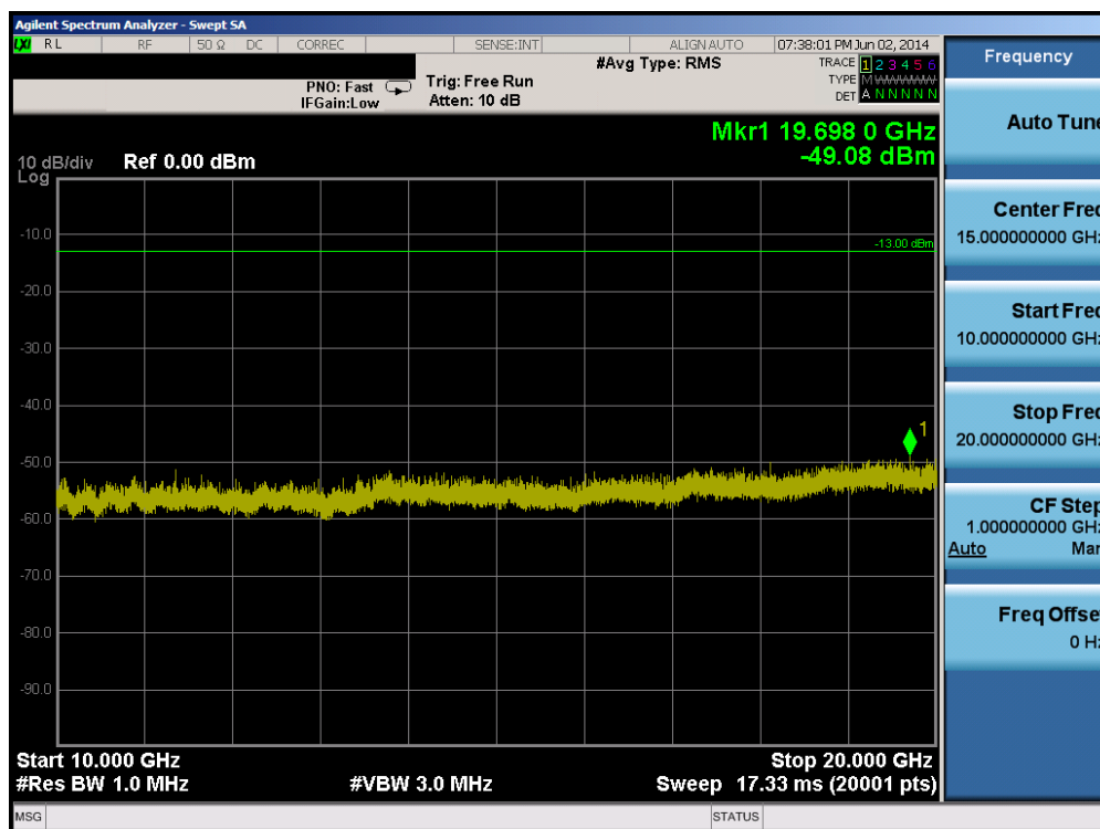
Plot 6-16. Conducted Spurious Plot (Band 4 – 5.0MHz QPSK – RB Size 1, RB Offset 0 – Mid Channel)
