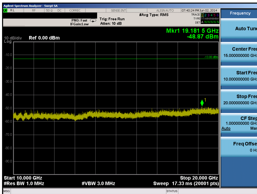
Plot 6-14. Conducted Spurious Plot (Band 4 – 5.0MHz QPSK – RB Size 1, RB Offset 0 – Low Channel)
