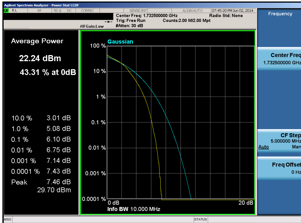
Plot 6-44. PAR Plot (Band 4 – 10.0MHz 16-QAM – RB Size 50)
