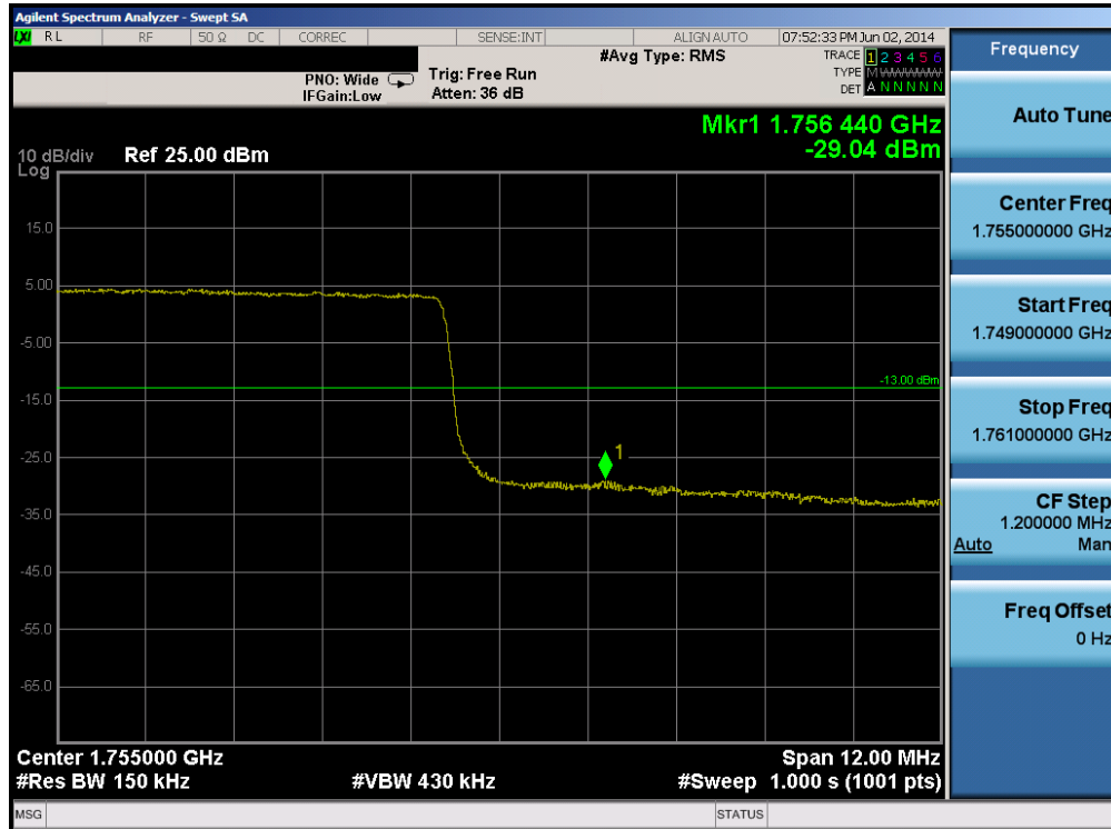
Plot 6-33. Upper Band Edge Plot (Band 4 – 15.0MHz QPSK – RB Size 75)
