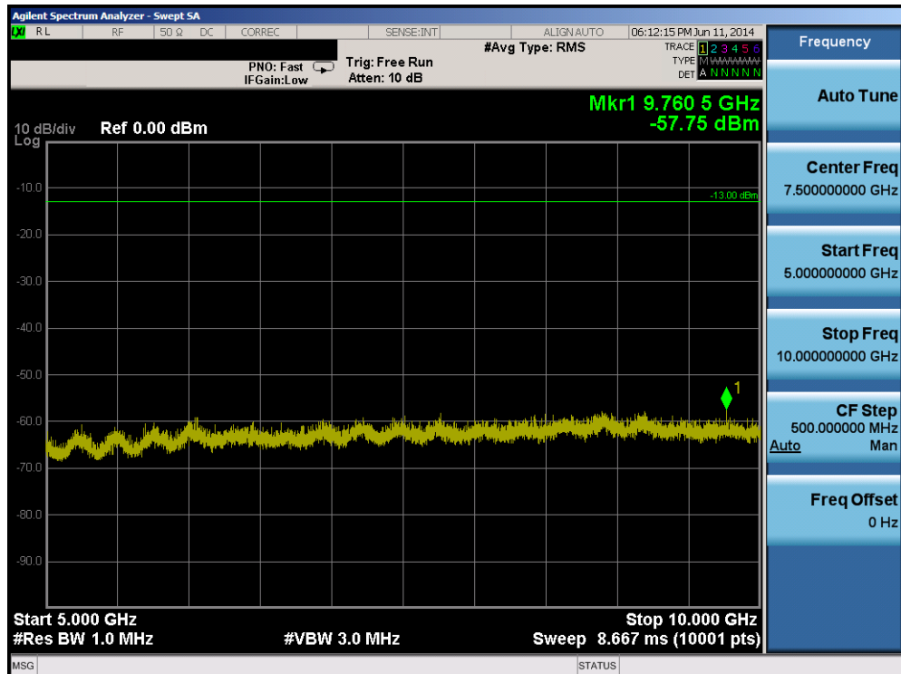
Plot 6-12. Conducted Spurious Plot (Band 13 – 10.0MHz QPSK – RB Size 1, RB Offset 0)
