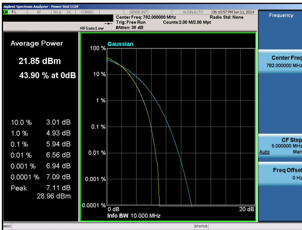
Plot 6-40. PAR Plot (Band 13 – 10.0MHz 16-QAM – RB Size 25)
