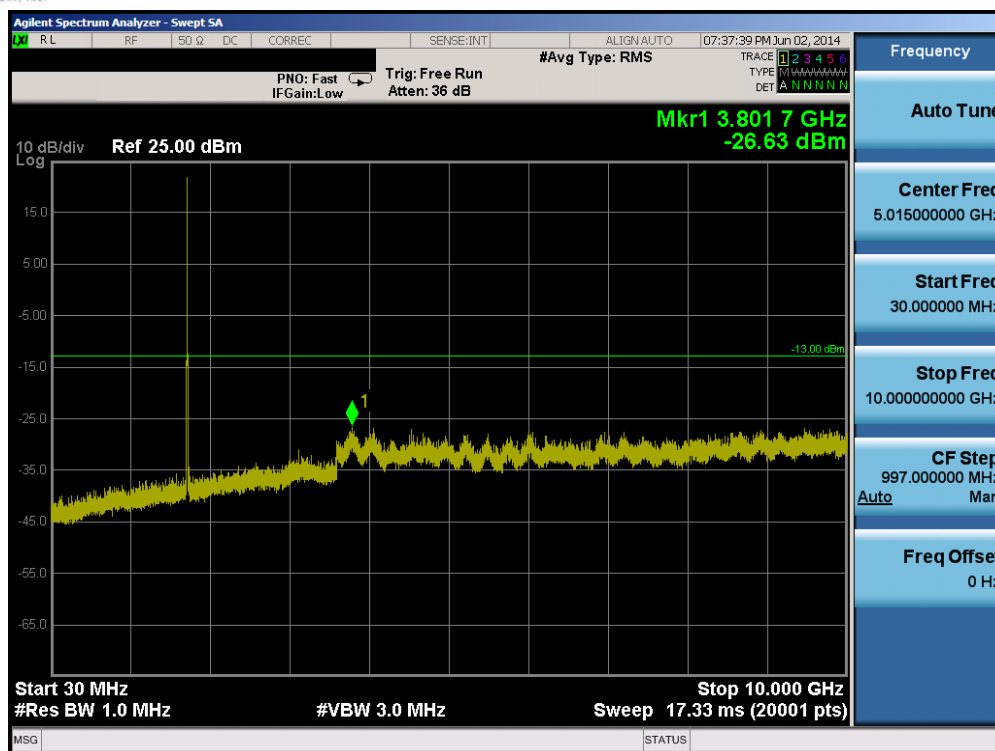
Plot 6-15. Conducted Spurious Plot (Band 4 – 5.0MHz QPSK – RB Size 1, RB Offset 0 – Mid Channel)
