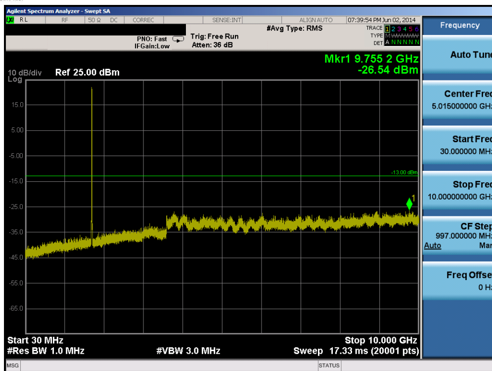
Plot 6-13. Conducted Spurious Plot (Band 4 – 5.0MHz QPSK – RB Size 1, RB Offset 0 – Low Channel)
