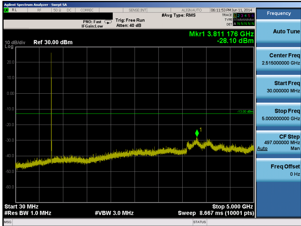
Plot 6-11. Conducted Spurious Plot (Band 13 – 10.0MHz QPSK – RB Size 1, RB Offset 0)
