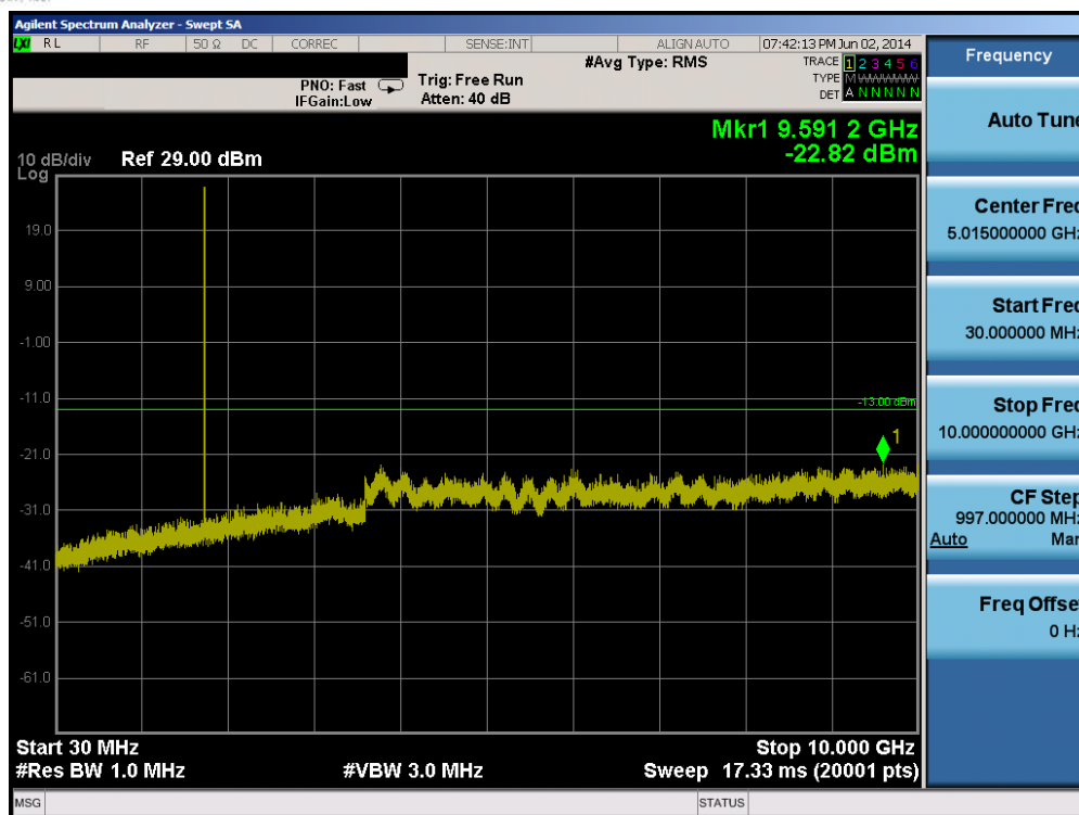
Plot 6-17. Conducted Spurious Plot (Band 4 – 5.0MHz QPSK – RB Size 1, RB Offset 0 – High Channel)
