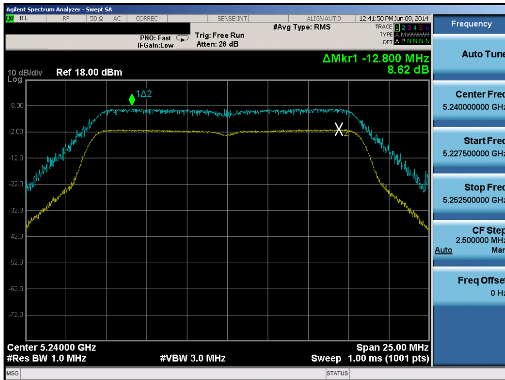
Plot 6-56. Peak Excursion Ratio Plot (802.11a (UNII Band 1) – Ch. 48)
