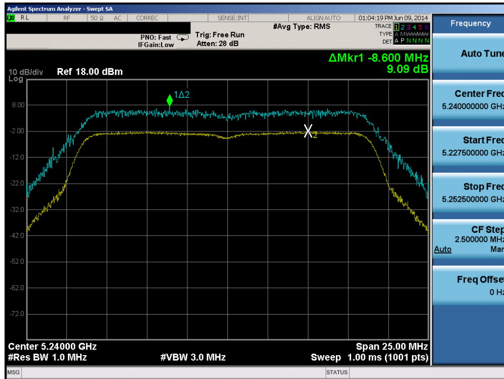
Plot 6-57. Peak Excursion Ratio Plot (20MHz BW 802.11n (UNII Band 1) – Ch. 48)
