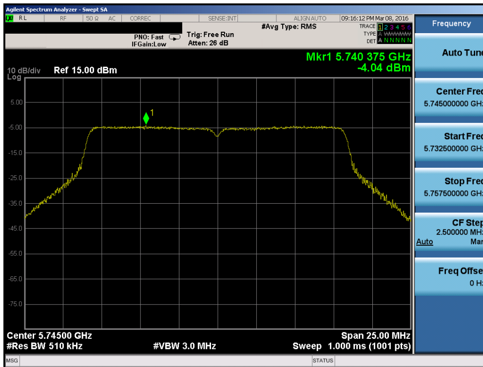
Plot 7-1. Power Spectral Density Plot (802.11a (UNII Band 3) – Ch. 149)
