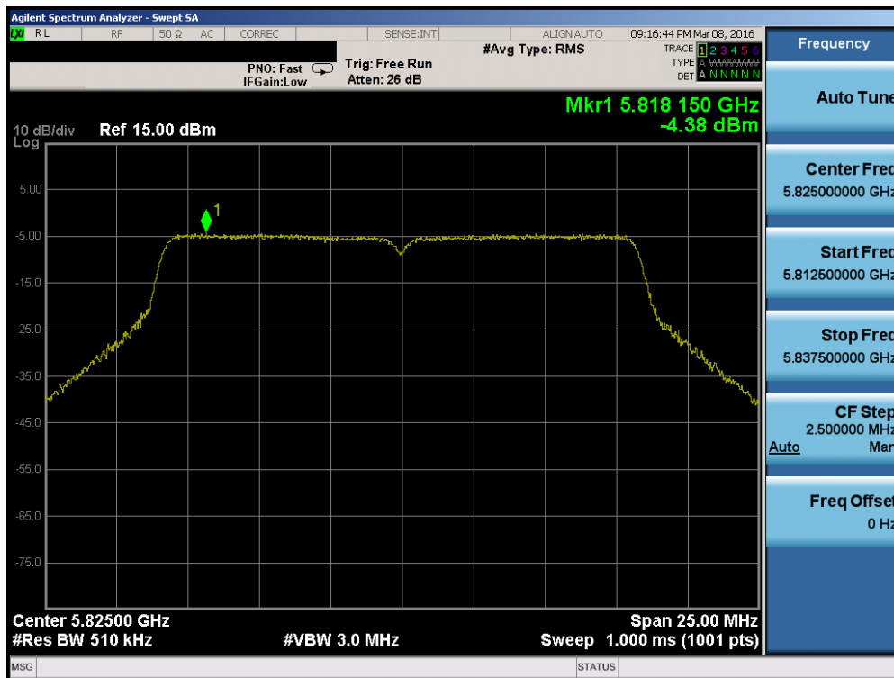
Plot 7-3. Power Spectral Density Plot (802.11a (UNII Band 3) – Ch. 165)
