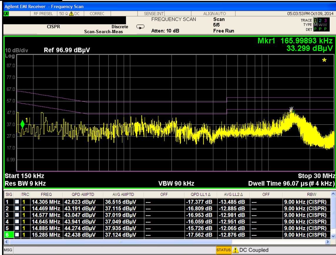
Plot 6-21. Line Conducted Plot with Bluetooth LE (N)
