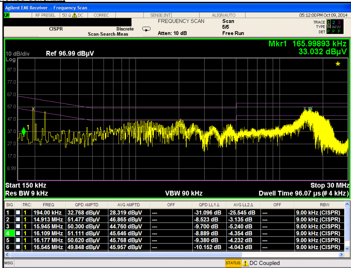
Plot 6-20. Line Conducted Plot with Bluetooth LE (L1)
