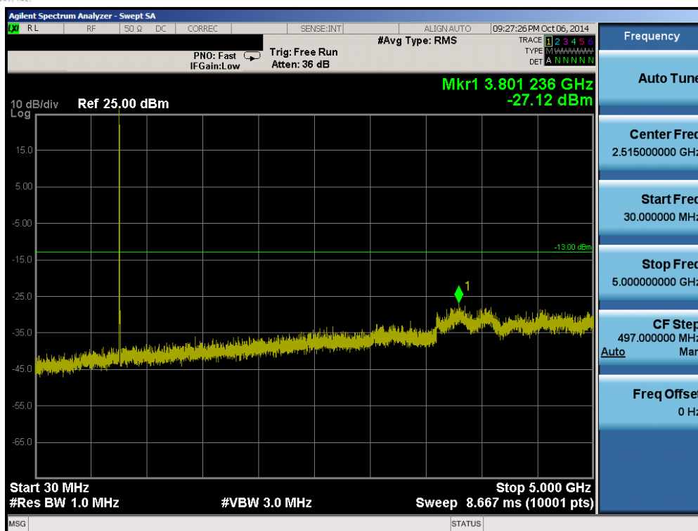
Plot 6-11. Conducted Spurious Plot (Band 13 – 10.0MHz QPSK – RB Size 1, RB Offset 0 – Mid Channel)
