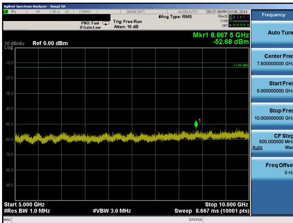
Plot 6-12. Conducted Spurious Plot (Band 13 – 10.0MHz QPSK – RB Size 1, RB Offset 0 – Mid Channel)
