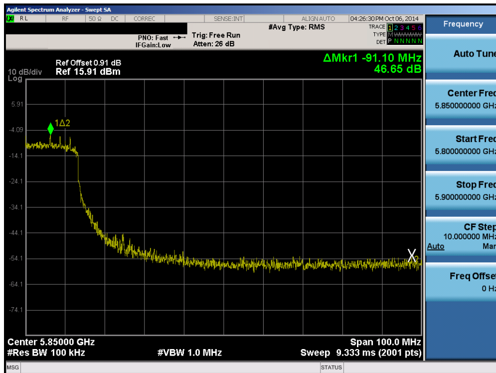
Plot 6-46. Band Edge Plot (40MHz BW 802.11n (5.8GHz) – Ch. 161)
