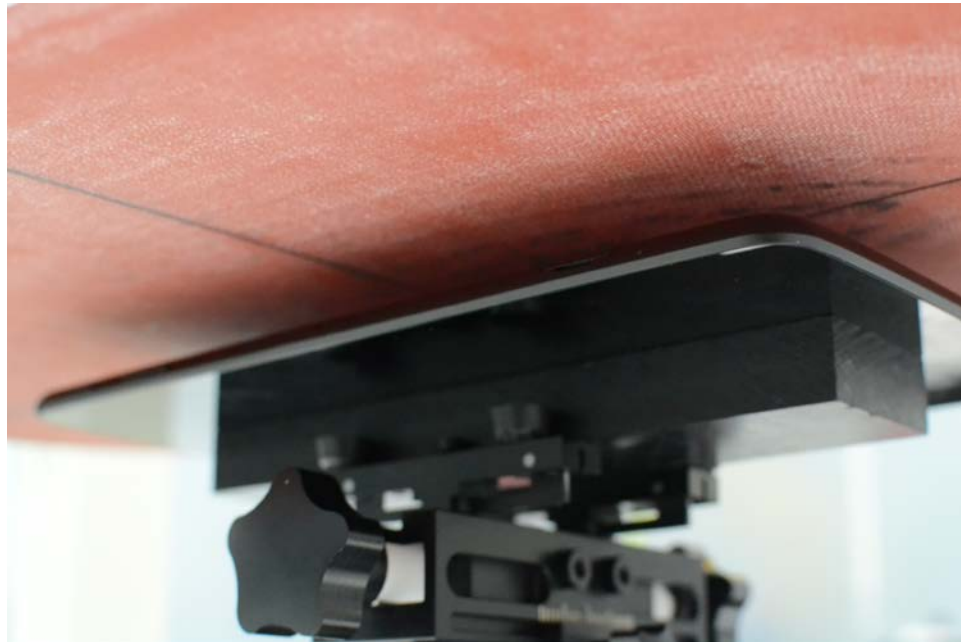
SAR Test Setup Photo 2: Back Side at 17 mm
