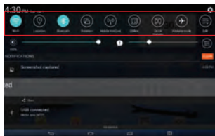
Notifications panel
