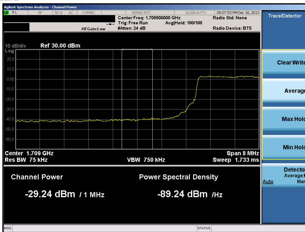
Plot 8-16. Lower Extended Band Edge Plot (10.0MHz QPSK – RB Size 50)
