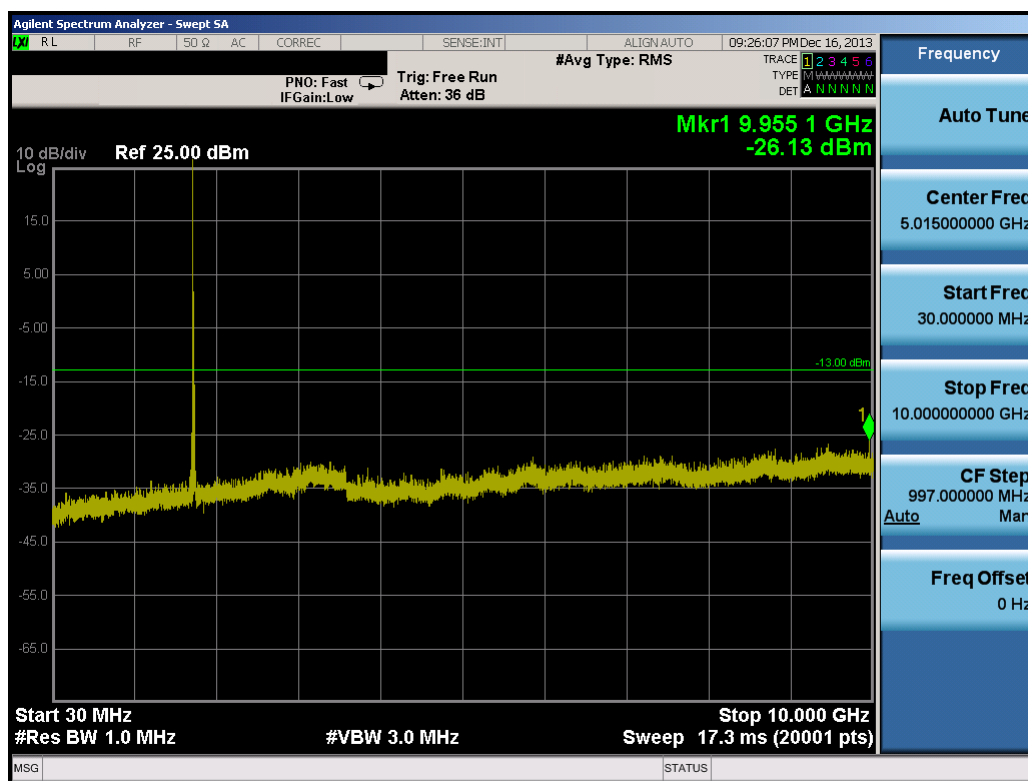
Plot 8-51. Conducted Spurious Plot (20.0MHz QPSK – RB Size 1, RB Offset 0 – High Channel)
