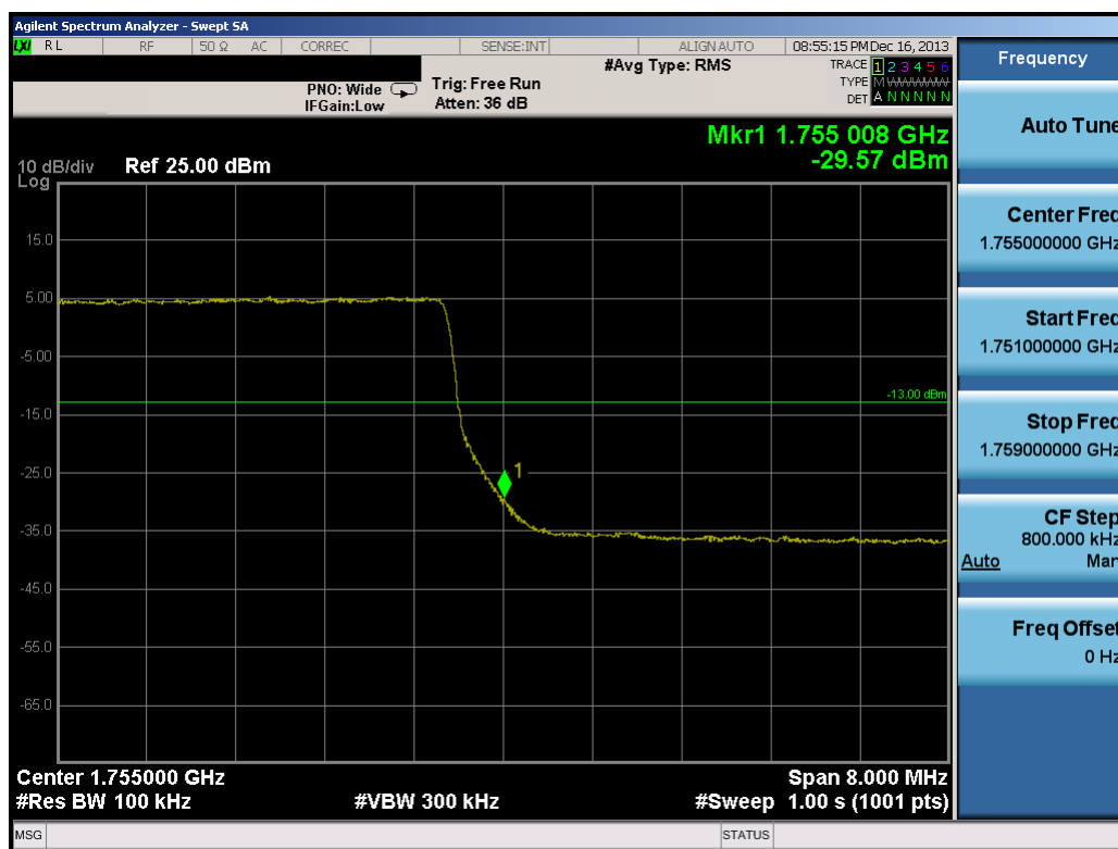
Plot 8-25. Upper Band Edge Plot (10.0MHz QPSK – RB Size 50)
