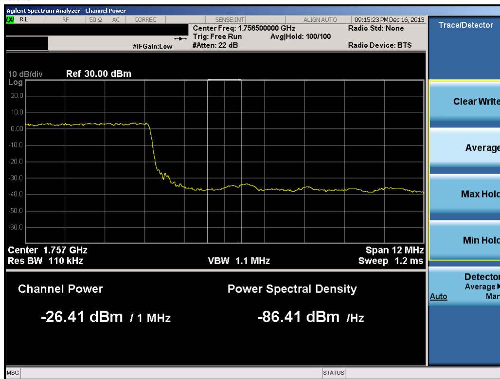
Plot 8-40. Upper Extended Band Edge Plot (15.0MHz QPSK – RB Size 75)
