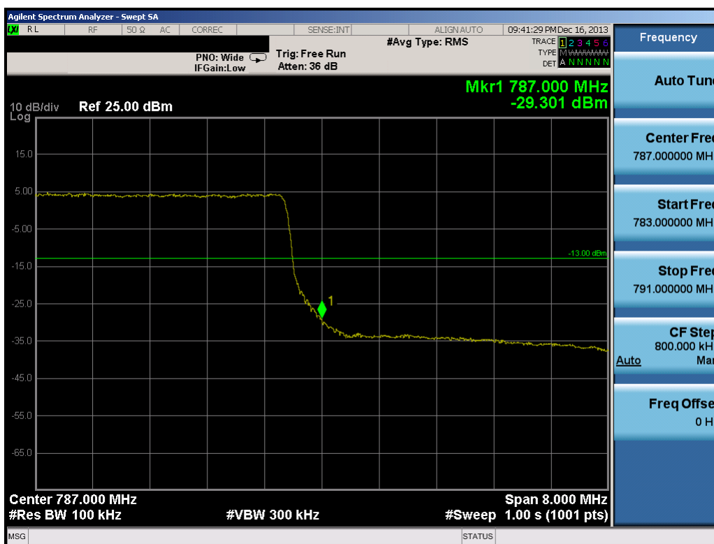
Plot 7-7. Upper Band Edge Plot (10.0MHz QPSK – RB Size 50)
