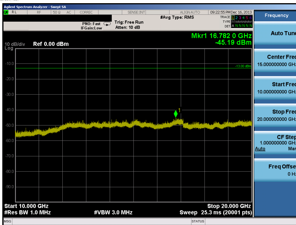
Plot 8-48. Conducted Spurious Plot (20.0MHz QPSK – RB Size 1, RB Offset 0 – Low Channel)
