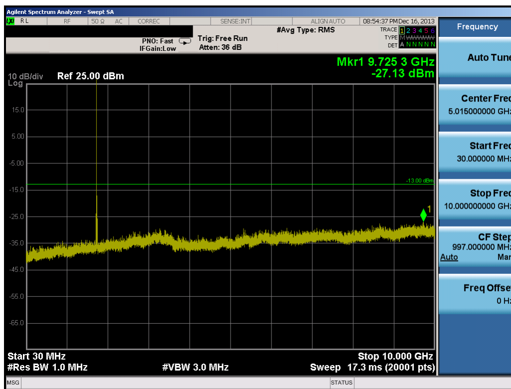
Plot 8-23. Conducted Spurious Plot (10.0MHz QPSK – RB Size 1, RB Offset 0 – High Channel)
