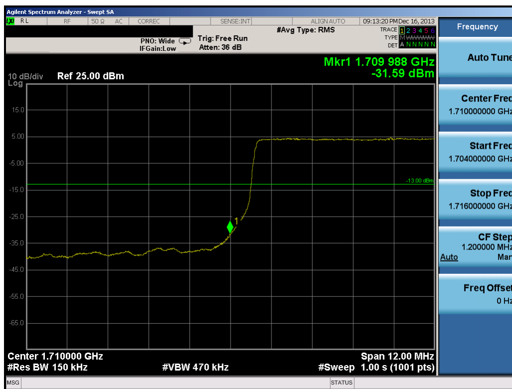
Plot 8-29. Lower Band Edge Plot (15.0MHz QPSK – RB Size 75)
