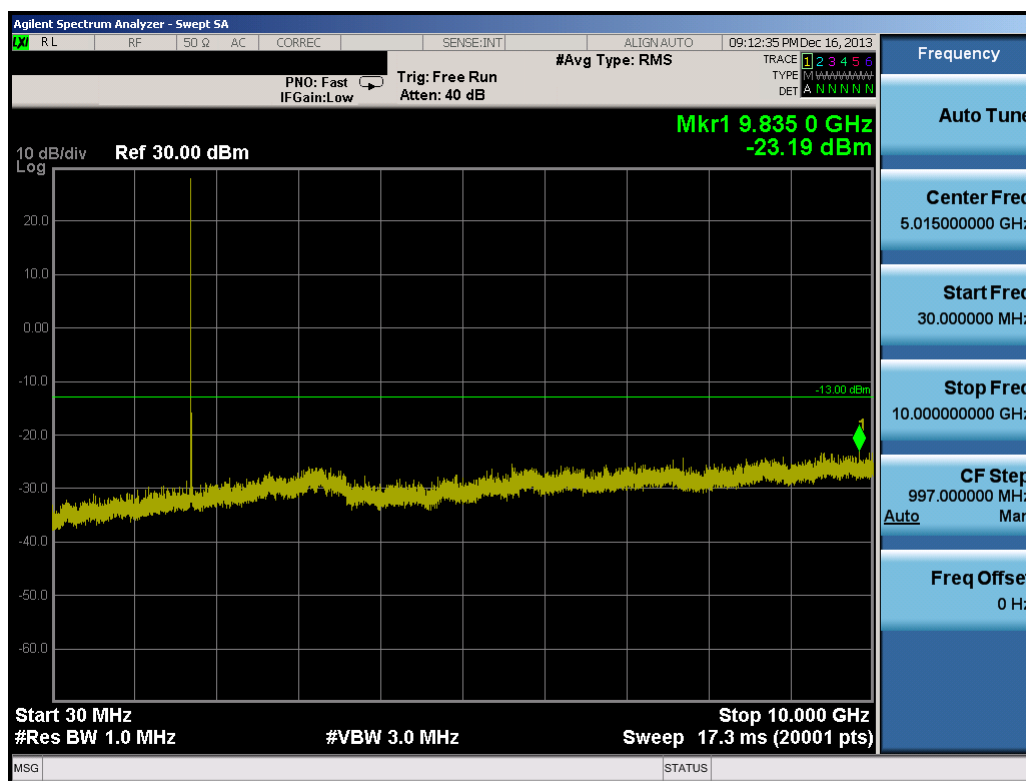
Plot 8-33. Conducted Spurious Plot (15.0MHz QPSK – RB Size 1, RB Offset 0 – Low Channel)
