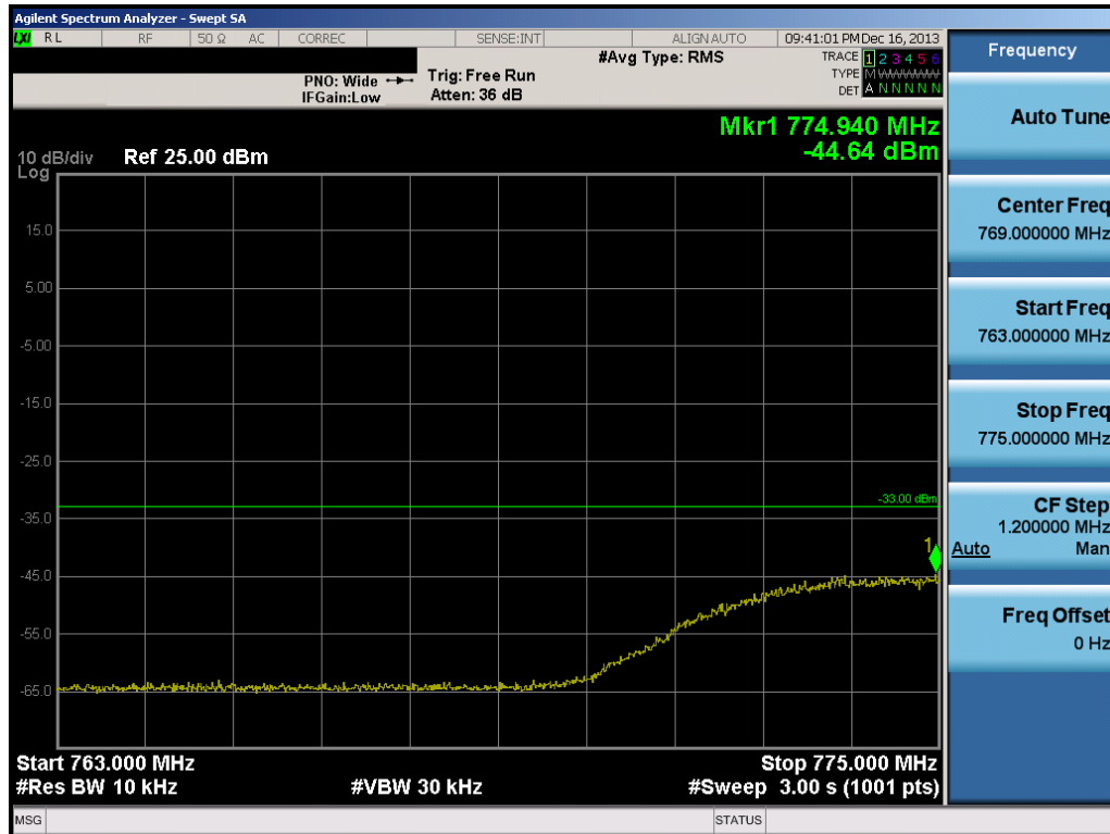
Plot 7-2. Lower Emission Mask Plot (10.0MHz QPSK – RB Size 50)
