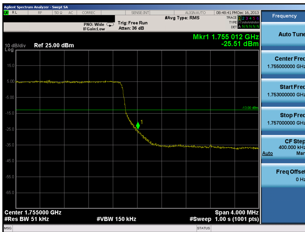
Plot 8-11. Upper Band Edge Plot (5.0MHz QPSK – RB Size 25)
