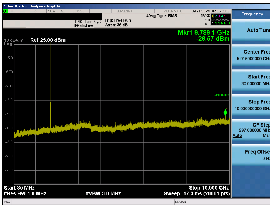
Plot 8-47. Conducted Spurious Plot (20.0MHz QPSK – RB Size 1, RB Offset 0– Low Channel)
