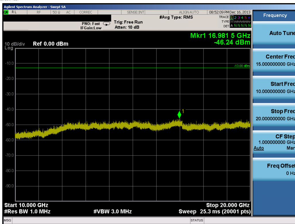
Plot 8-20. Conducted Spurious Plot (10.0MHz QPSK – RB Size 1, RB Offset 0 – Low Channel)
