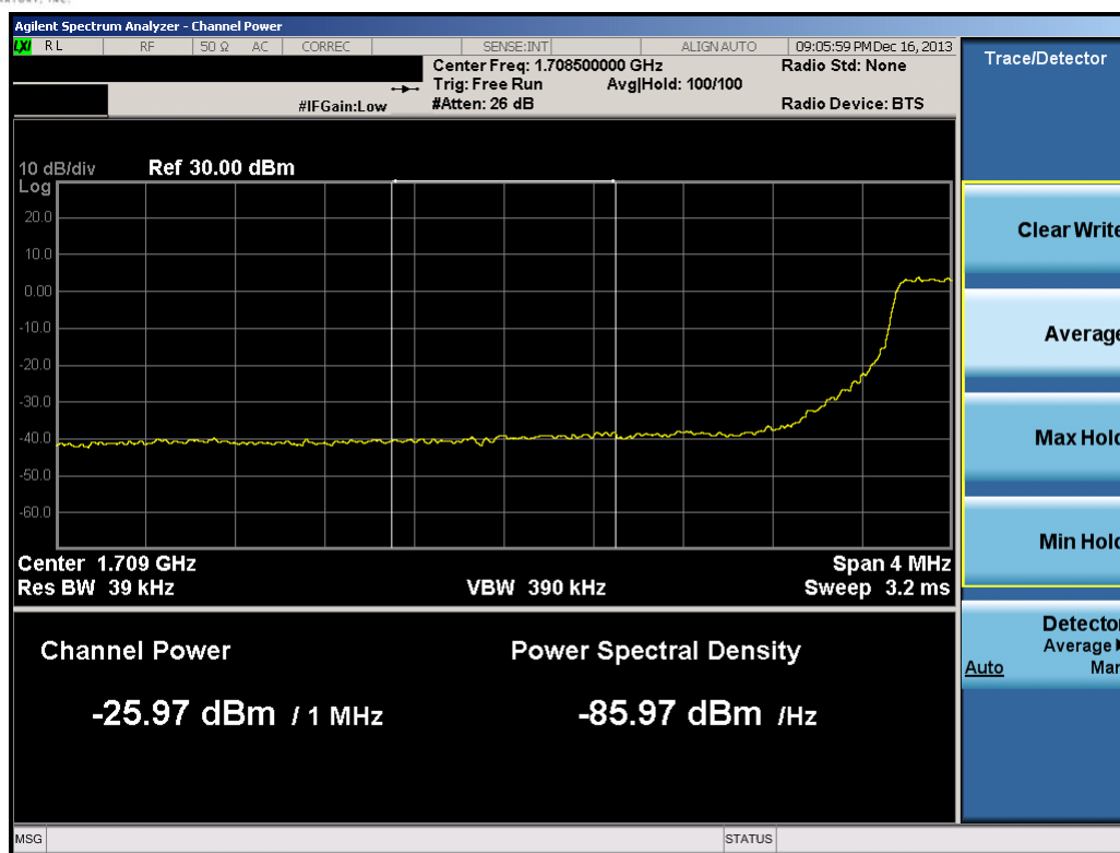
Plot 8-2. Lower Extended Band Edge Plot (5.0MHz QPSK – RB Size 25)
