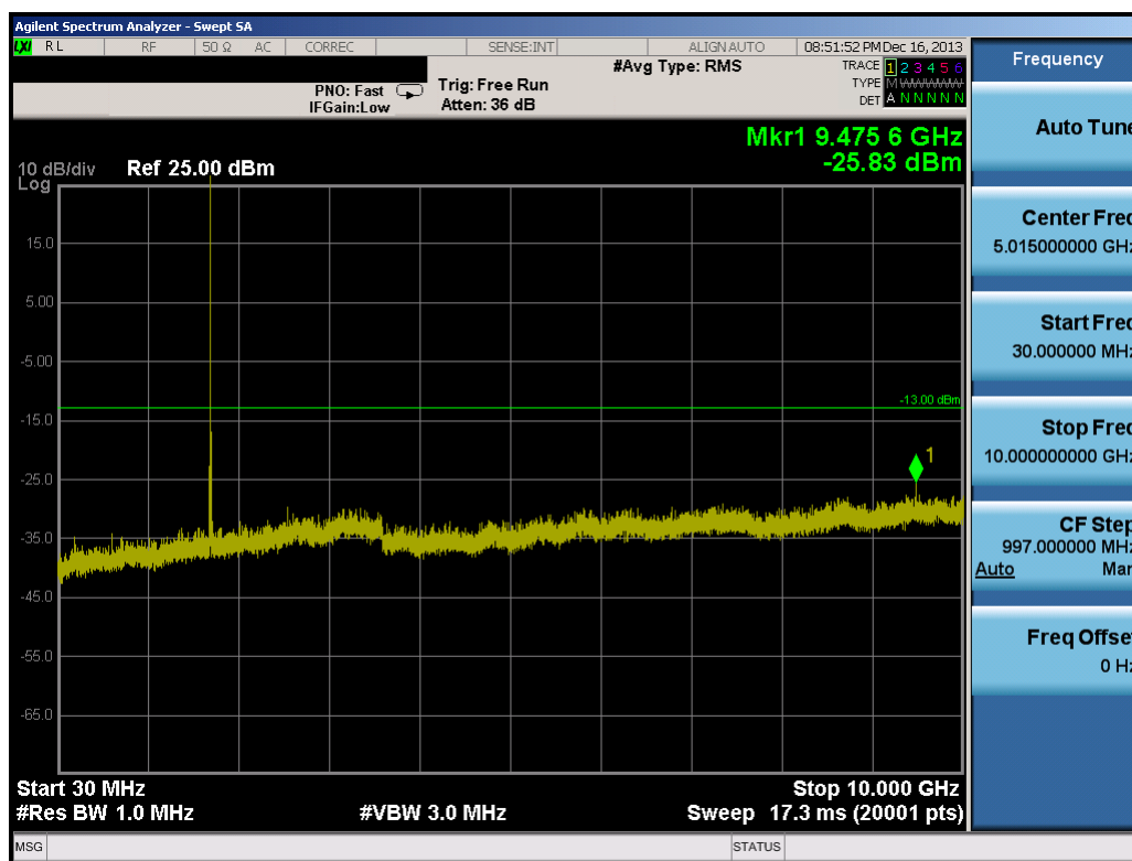
Plot 8-19. Conducted Spurious Plot (10.0MHz QPSK – RB Size 1, RB Offset 0– Low Channel)
