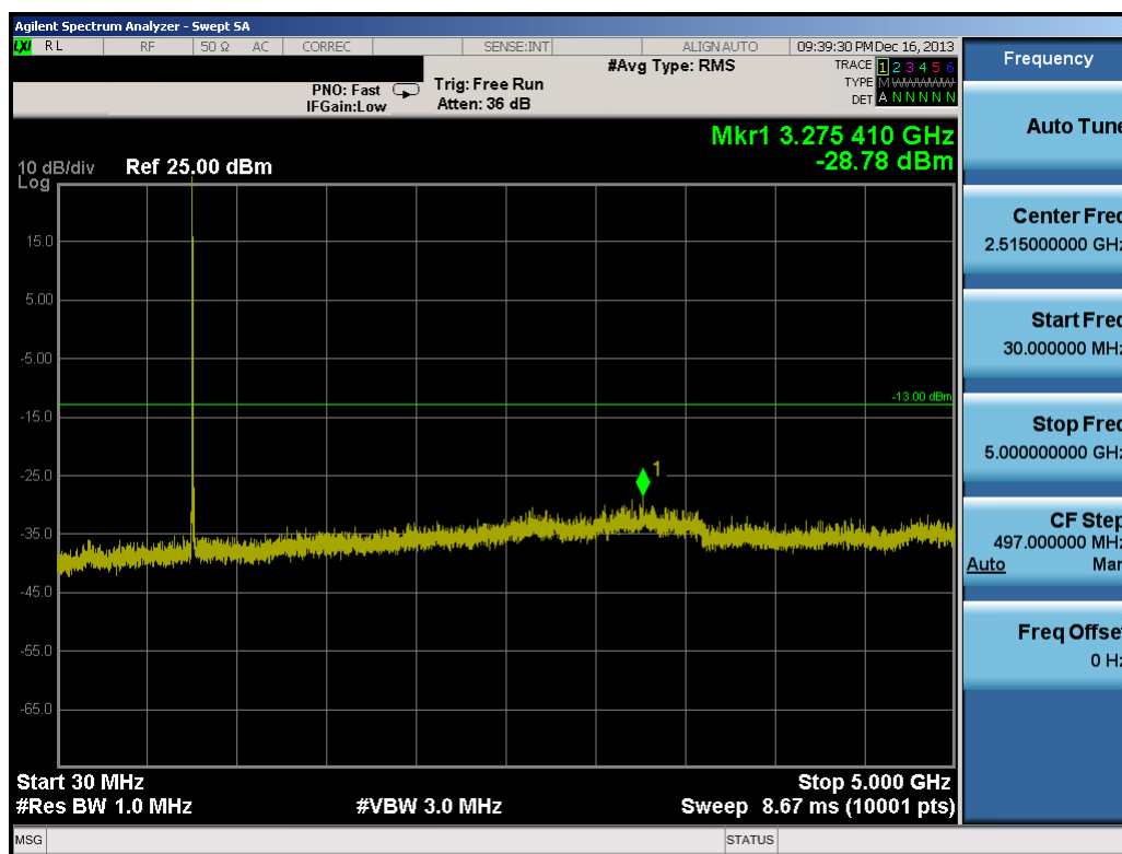
Plot 7-5. Conducted Spurious Plot (10.0MHz QPSK – RB Size 1, RB Offset 0)
