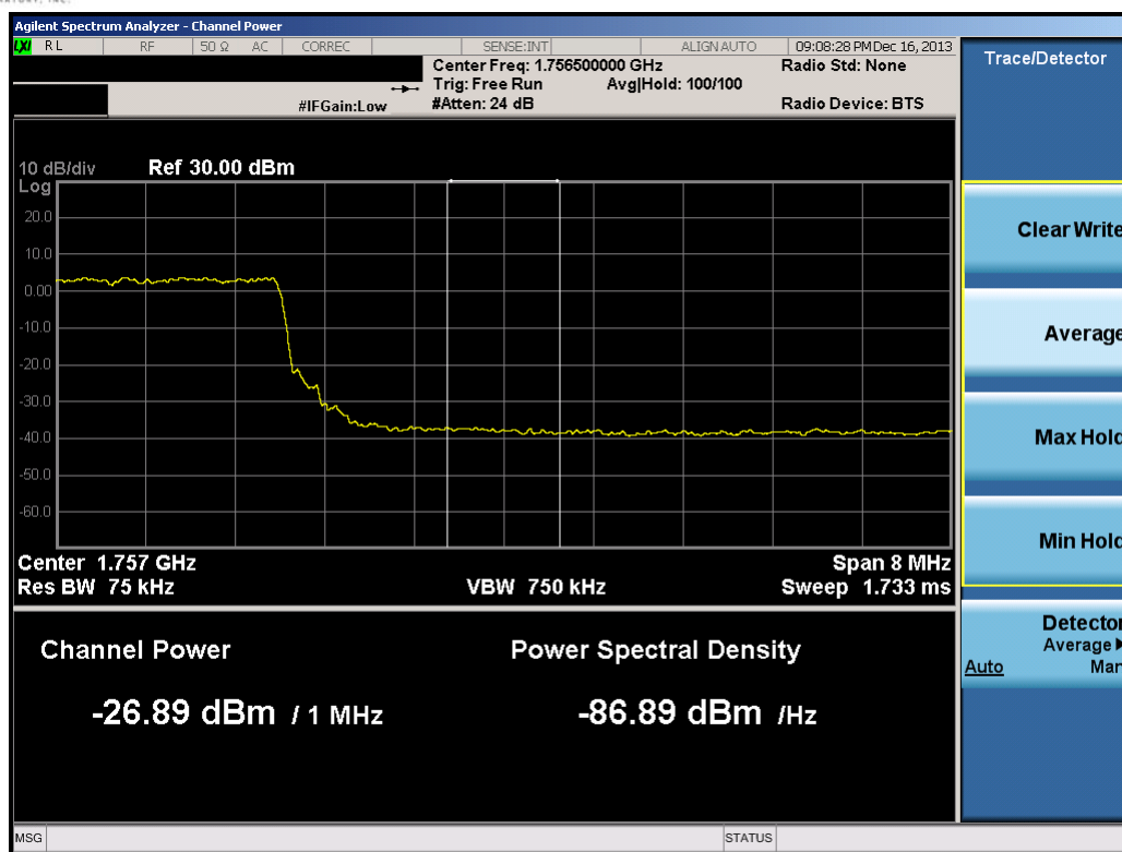
Plot 8-26. Upper Extended Band Edge Plot (10.0MHz QPSK – RB Size 50)
