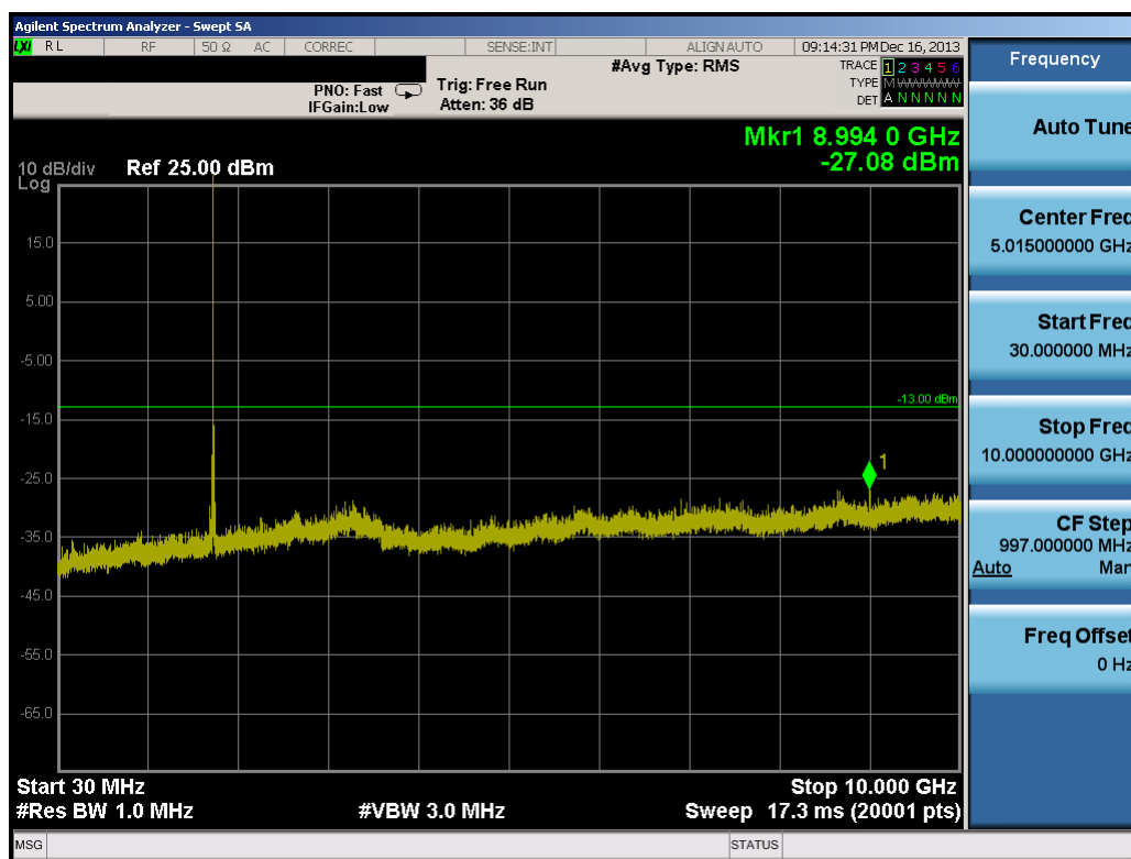
Plot 8-37. Conducted Spurious Plot (15.0MHz QPSK – RB Size 1, RB Offset 0 – High Channel)
