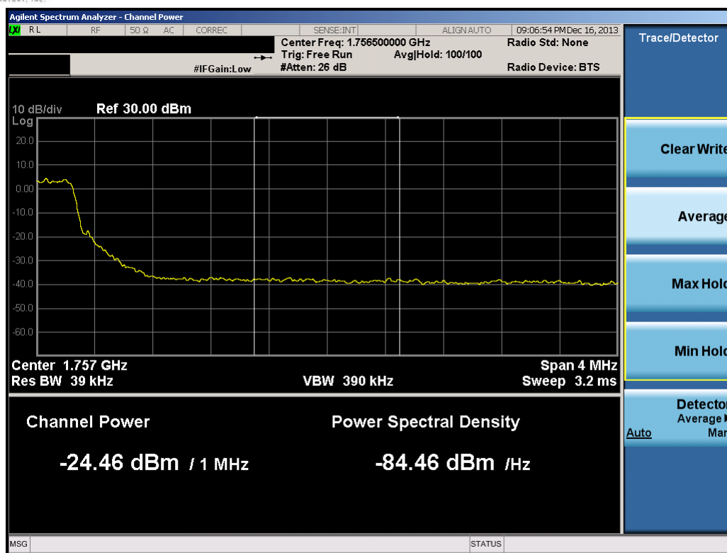
Plot 8-12. Upper Extended Band Edge Plot (5.0MHz QPSK – RB Size 25)
