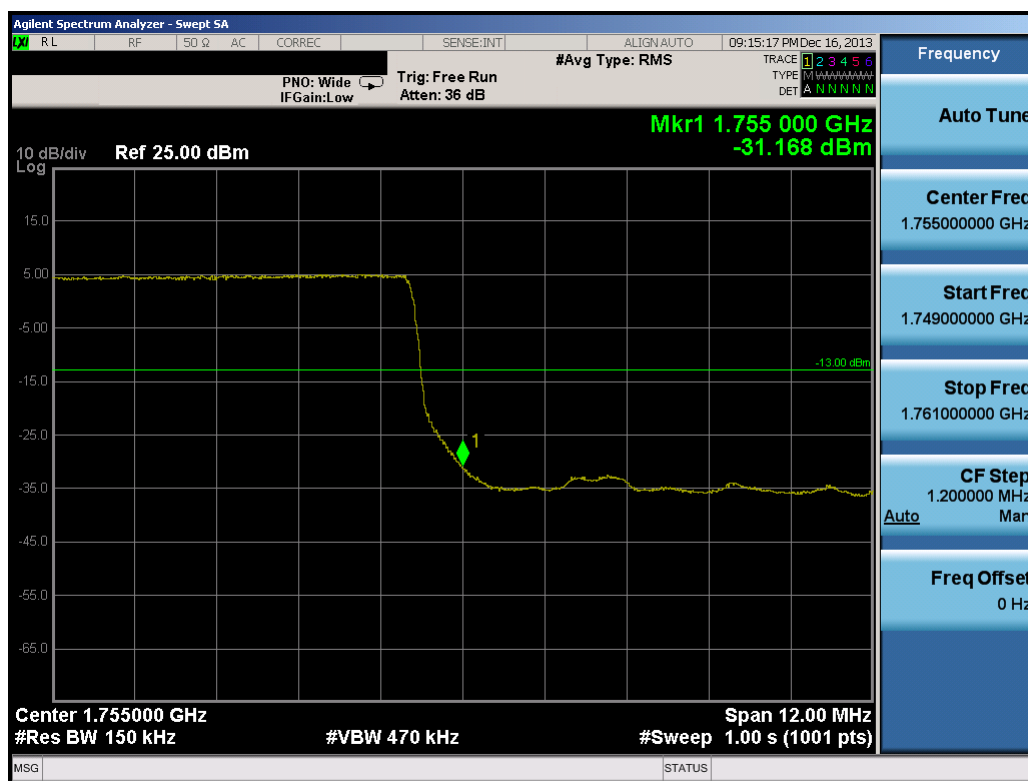
Plot 8-39. Upper Band Edge Plot (15.0MHz QPSK – RB Size 75)
