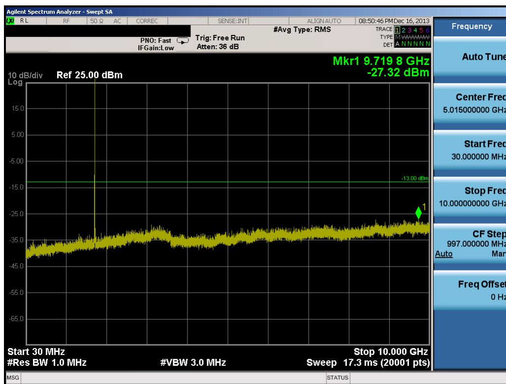
Plot 8-21. Conducted Spurious Plot (10.0MHz QPSK – RB Size 1, RB Offset 0 – Mid Channel)
