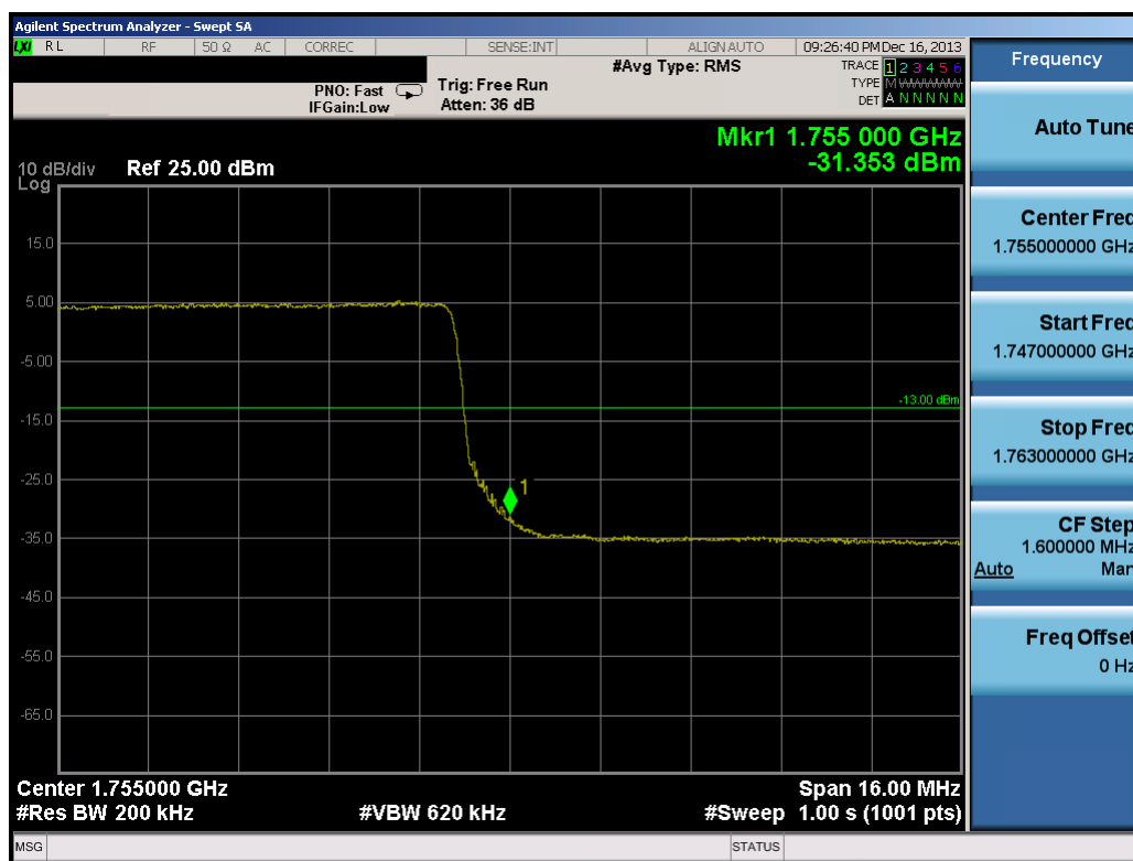
Plot 8-53. Upper Band Edge Plot (20.0MHz QPSK – RB Size 100)
