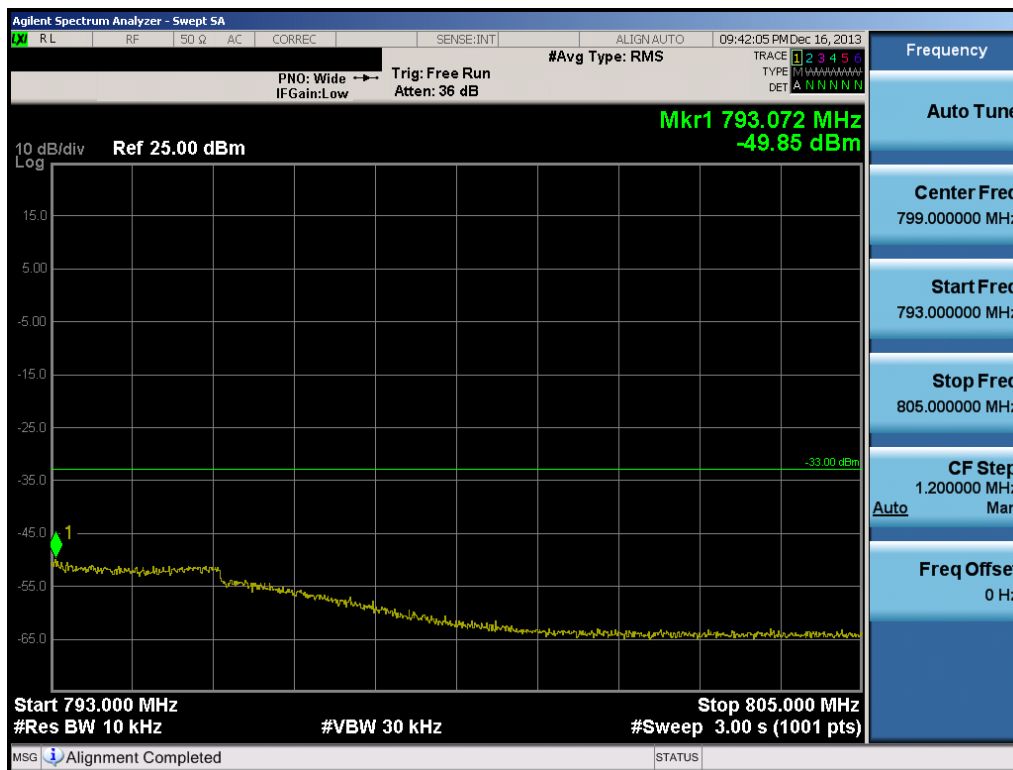
Plot 7-8. Upper Emission Mask Plot (10.0MHz QPSK – RB Size 50)
