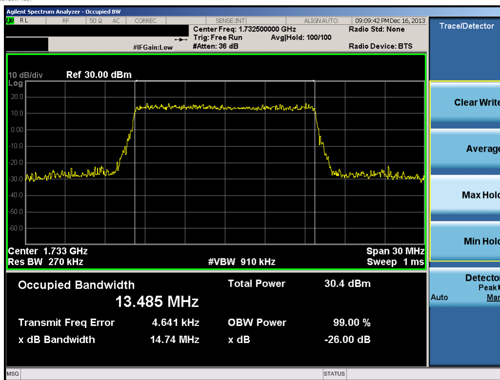
Plot 8-32. Occupied Bandwidth Plot (15.0MHz 16-QAM – RB Size 75)
