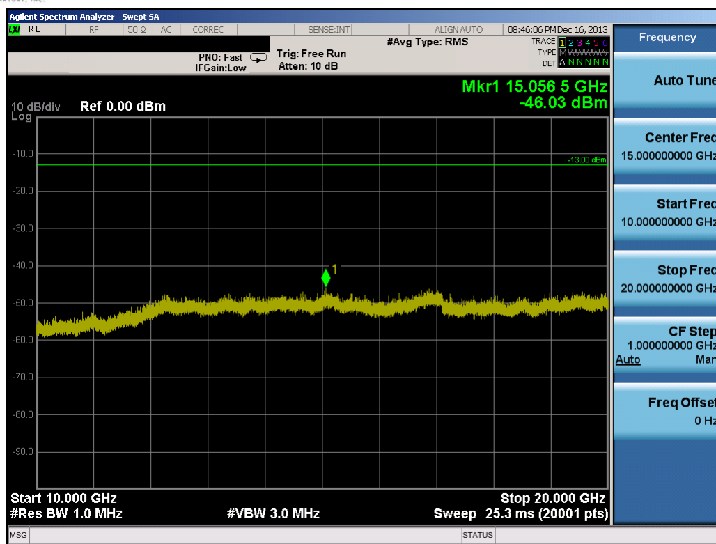
Plot 8-6. Conducted Spurious Plot (5.0MHz QPSK – RB Size 1, RB Offset 0 – Low Channel)
