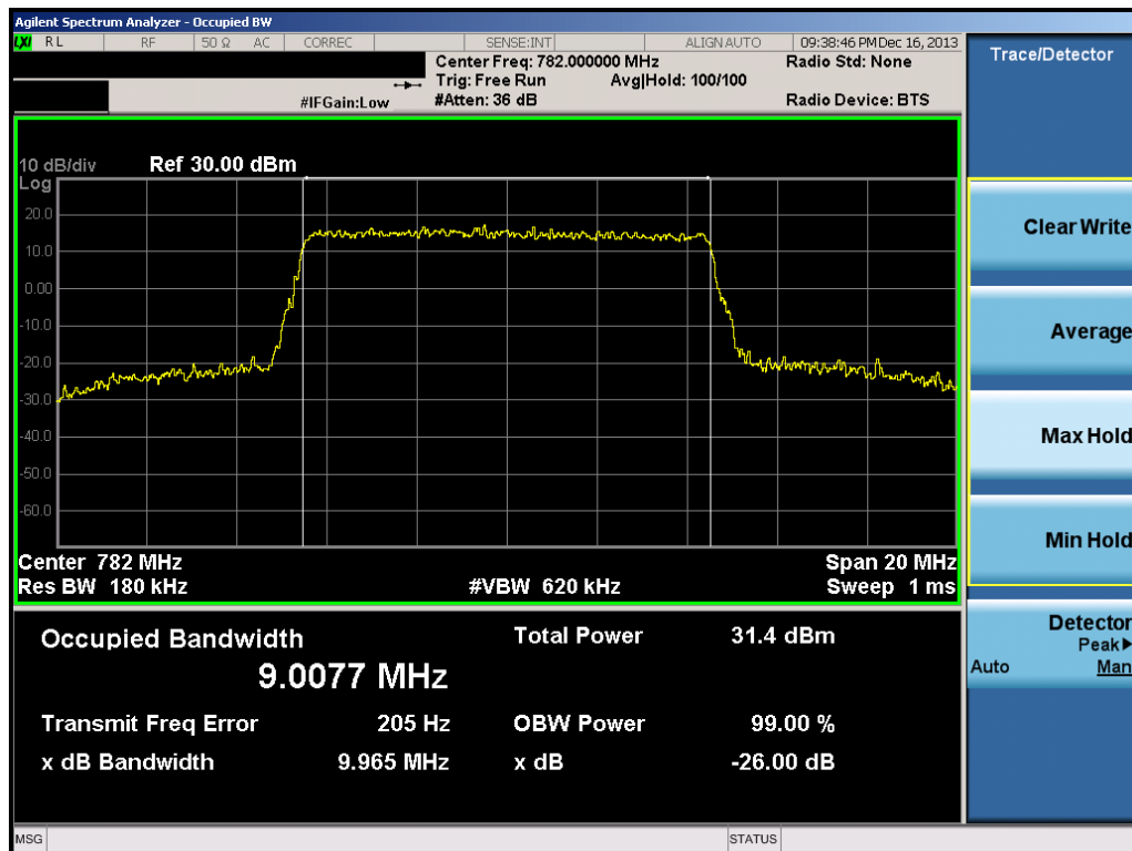
Plot 7-3. Occupied Bandwidth Plot (10.0MHz QPSK – RB Size 50)
