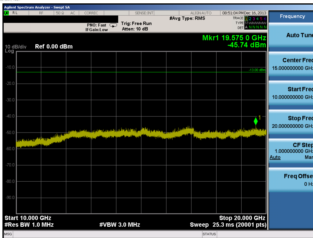
Plot 8-22. Conducted Spurious Plot (10.0MHz QPSK – RB Size 1, RB Offset 0 – Mid Channel)
