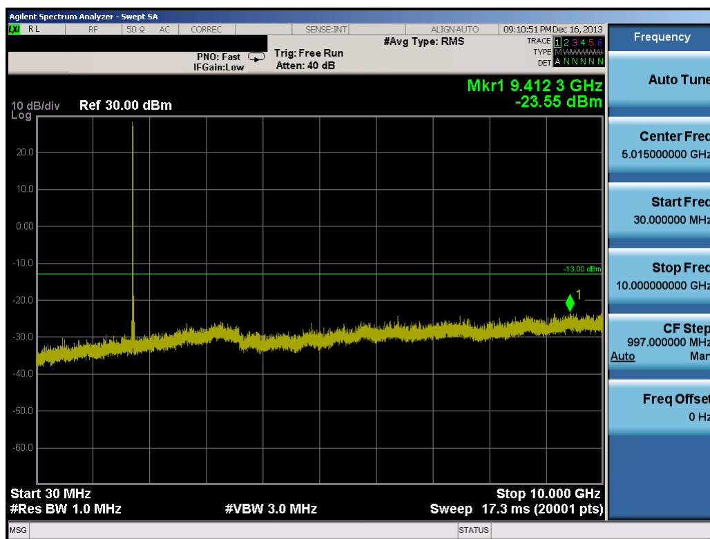
Plot 8-35. Conducted Spurious Plot (15.0MHz QPSK – RB Size 1, RB Offset 0 – Mid Channel)
