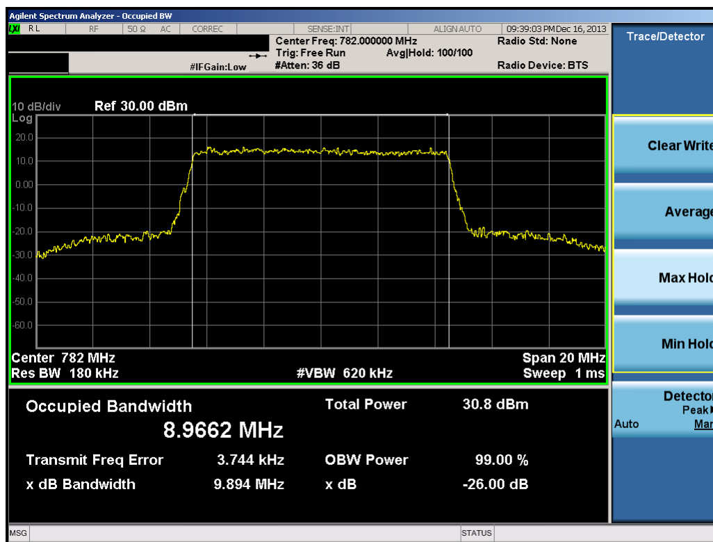
Plot 7-4. Occupied Bandwidth Plot (10.0MHz 16-QAM – RB Size 50)
