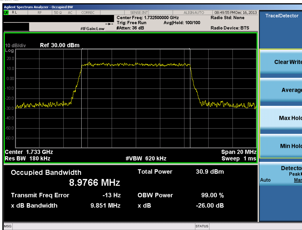
Plot 8-18. Occupied Bandwidth Plot (10.0MHz 16-QAM – RB Size 50)
