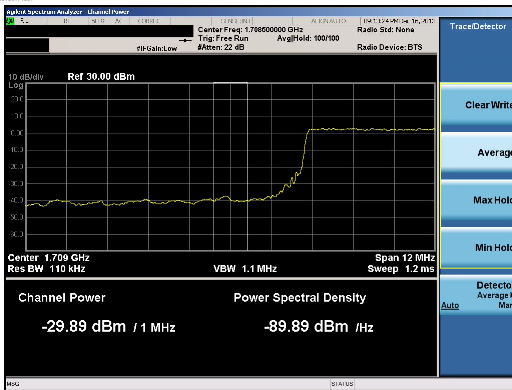
Plot 8-30. Lower Extended Band Edge Plot (15.0MHz QPSK – RB Size 75)
