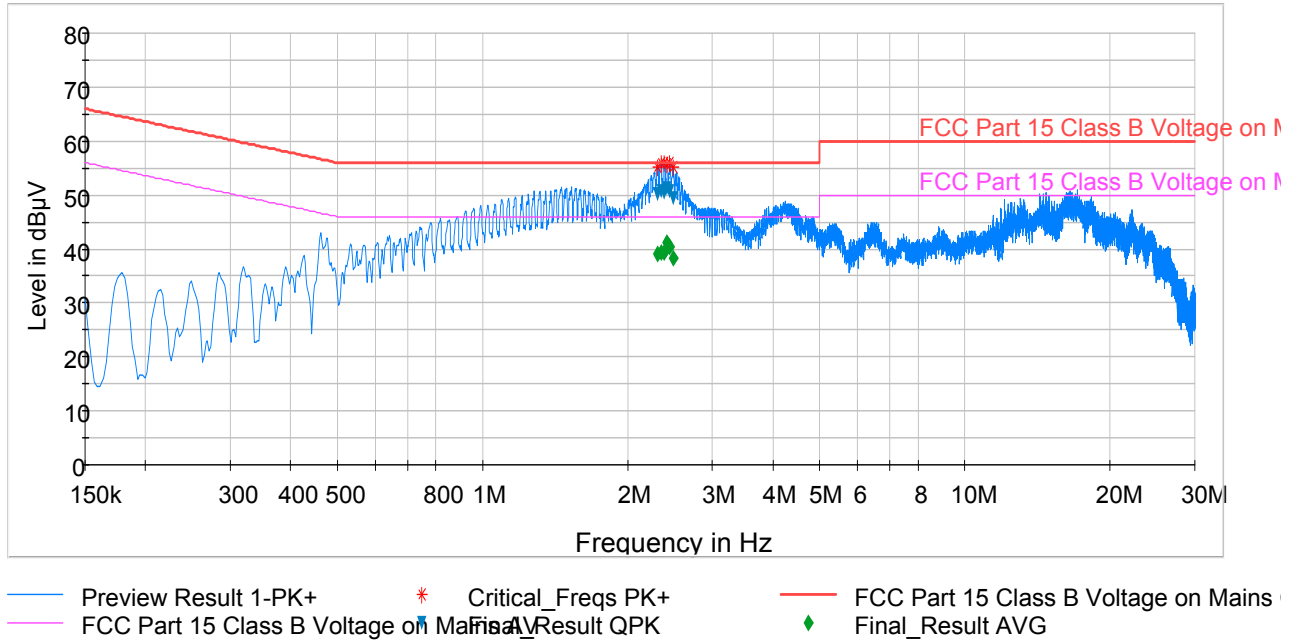
Plot 6-55. Line-Conducted Test Plot (N)
