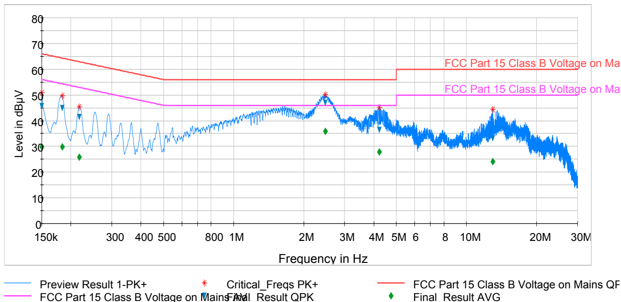
Plot 6-54. Line-Conducted Test Plot (L1)
