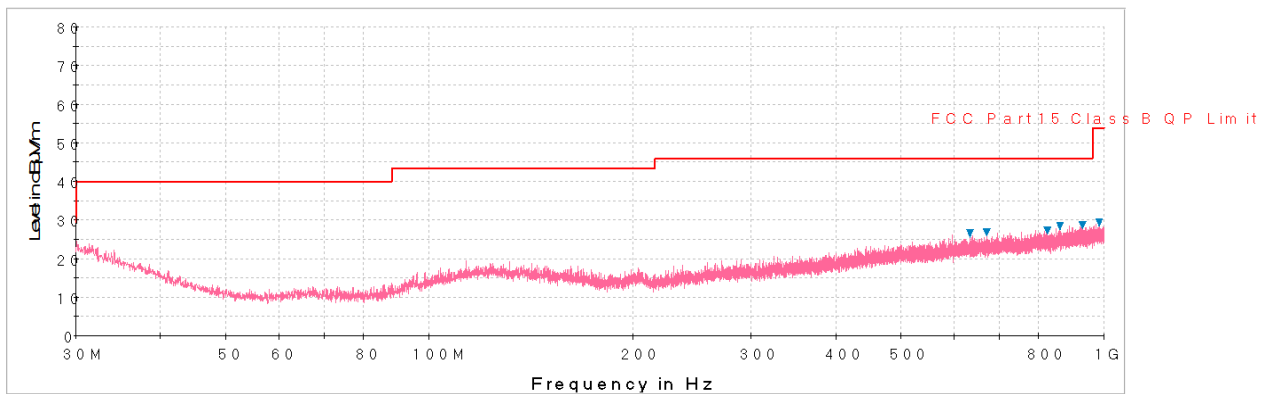
Plot 6-10. Radiated Spurious Plot below 1GHz (Pol. V)
