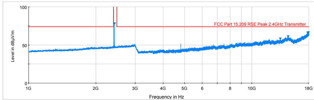
Plot 6-1. Radiated Spurious Plot above 1GHz (BT – Ch. 0, Ant. Pol. H)
