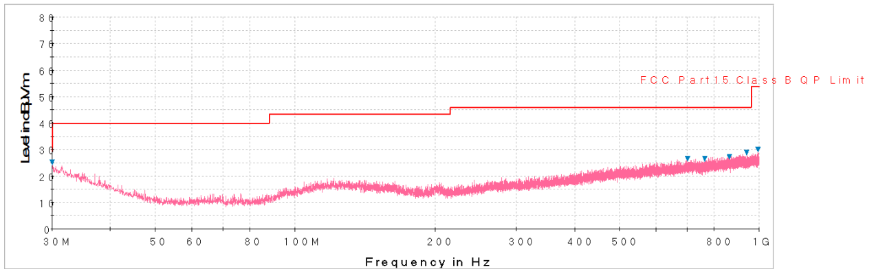
Plot 6-9. Radiated Spurious Plot below 1GHz (Pol. H)
