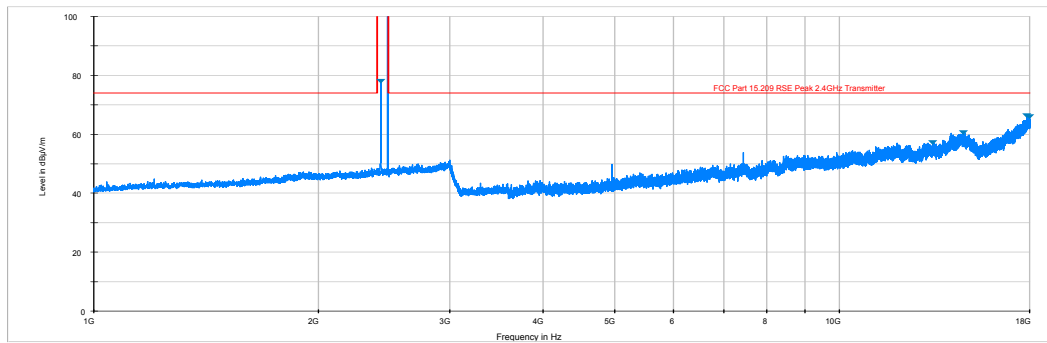
Plot 6-5. Radiated Spurious Plot above 1GHz (BT – Ch. 78, Ant. Pol. H)
