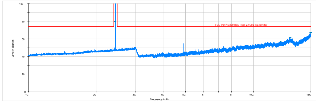
Plot 6-4. Radiated Spurious Plot above 1GHz (BT – Ch. 39, Ant. Pol. V)
