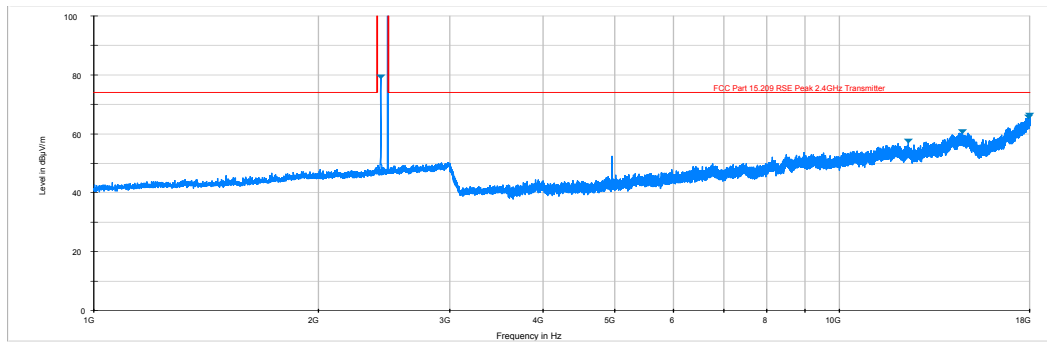
Plot 6-6. Radiated Spurious Plot above 1GHz (BT – Ch. 78, Ant. Pol. V)
