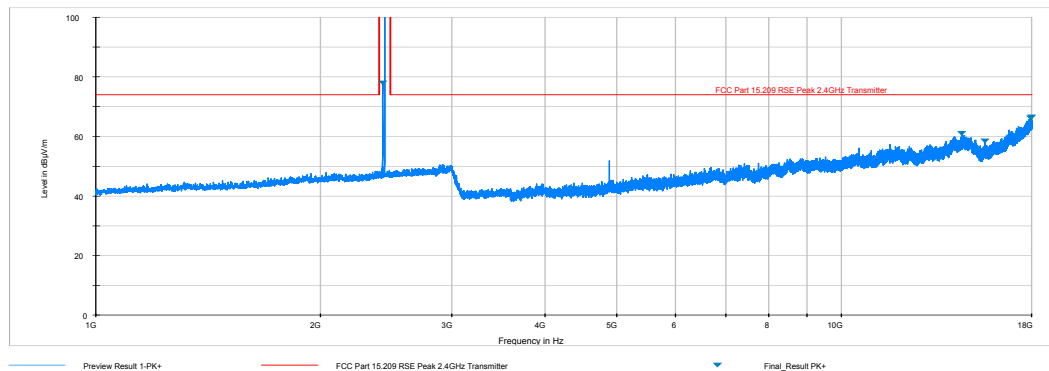
Plot 6-3. Radiated Spurious Plot above 1GHz (BT – Ch. 39, Ant. Pol. H)
