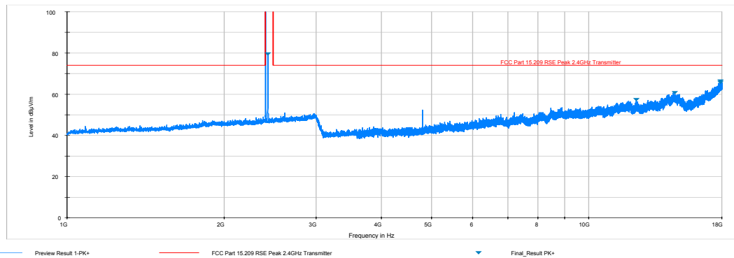
Plot 6-2. Radiated Spurious Plot above 1GHz (BT – Ch. 0, Ant. Pol. V)
