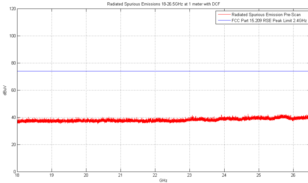
Plot 6-7. Radiated Spurious Plot above 18GHz (Pol. H)
