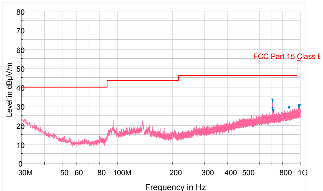
Plot 6-93. Radiated Spurious Plot below 1GHz (802.11a – U3 Ch. 157, Ant. Pol. H)
