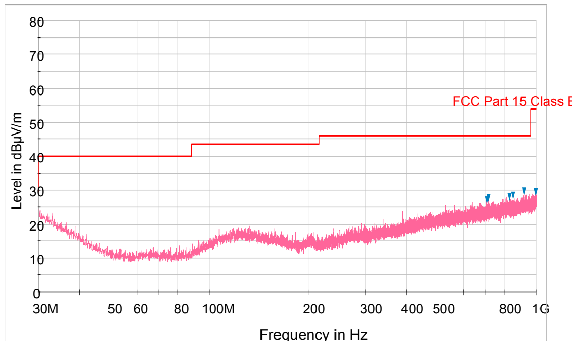
Plot 6-94. Radiated Spurious Plot below 1GHz (802.11a – U3 Ch. 157, Ant. Pol. V)
