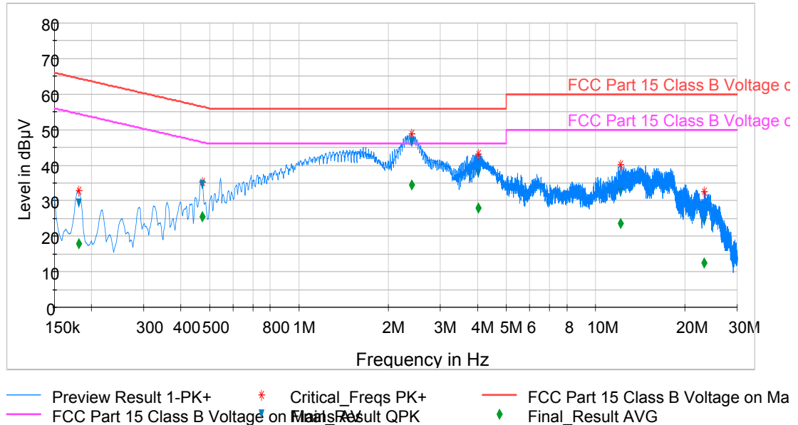
Plot 6-45. Line Conducted Plot with 802.11b (L1)
