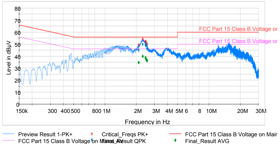
Plot 6-46. Line Conducted Plot with 802.11b (N)
