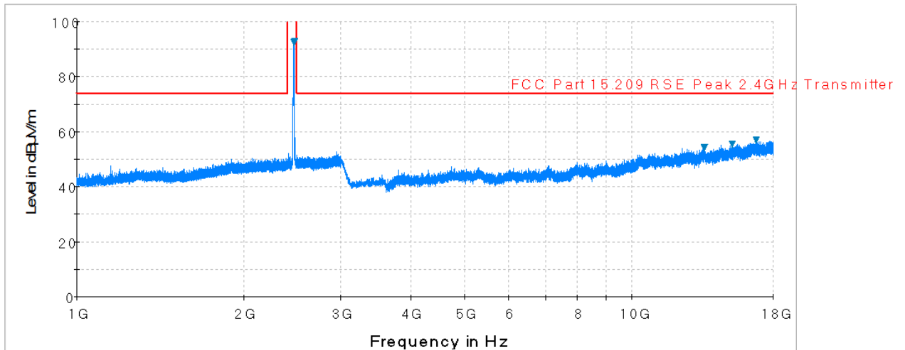
Plot 6-6. Radiated Spurious Plot above 1GHz (802.11b – Ch. 11, Ant. Pol. V)
