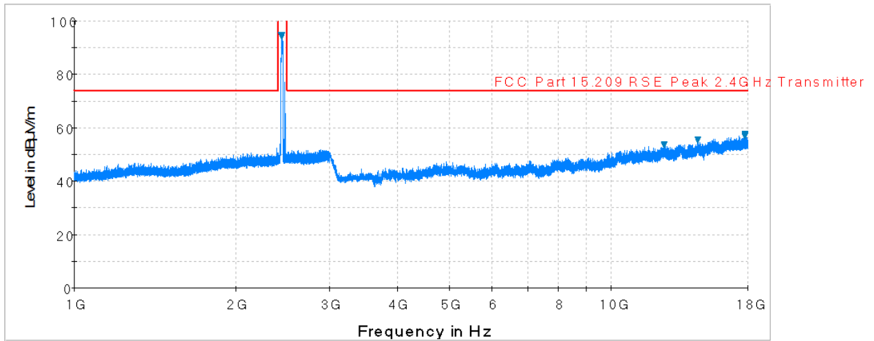
Plot 6-4. Radiated Spurious Plot above 1GHz (802.11b – Ch. 6, Ant. Pol. V)
