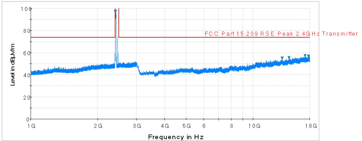
Plot 6-1. Radiated Spurious Plot above 1GHz (802.11b – Ch. 1, Ant. Pol. H)
