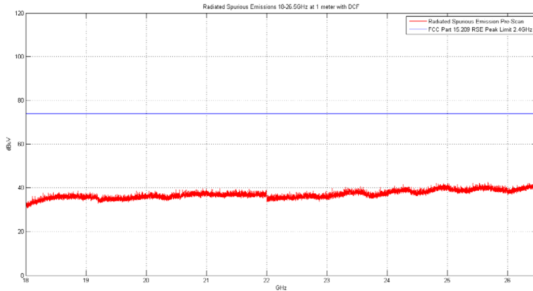
Plot 6-7. Radiated Spurious Plot above 18GHz (Pol. H)
