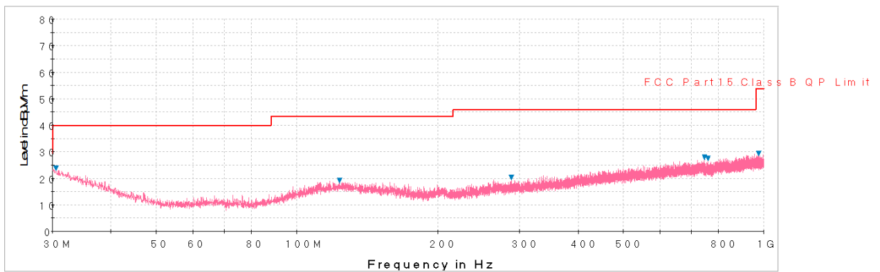
Plot 6-14. Radiated Spurious Plot below 1GHz (Pol. V)
