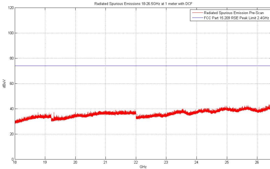
Plot 6-8. Radiated Spurious Plot above 18GHz (Pol. V)
