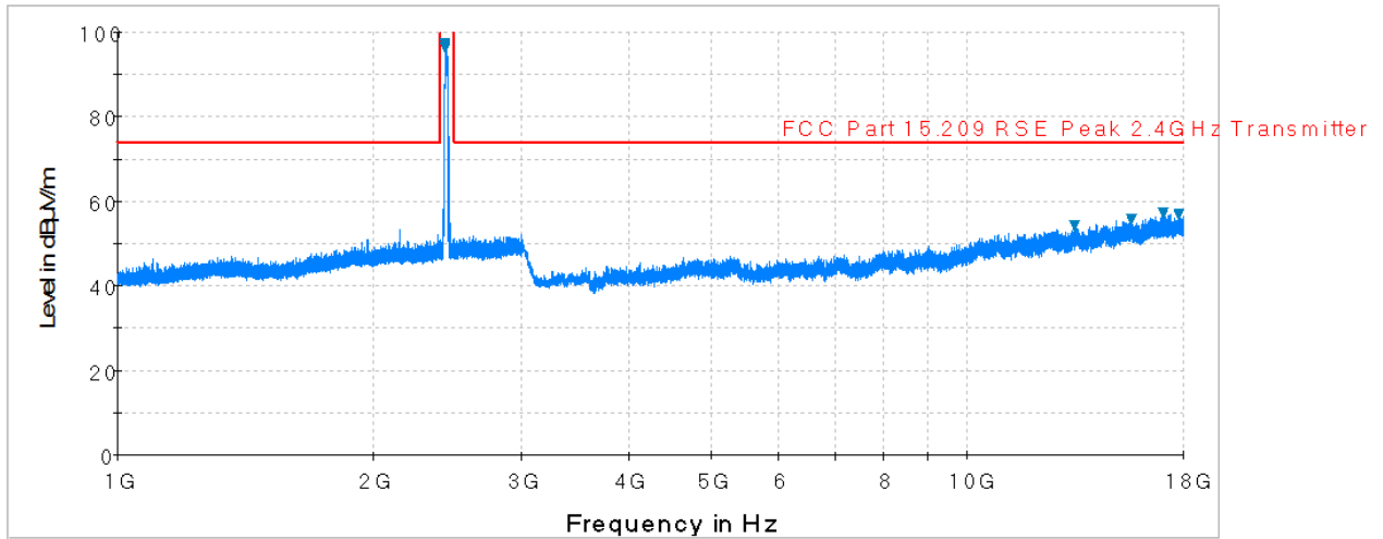
Plot 6-3. Radiated Spurious Plot above 1GHz (802.11b – Ch. 6, Ant. Pol. H)
