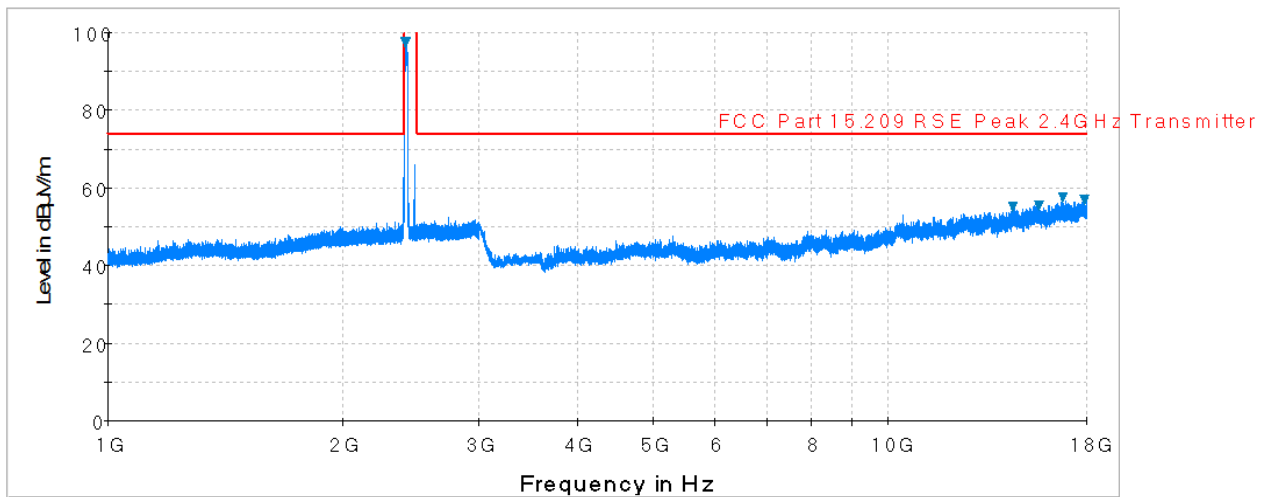
Plot 6-2. Radiated Spurious Plot above 1GHz (802.11b – Ch. 1, Ant. Pol. V)
