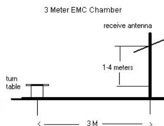
Figure 6-1. Test Instrument & Measurement Setup
