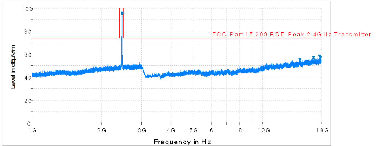
Plot 6-5. Radiated Spurious Plot above 1GHz (802.11b – Ch. 11, Ant. Pol. H)
