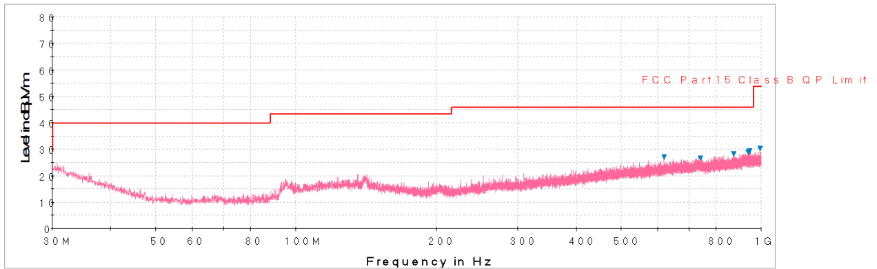
Plot 6-13. Radiated Spurious Plot below 1GHz (Pol. H)
