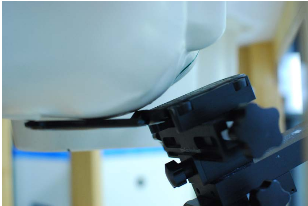
SAR Test Setup Photo 3 - Right Cheek
