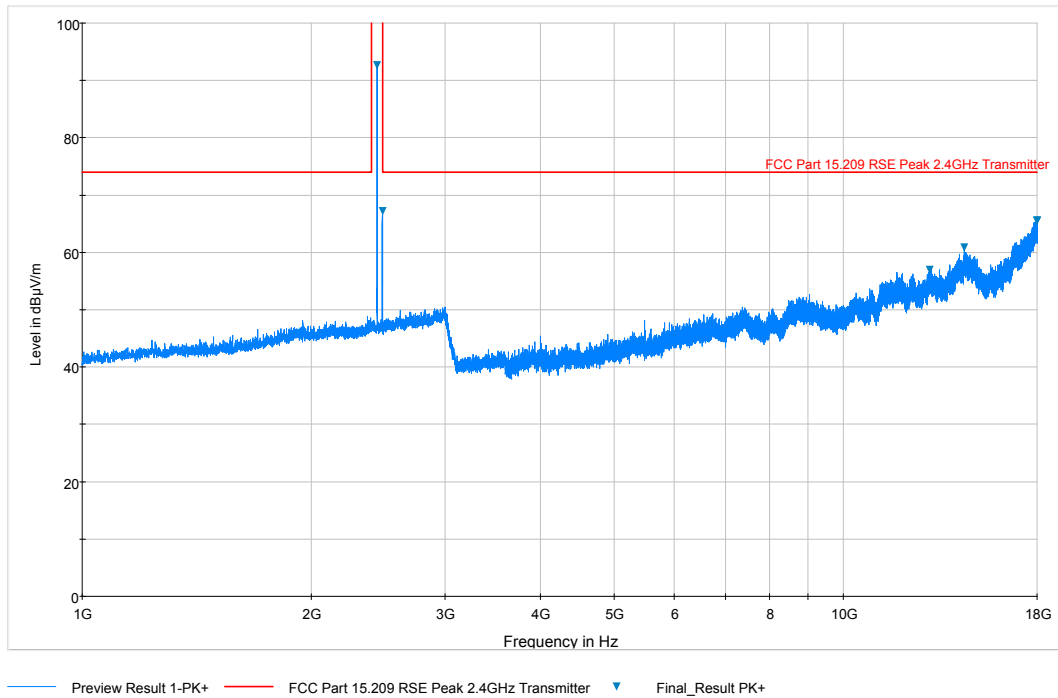
Plot 6-45. Radiated Spurious Plot above 1GHz (BT – Ch. 39, Ant. Pol. V)
