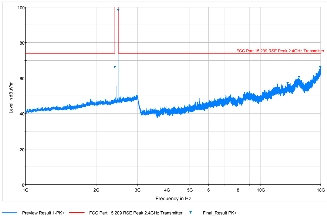
Plot 6-47. Radiated Spurious Plot above 1GHz (BT – Ch. 78, Ant. Pol. V)
