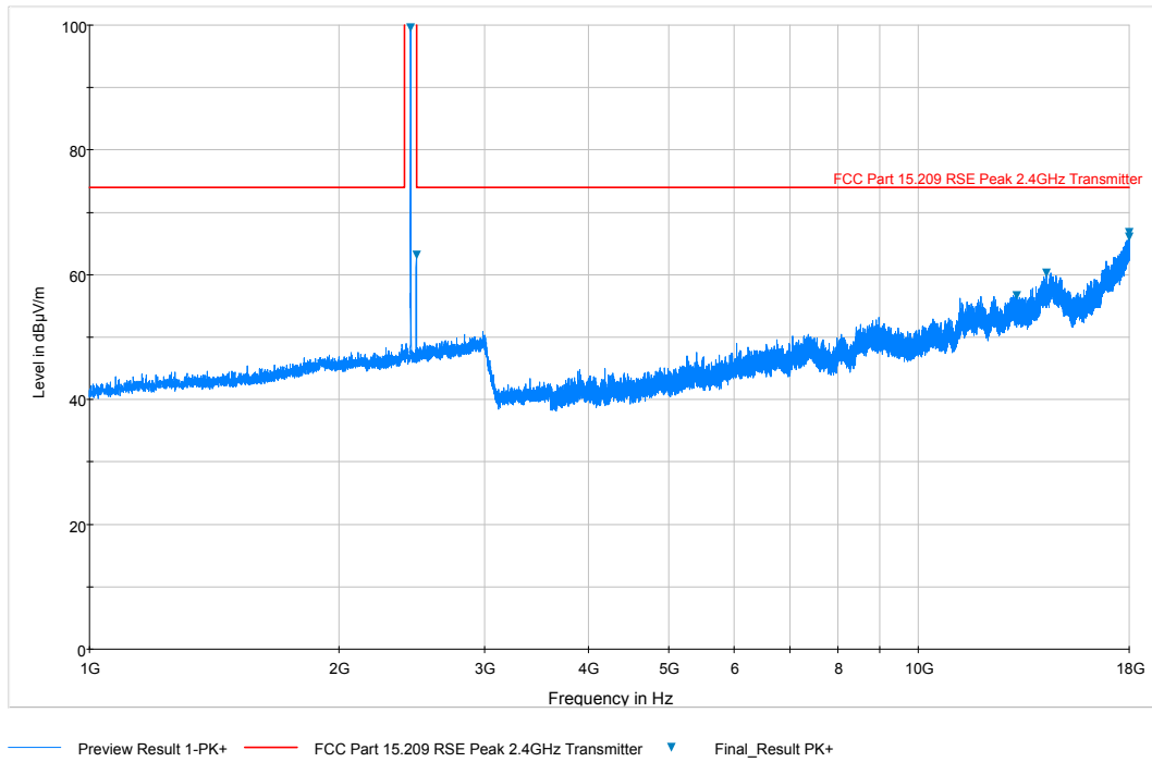
Plot 6-44. Radiated Spurious Plot above 1GHz (BT – Ch. 39, Ant. Pol. H)
