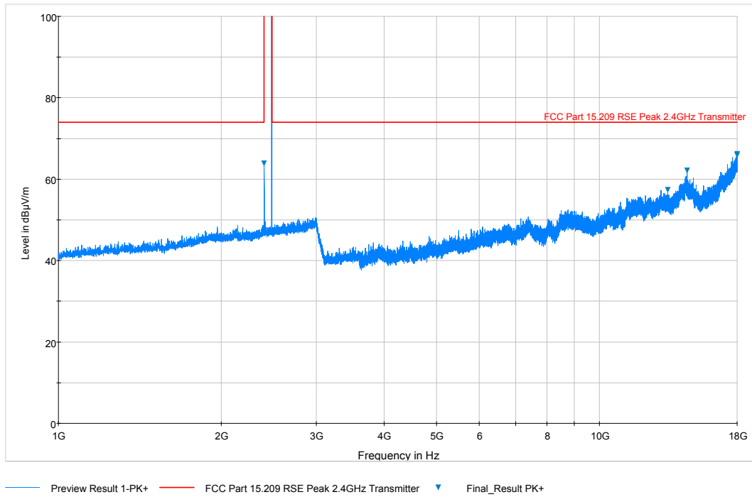
Plot 6-46. Radiated Spurious Plot above 1GHz (BT – Ch. 78, Ant. Pol. H)
