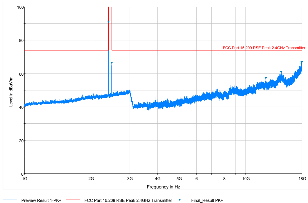
Plot 6-43. Radiated Spurious Plot above 1GHz (BT – Ch. 0, Ant. Pol. V)
