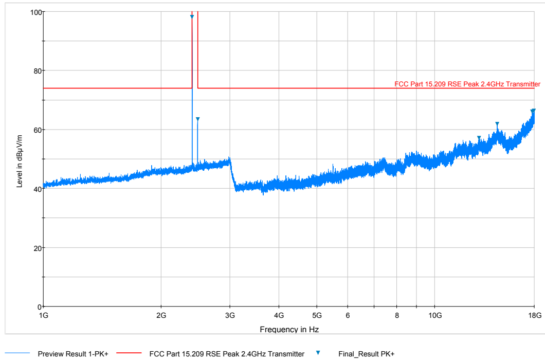
Plot 6-42. Radiated Spurious Plot above 1GHz (BT – Ch. 0, Ant. Pol. H)
