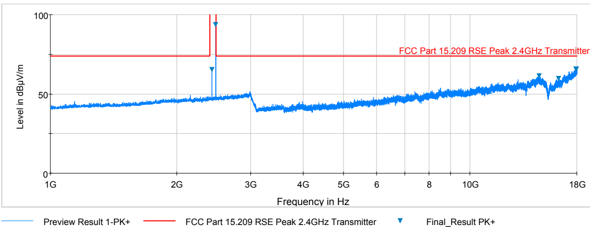
Plot 6-6. Radiated Spurious Plot above 1GHz (BT – Ch. 78, Ant. Pol. V)
