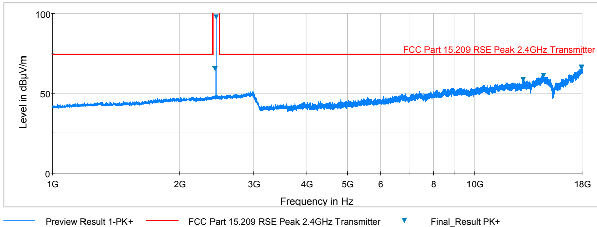
Plot 6-4. Radiated Spurious Plot above 1GHz (BT – Ch. 39, Ant. Pol. V)
