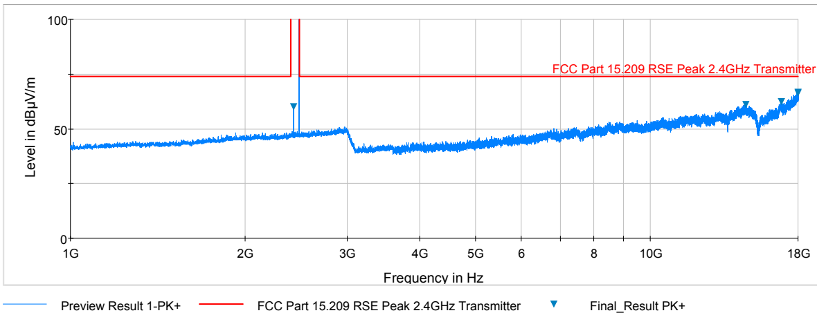
Plot 6-5. Radiated Spurious Plot above 1GHz (BT – Ch. 78, Ant. Pol. H)
