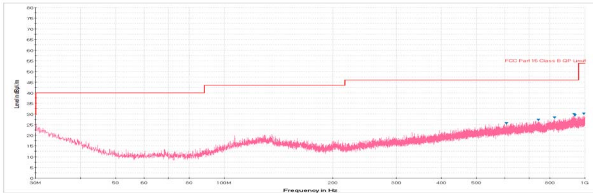
Plot 6-9. Radiated Spurious Plot below 1GHz (Pol. H)
