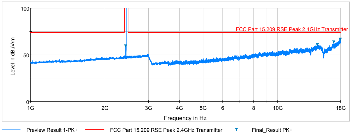
Plot 6-3. Radiated Spurious Plot above 1GHz (BT – Ch. 39, Ant. Pol. H)
