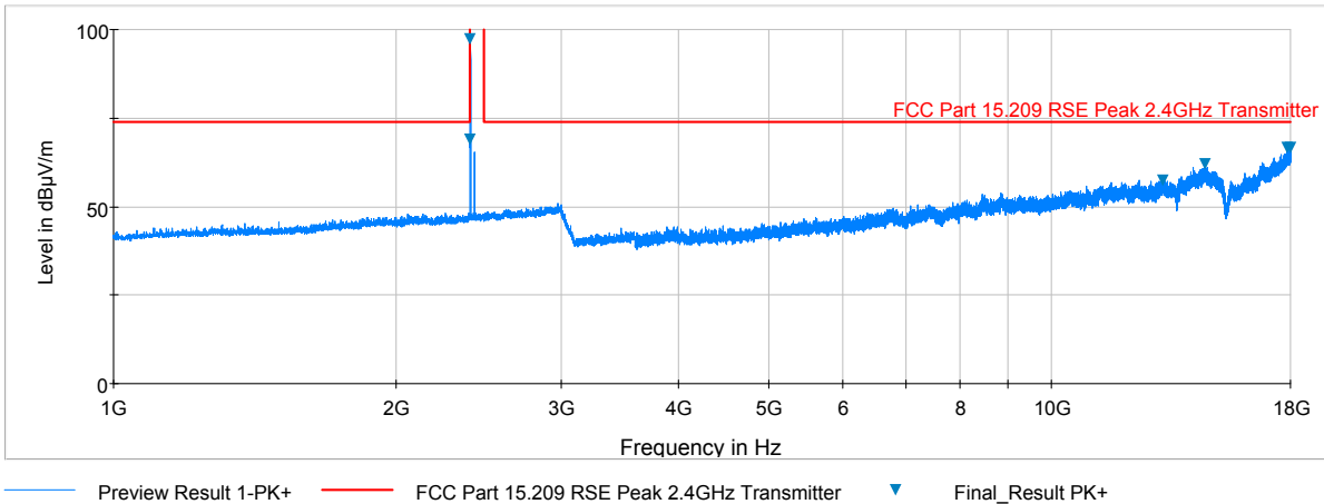
Plot 6-2. Radiated Spurious Plot above 1GHz (BT – Ch. 0, Ant. Pol. V)
