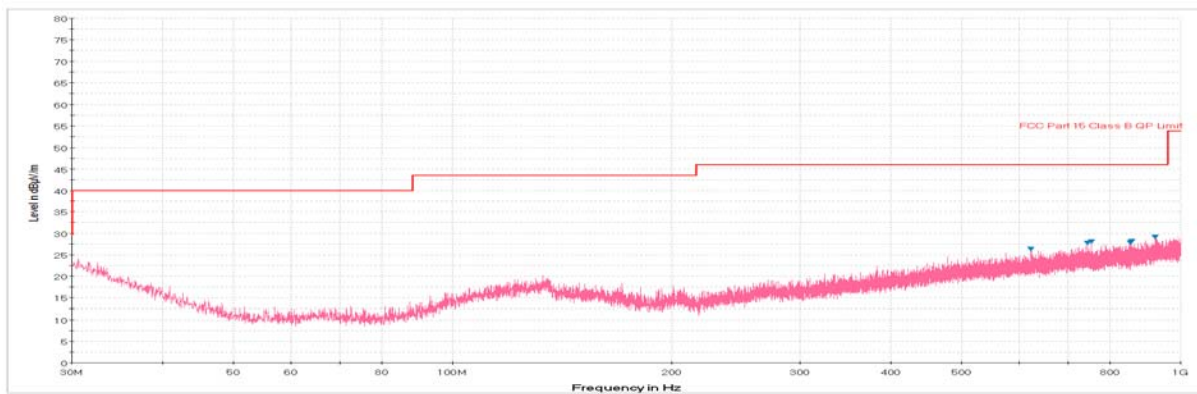
Plot 6-10. Radiated Spurious Plot below 1GHz (Pol. V)
