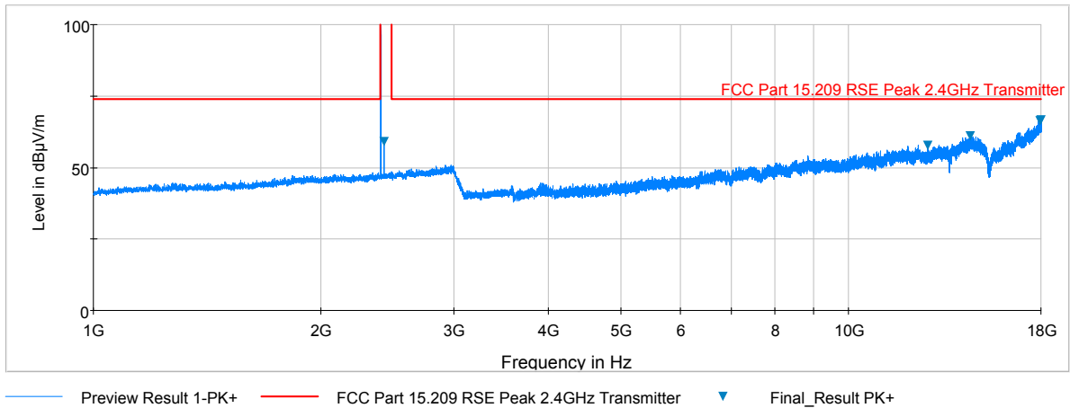
Plot 6-1. Radiated Spurious Plot above 1GHz (BT – Ch. 0, Ant. Pol. H)
