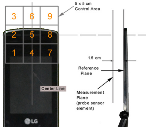
Figure 17-3 5x5 Scan grid above WD
