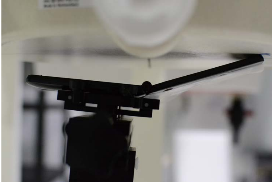
SAR Test Setup Photo 5 – Left Mouth-Jaw
