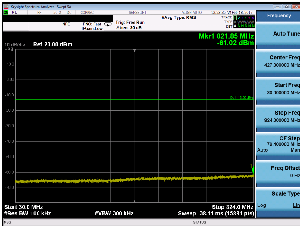
Plot 7-34. Conducted Spurious Plot (Band 5 – 10.0MHz QPSK – RB Size 1, RB Offset 0 – High Channel)
