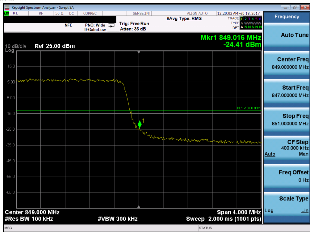
Plot 7-59. Upper Band Edge Plot (Band 5 – 5.0MHz QPSK – RB Size 25)
