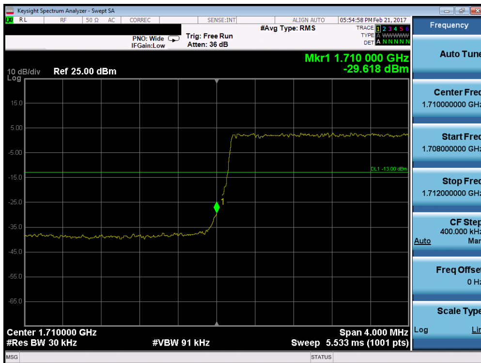
Plot 7-66. Lower Band Edge Plot (Band 4 – 3.0MHz QPSK – RB Size 15)
