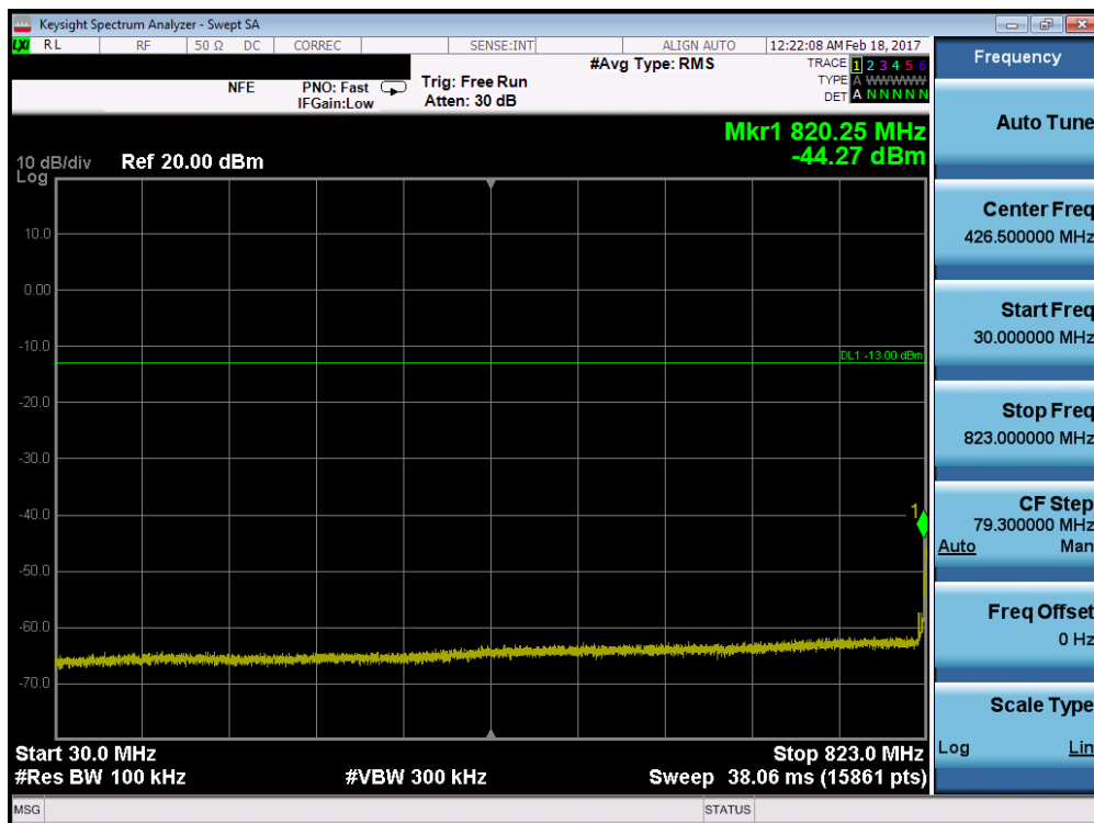
Plot 7-28. Conducted Spurious Plot (Band 5 – 10.0MHz QPSK – RB Size 1, RB Offset 0– Low Channel)
