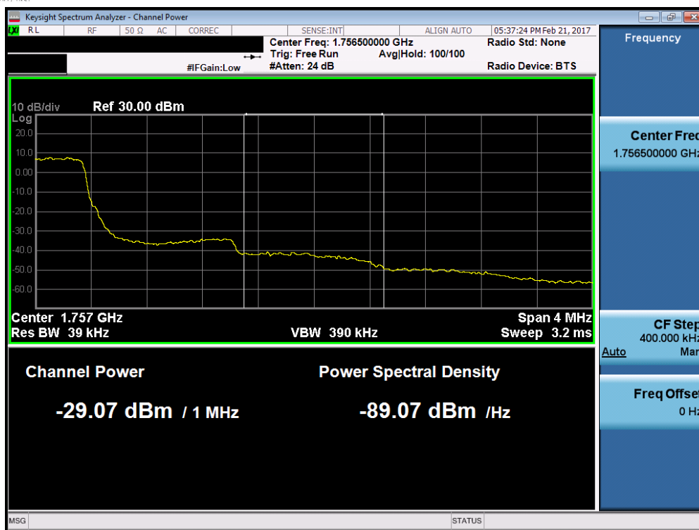
Plot 7-65. Upper Extended Band Edge Plot (Band 4 – 1.4MHz QPSK – RB Size 6)
