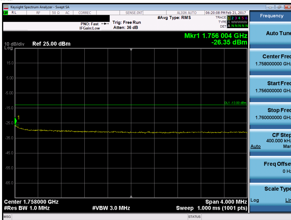
Plot 7-77. Upper Extended Band Edge Plot (Band 4 – 10.0MHz QPSK – RB Size 50)
