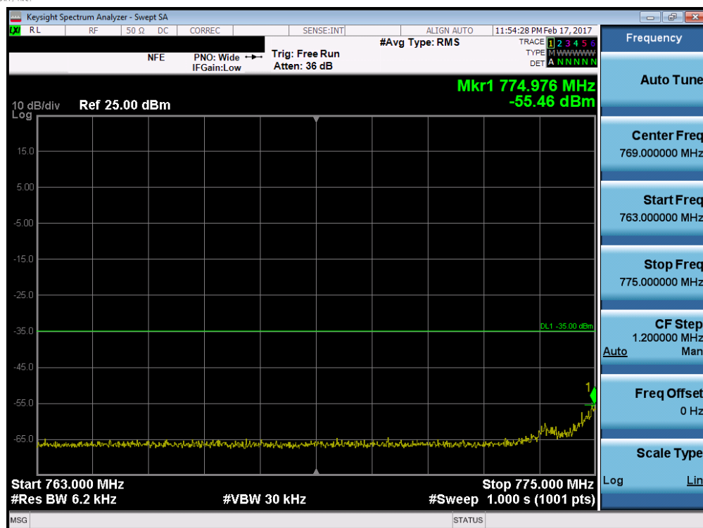
Plot 7-47. Lower Emission Mask Edge Plot (Band 13 - 5.0MHz QPSK - RB Size 25)
