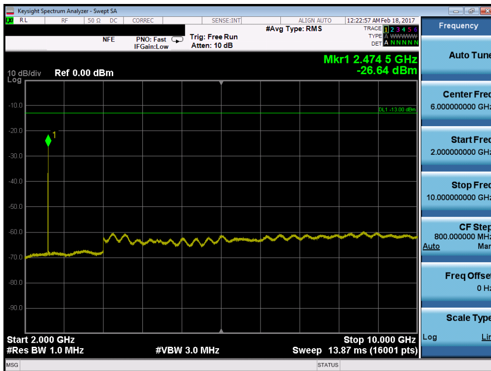
Plot 7-30. Conducted Spurious Plot (Band 5 – 10.0MHz QPSK – RB Size 1, RB Offset 0 – Low Channel)
