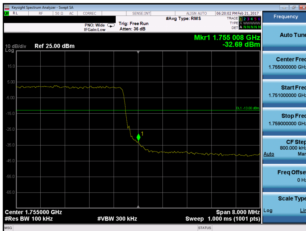
Plot 7-76. Upper Band Edge Plot (Band 4 - 10.0MHz QPSK - RB Size 50)
