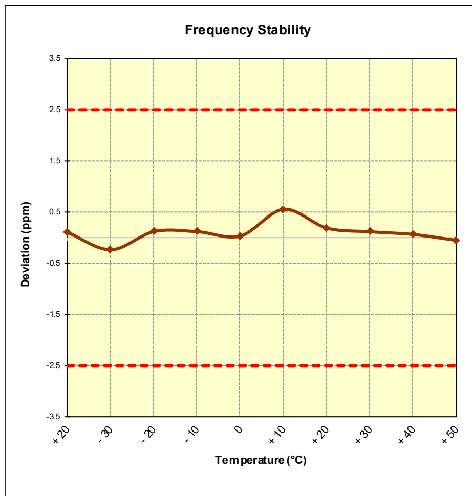
Figure 7-8. Frequency Stability Graph (Band 5)
