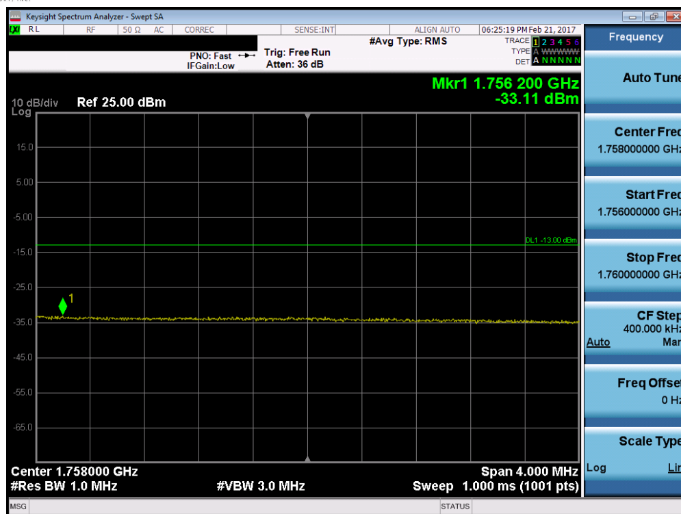
Plot 7-85. Upper Extended Band Edge Plot (Band 4 – 20.0MHz QPSK – RB Size 100)
