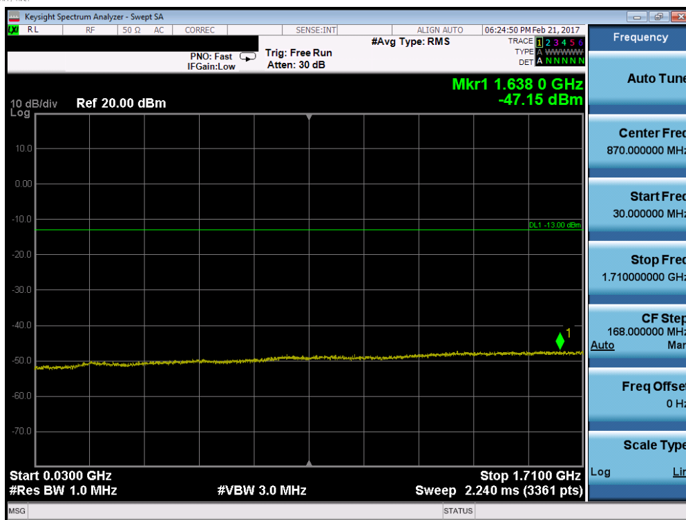
Plot 7-43. Conducted Spurious Plot (Band 4 – 20.0MHz QPSK – RB Size 1, RB Offset 0 – High Channel)
