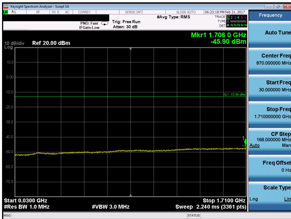
Plot 7-40. Conducted Spurious Plot (Band 4 – 20.0MHz QPSK – RB Size 1, RB Offset 0 – Mid Channel)
