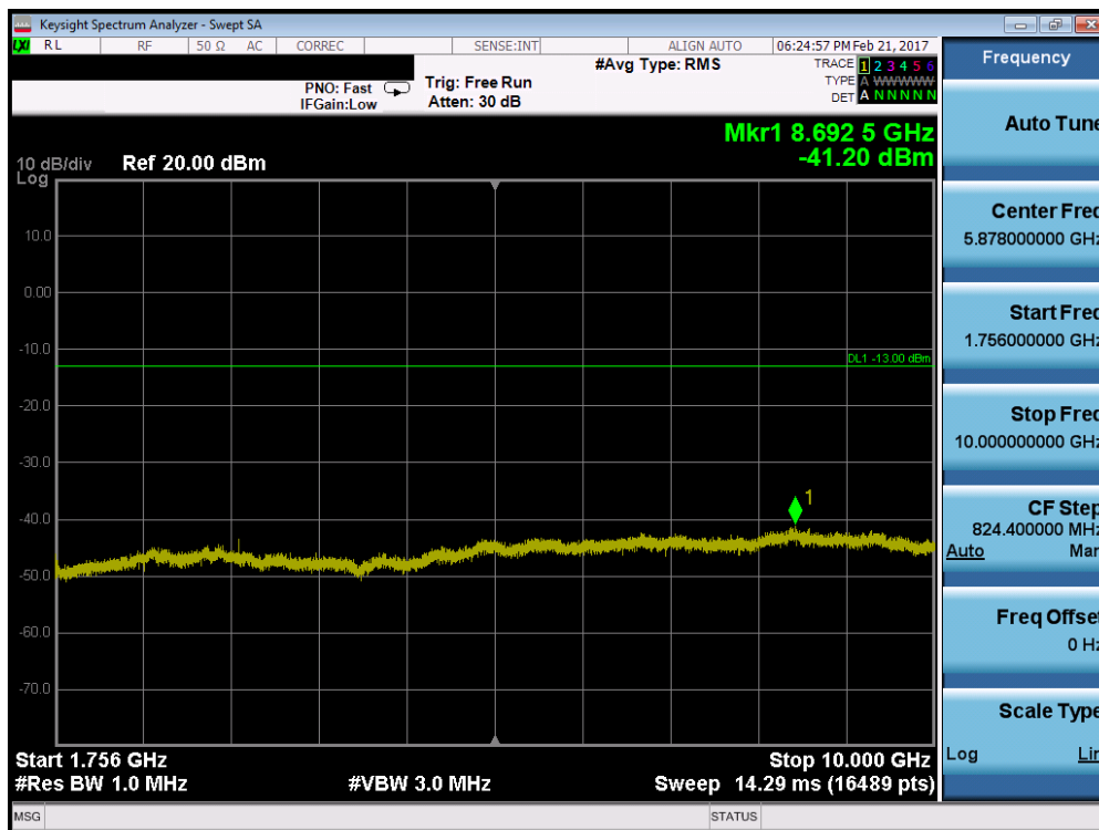
Plot 7-44. Conducted Spurious Plot (Band 4 – 20.0MHz QPSK – RB Size 1, RB Offset 0 – High Channel)
