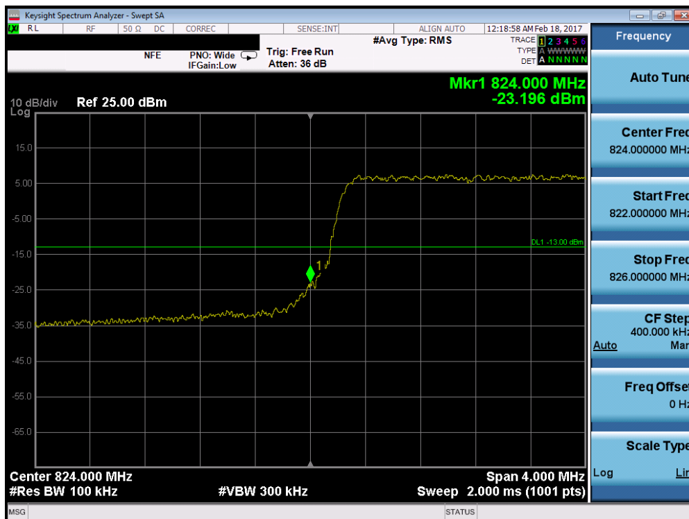
Plot 7-58. Lower Band Edge Plot (Band 5 – 5.0MHz QPSK – RB Size 25)
