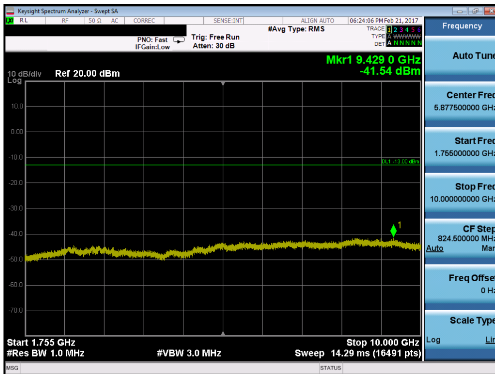
Plot 7-38. Conducted Spurious Plot (Band 4 – 20.0MHz QPSK – RB Size 1, RB Offset 0 – Low Channel)
