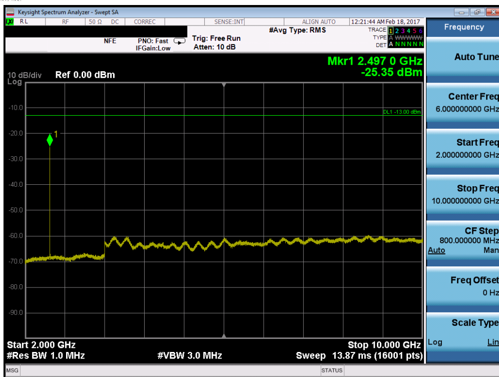
Plot 7-33. Conducted Spurious Plot (Band 5 – 10.0MHz QPSK – RB Size 1, RB Offset 0 – Mid Channel)
