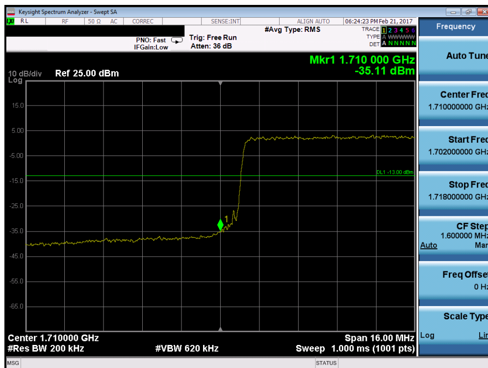
Plot 7-82. Lower Band Edge Plot (Band 4 – 20.0MHz QPSK – RB Size 100)
