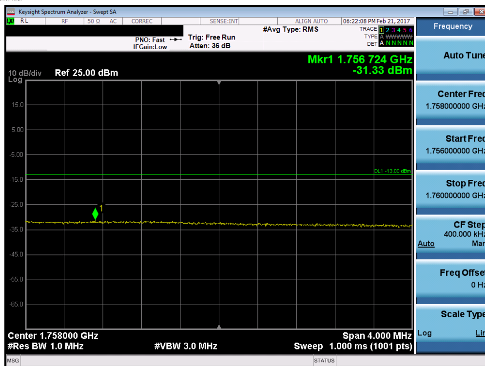
Plot 7-81. Upper Extended Band Edge Plot (Band 4 – 15.0MHz QPSK – RB Size 75)
