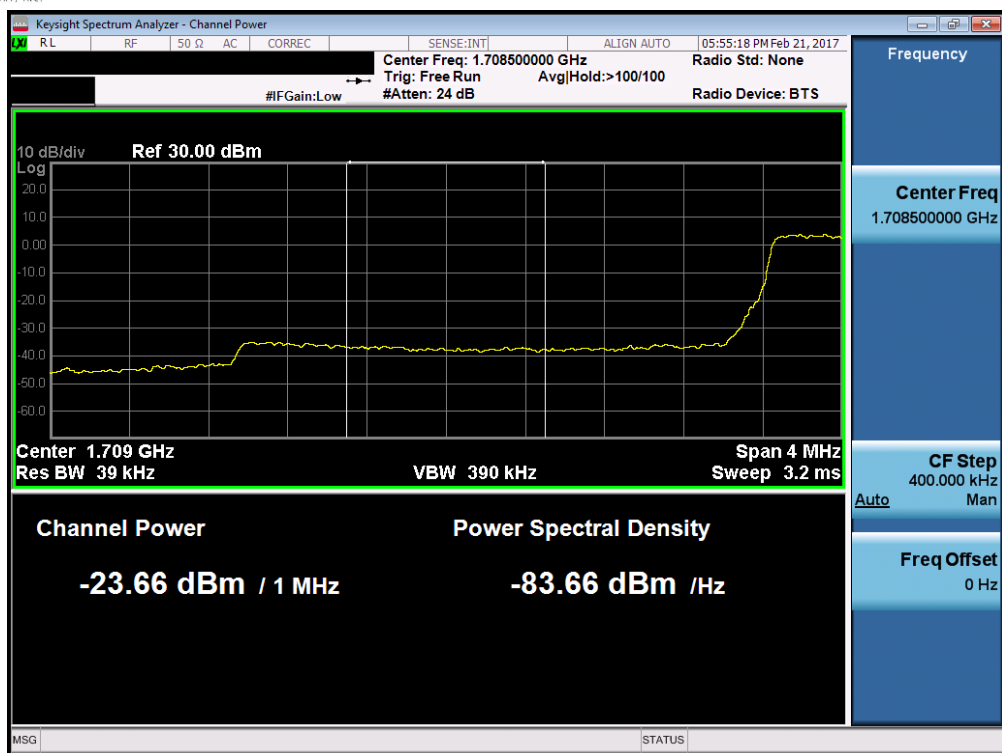
Plot 7-67. Lower Extended Band Edge Plot (Band 4 – 3.0MHz QPSK – RB Size 15)
