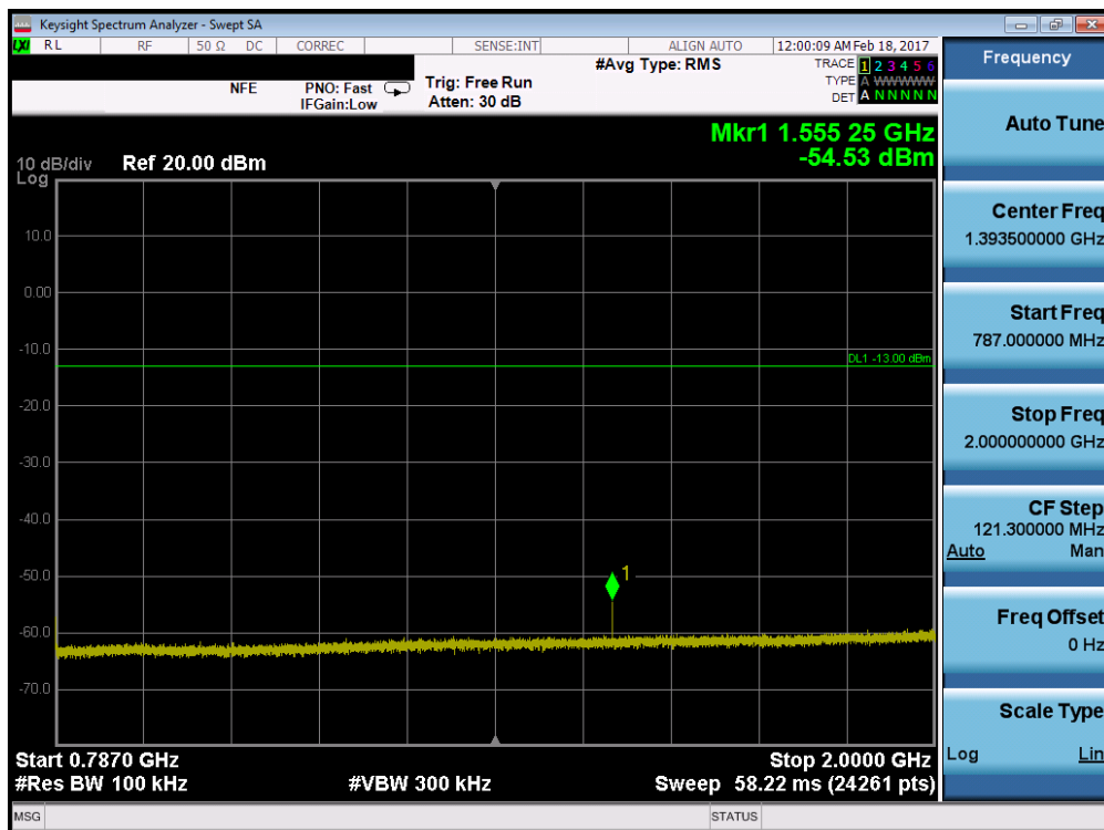
Plot 7-26. Conducted Spurious Plot (Band 13 – 10.0MHz QPSK – RB Size 1, RB Offset 0)
