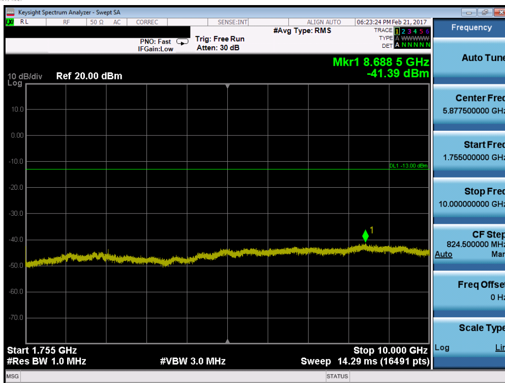
Plot 7-41. Conducted Spurious Plot (Band 4 – 20.0MHz QPSK – RB Size 1, RB Offset 0 – Mid Channel)
