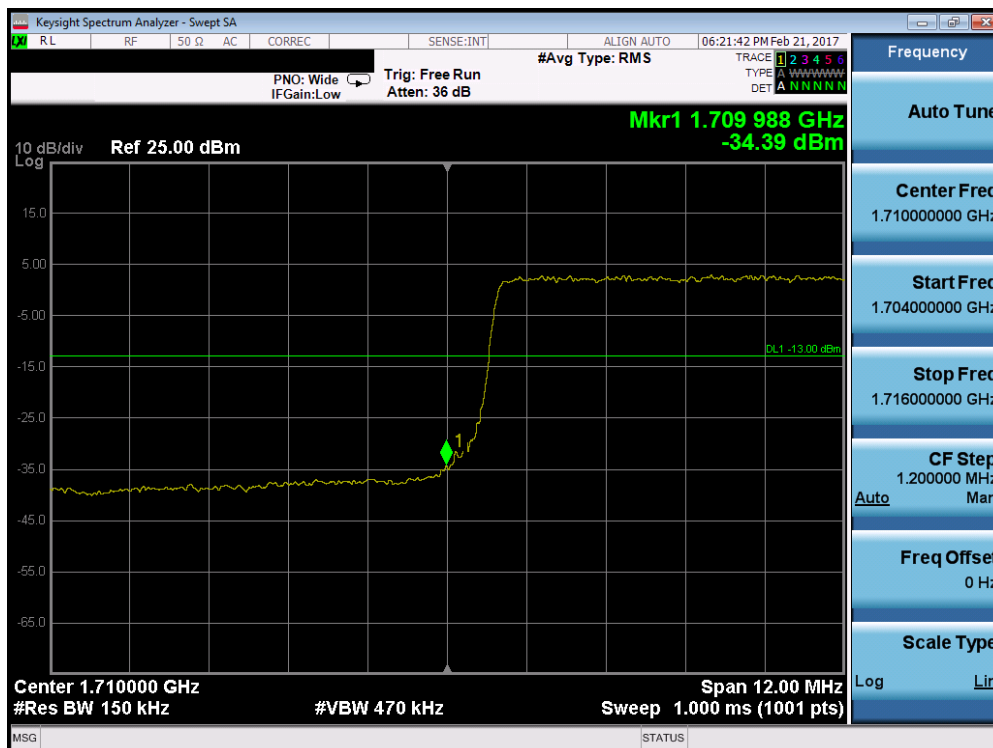
Plot 7-78. Lower Band Edge Plot (Band 4 – 15.0MHz QPSK – RB Size 75)
