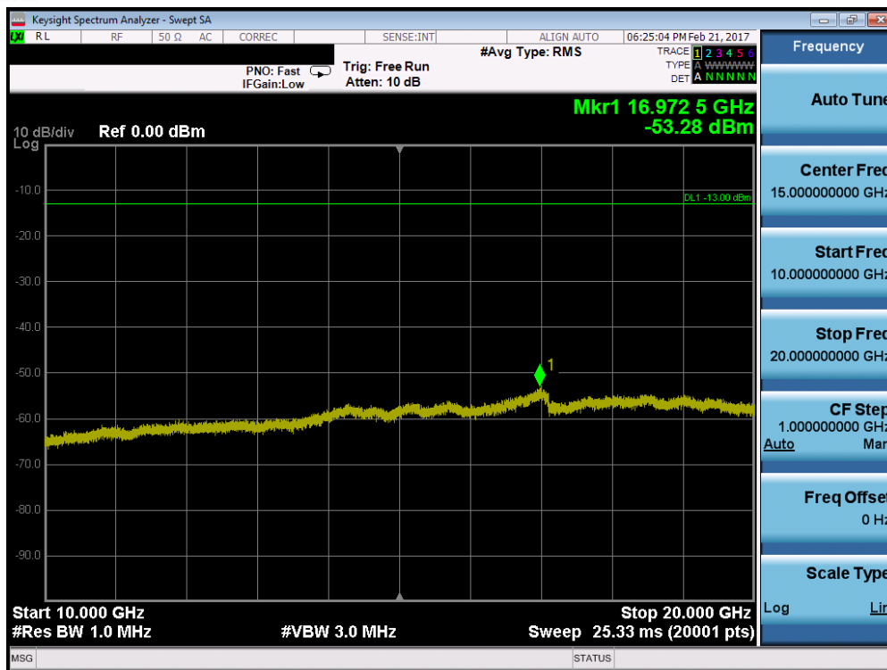
Plot 7-45. Conducted Spurious Plot (Band 4 – 20.0MHz QPSK – RB Size 1, RB Offset 0 – High Channel)
