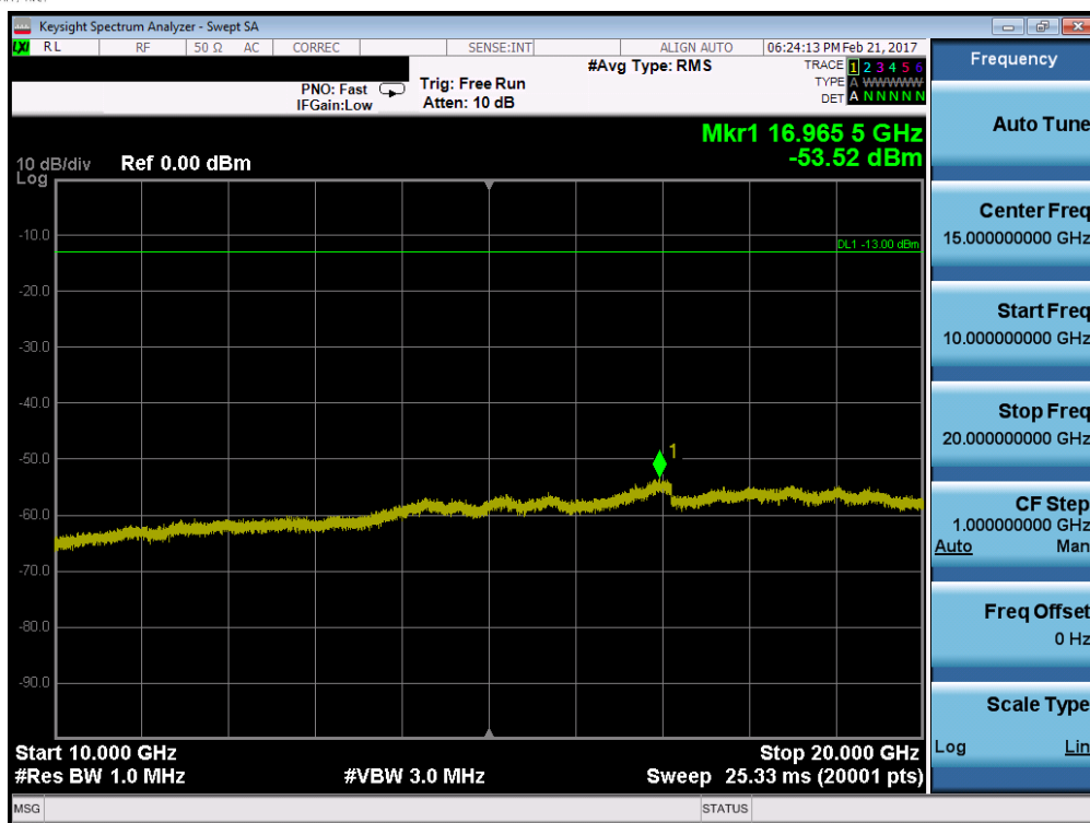
Plot 7-39. Conducted Spurious Plot (Band 4 – 20.0MHz QPSK – RB Size 1, RB Offset 0 – Low Channel)
