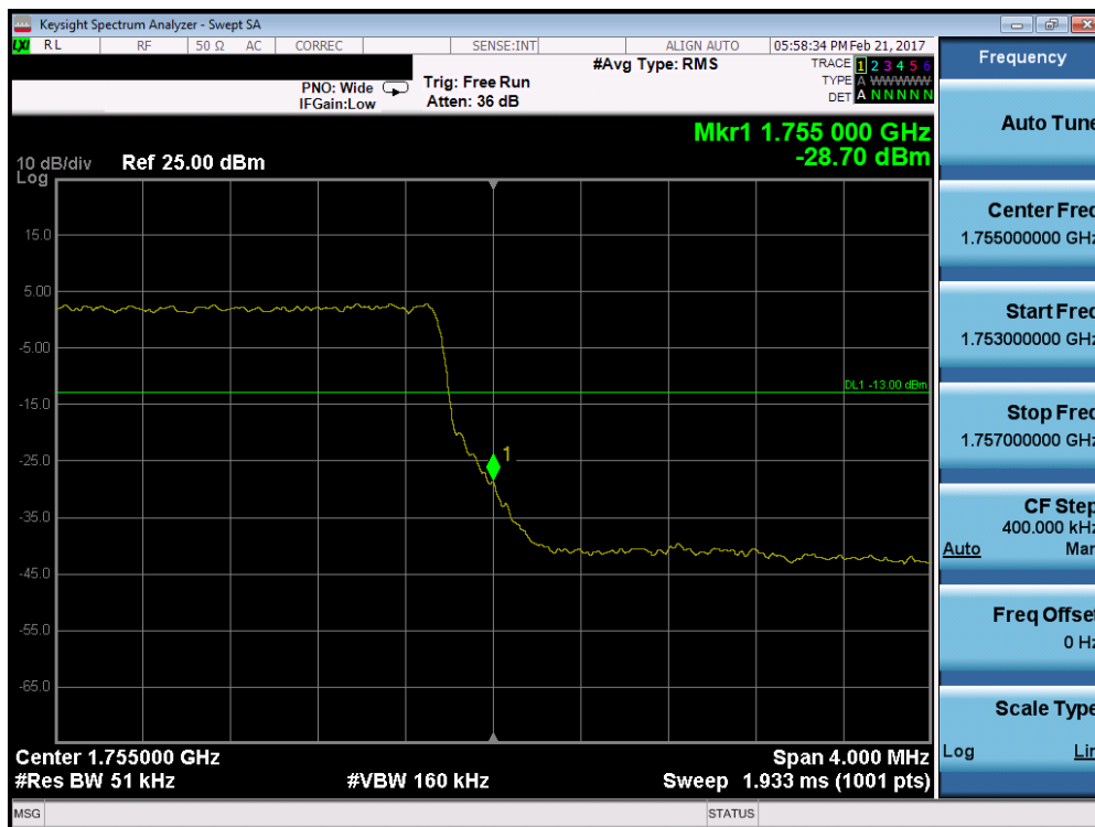
Plot 7-72. Upper Band Edge Plot (Band 4 - 5.0MHz QPSK - RB Size 25)
