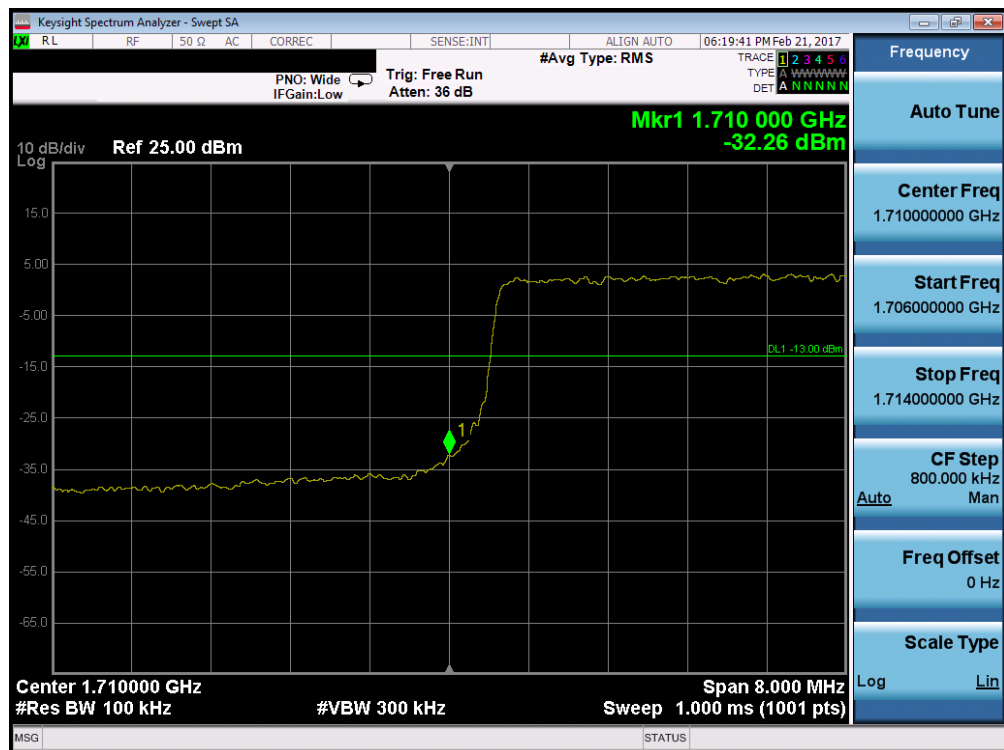
Plot 7-74. Lower Band Edge Plot (Band 4 – 10.0MHz QPSK – RB Size 50)
