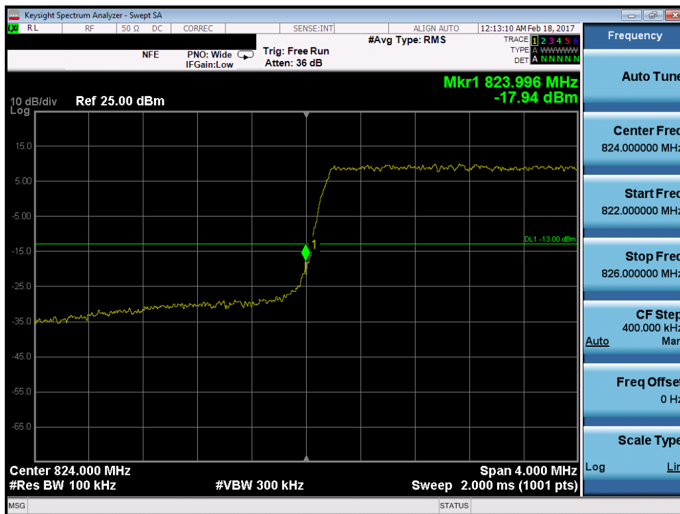
Plot 7-56. Lower Band Edge Plot (Band 5 – 3.0MHz QPSK – RB Size 15)
