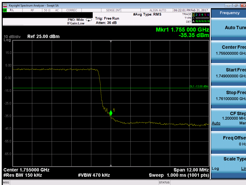
Plot 7-80. Upper Band Edge Plot (Band 4 - 15.0MHz QPSK - RB Size 75)
