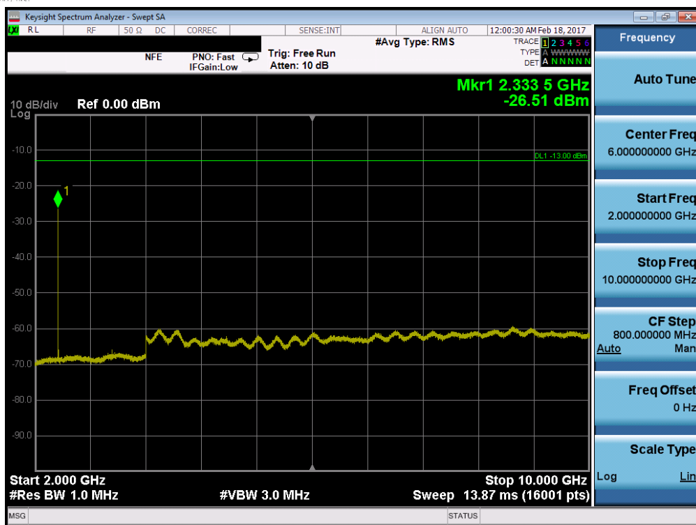
Plot 7-27. Conducted Spurious Plot (Band 13 – 10.0MHz QPSK – RB Size 1, RB Offset 0)
