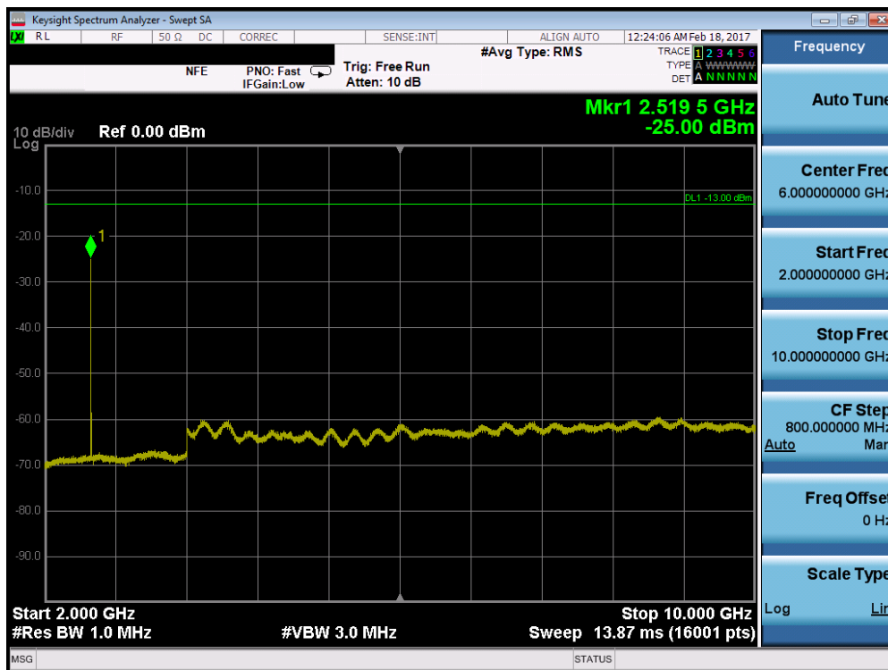
Plot 7-36. Conducted Spurious Plot (Band 5 – 10.0MHz QPSK – RB Size 1, RB Offset 0 – High Channel)
