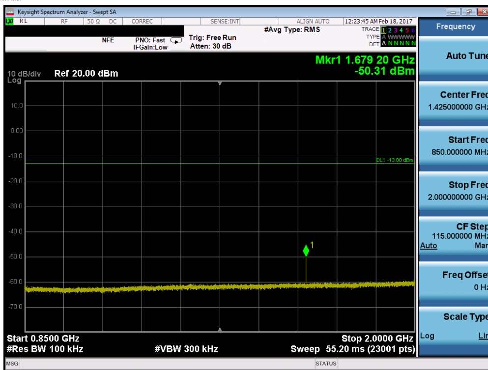
Plot 7-35. Conducted Spurious Plot (Band 5 – 10.0MHz QPSK – RB Size 1, RB Offset 0 – High Channel)
