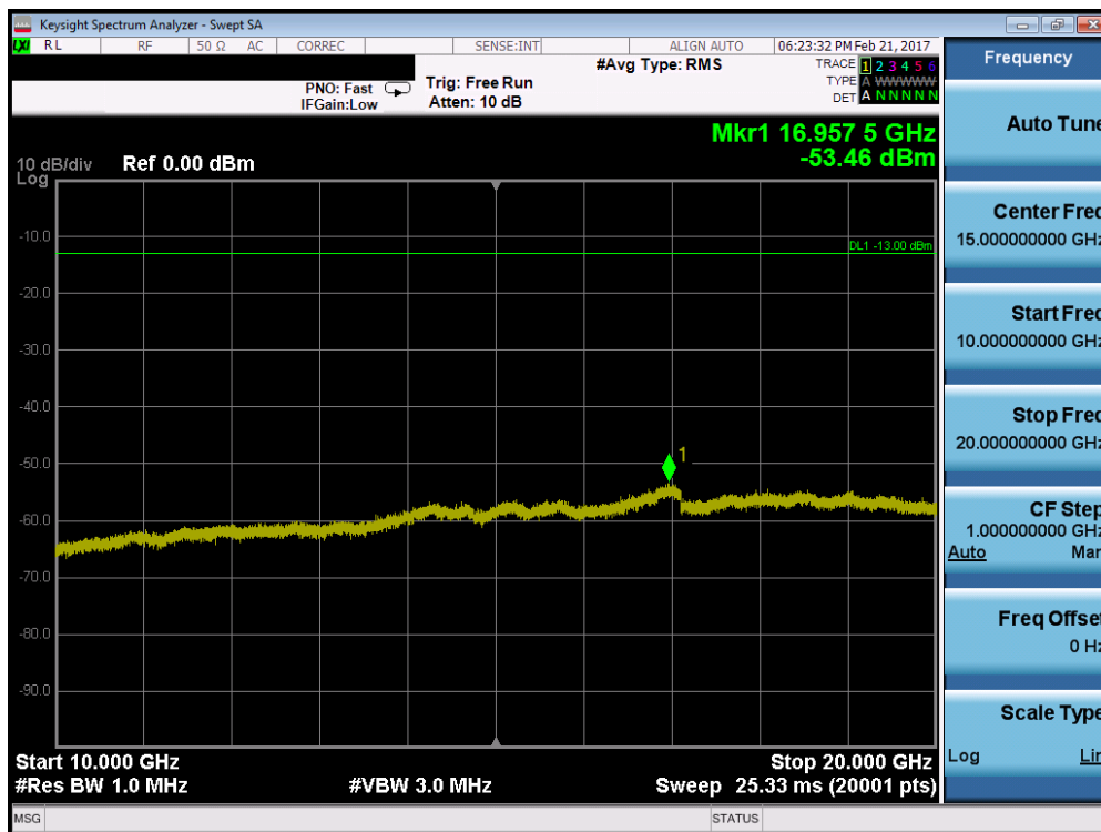
Plot 7-42. Conducted Spurious Plot (Band 4 – 20.0MHz QPSK – RB Size 1, RB Offset 0 – Mid Channel)
