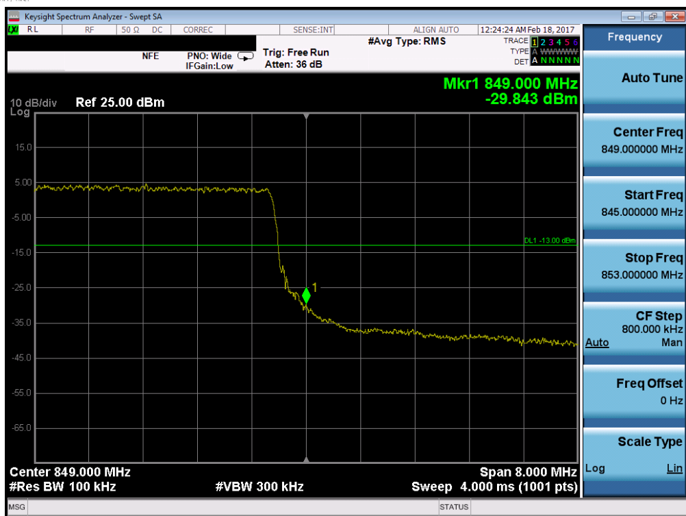
Plot 7-61. Upper Band Edge Plot (Band 5 - 10.0MHz QPSK - RB Size 50)
