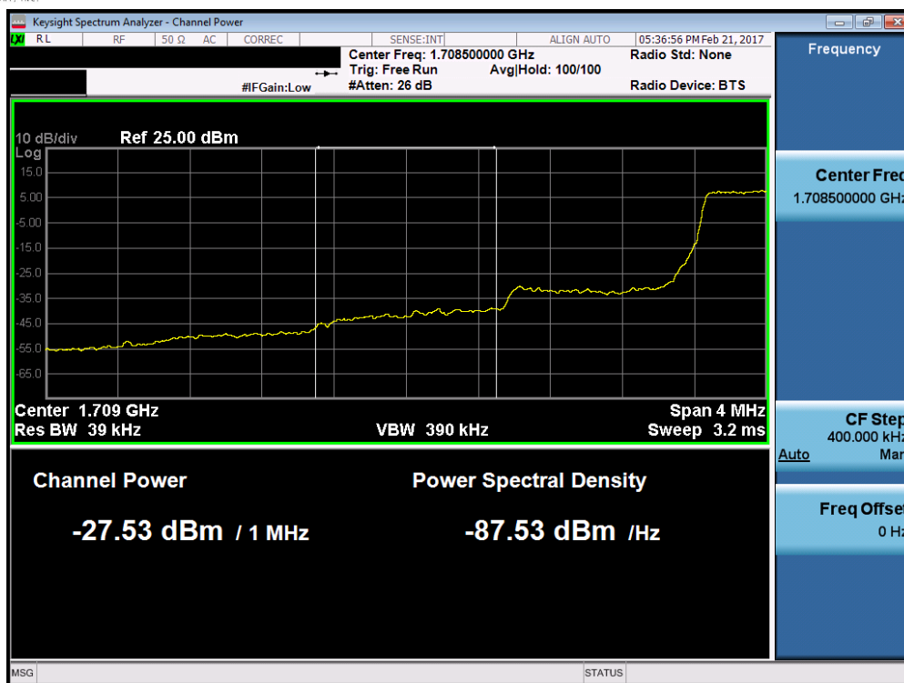
Plot 7-63. Lower Extended Band Edge Plot (Band 4 – 1.4MHz QPSK – RB Size 6)
