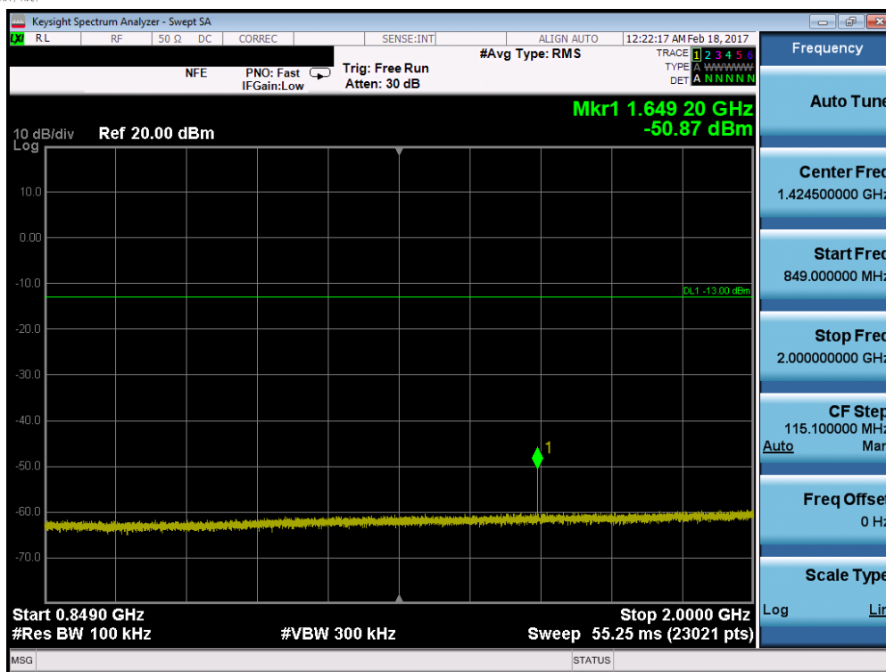
Plot 7-29. Conducted Spurious Plot (Band 5 – 10.0MHz QPSK – RB Size 1, RB Offset 0 – Low Channel)
