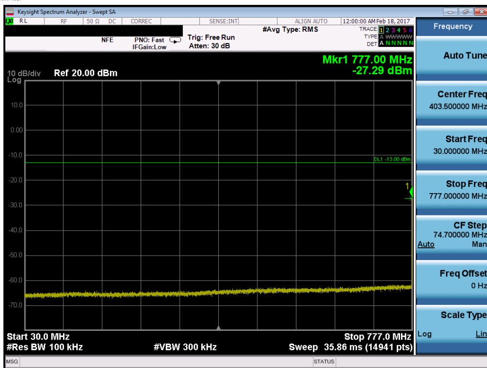
Plot 7-25. Conducted Spurious Plot (Band 13 – 10.0MHz QPSK – RB Size 1, RB Offset 0)
