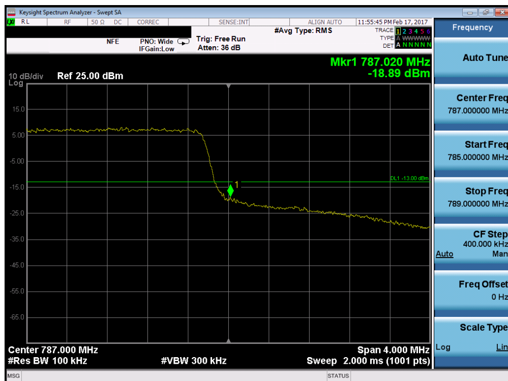
Plot 7-48. Upper Band Edge Plot (Band 13 - 5.0MHz QPSK - RB Size 25)
