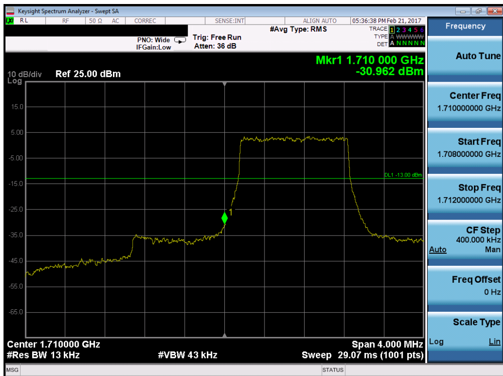
Plot 7-62. Lower Band Edge Plot (Band 4 - 1.4MHz QPSK - RB Size 6)
