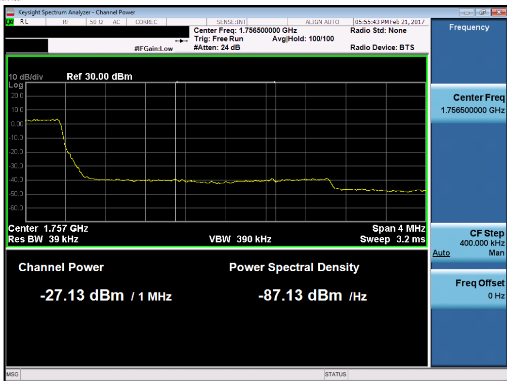
Plot 7-69. Upper Extended Band Edge Plot (Band 4 – 3.0MHz QPSK – RB Size 15)
