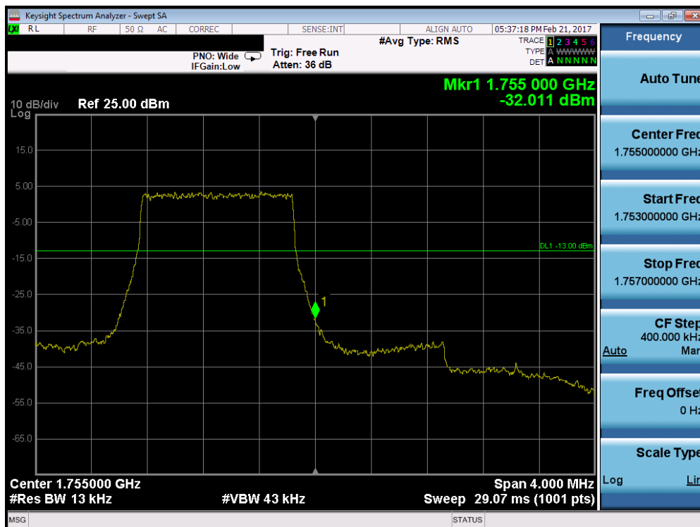
Plot 7-64. Upper Band Edge Plot (Band 4 – 1.4MHz QPSK – RB Size 6)
