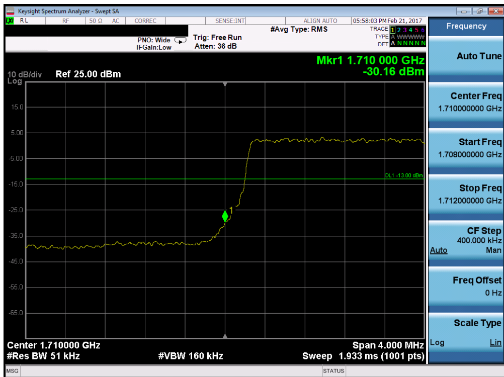
Plot 7-70. Lower Band Edge Plot (Band 4 – 5.0MHz QPSK – RB Size 25)
