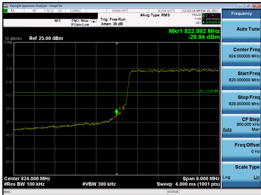
Plot 7-60. Lower Band Edge Plot (Band 5 – 10.0MHz QPSK – RB Size 50)
