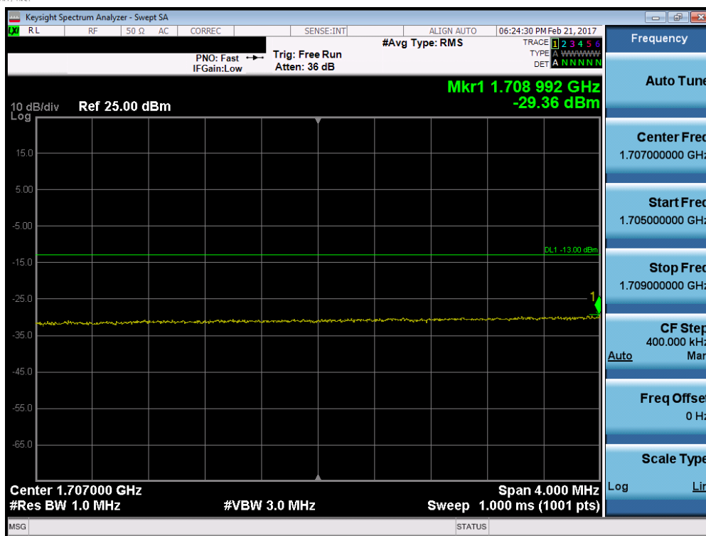
Plot 7-83. Lower Extended Band Edge Plot (Band 4 – 20.0MHz QPSK – RB Size 100)
