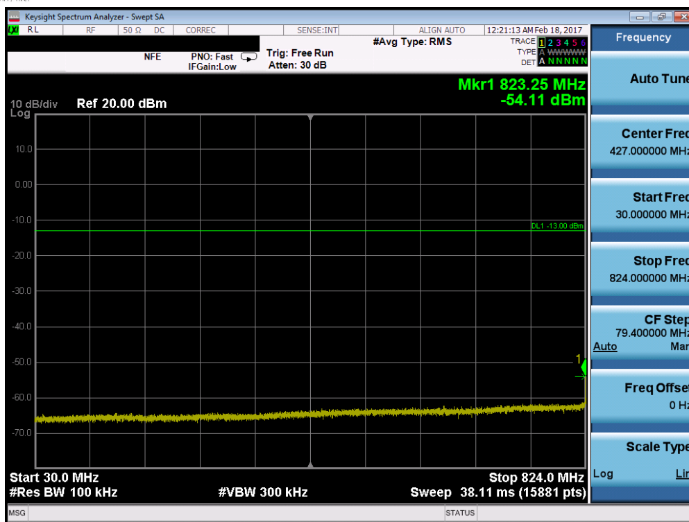
Plot 7-31. Conducted Spurious Plot (Band 5 – 10.0MHz QPSK – RB Size 1, RB Offset 0 – Mid Channel)
