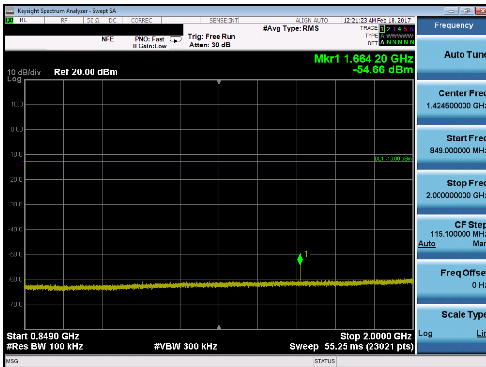
Plot 7-32. Conducted Spurious Plot (Band 5 – 10.0MHz QPSK – RB Size 1, RB Offset 0 – Mid Channel)
