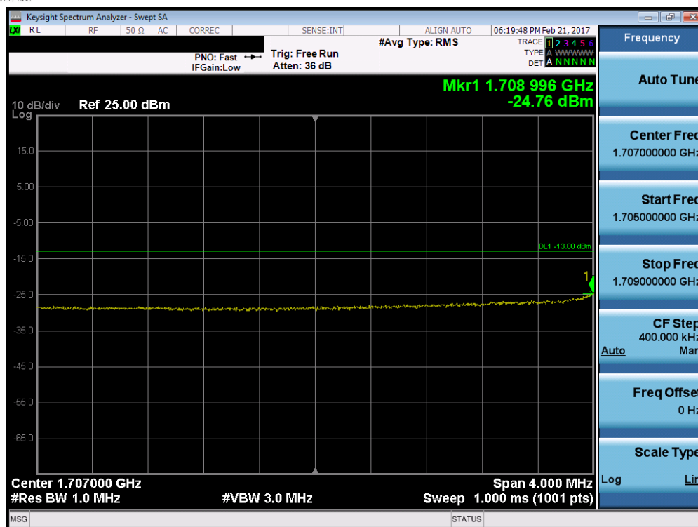
Plot 7-75. Lower Extended Band Edge Plot (Band 4 - 10.0MHz QPSK - RB Size 50)
