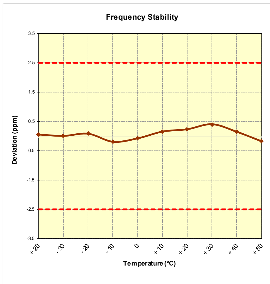
Figure 7-7. Frequency Stability Graph (Band 13)
