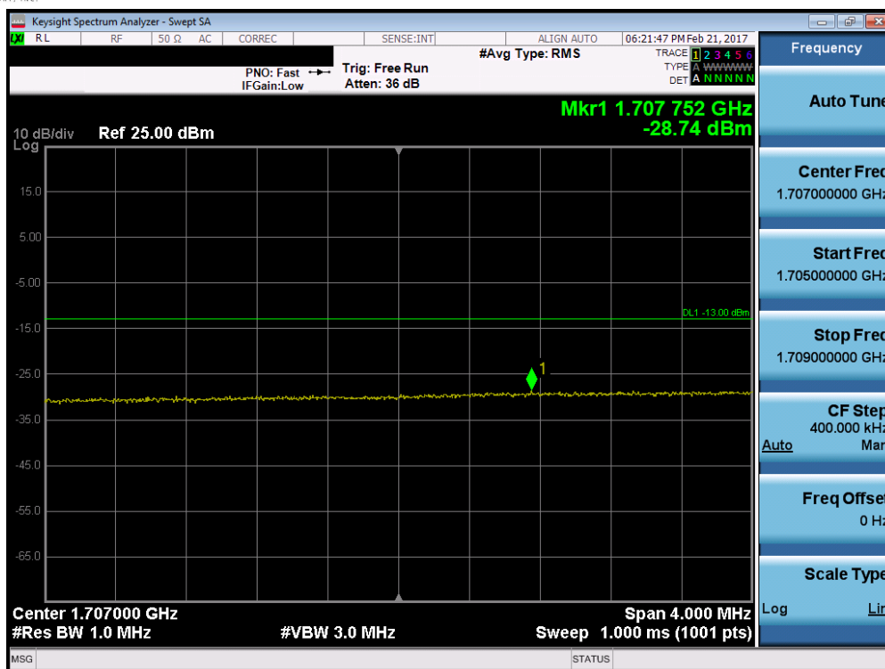
Plot 7-79. Lower Extended Band Edge Plot (Band 4 - 15.0MHz QPSK - RB Size 75)
