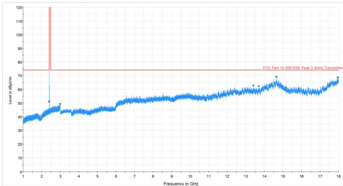
Plot 7-2. Radiated Spurious Plot above 1GHz (BT – Ch. 0, Ant. Pol. V)
