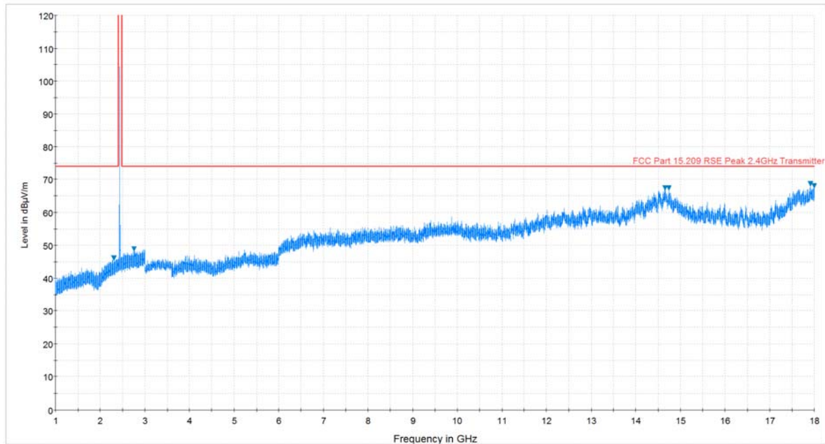
Plot 7-3. Radiated Spurious Plot above 1GHz (BT – Ch. 39, Ant. Pol. H)
