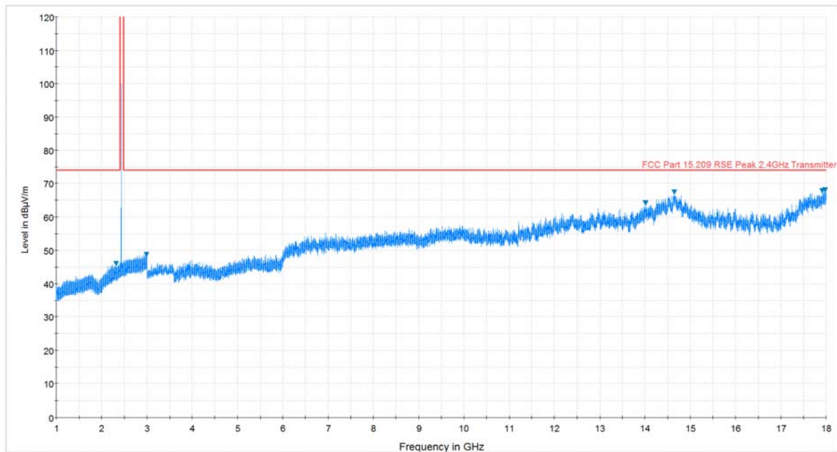
Plot 7-4. Radiated Spurious Plot above 1GHz (BT – Ch. 39, Ant. Pol. V)
