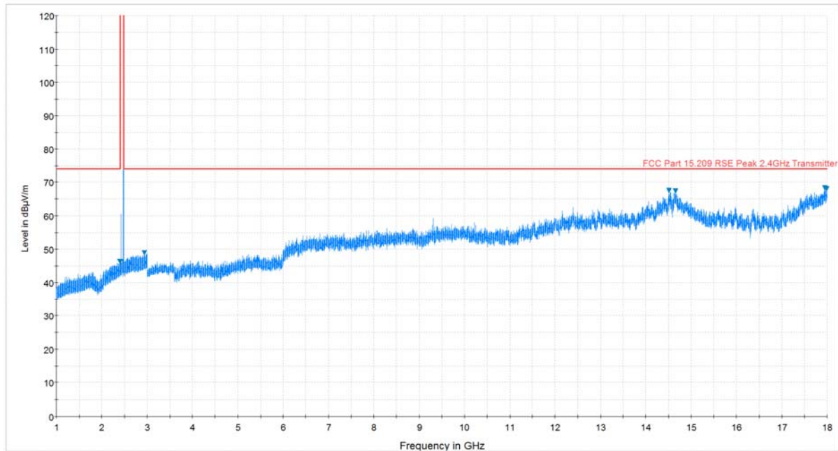
Plot 7-5. Radiated Spurious Plot above 1GHz (BT – Ch. 78, Ant. Pol. H)
