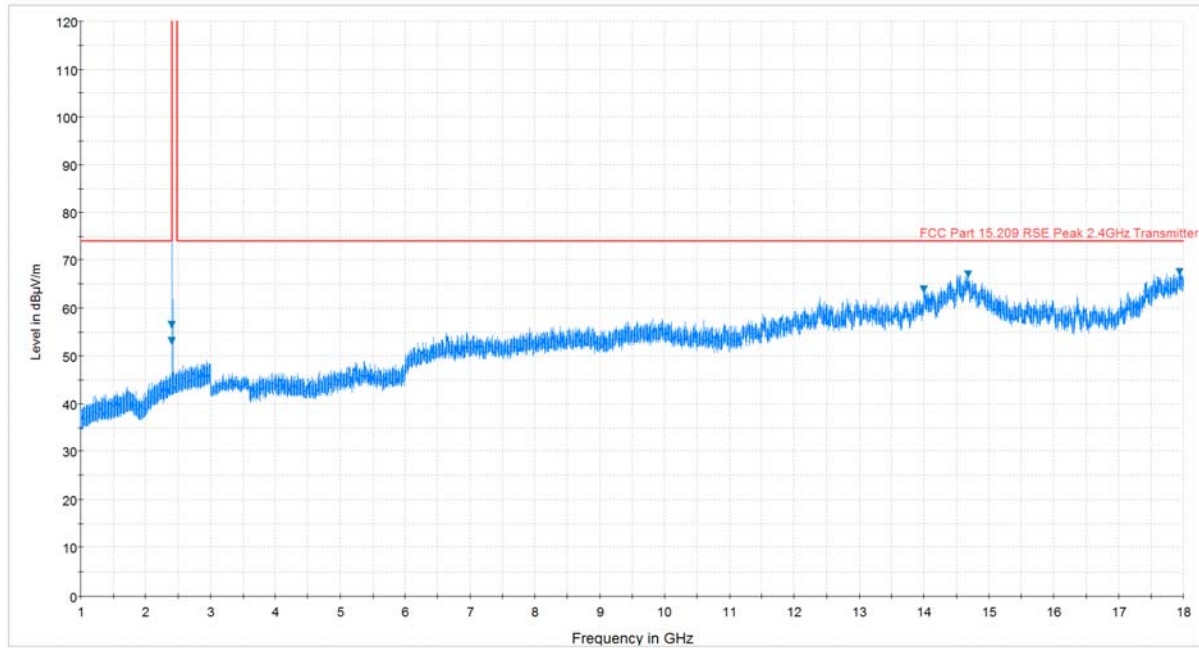
Plot 7-1. Radiated Spurious Plot above 1GHz (BT – Ch. 0, Ant. Pol. H)
