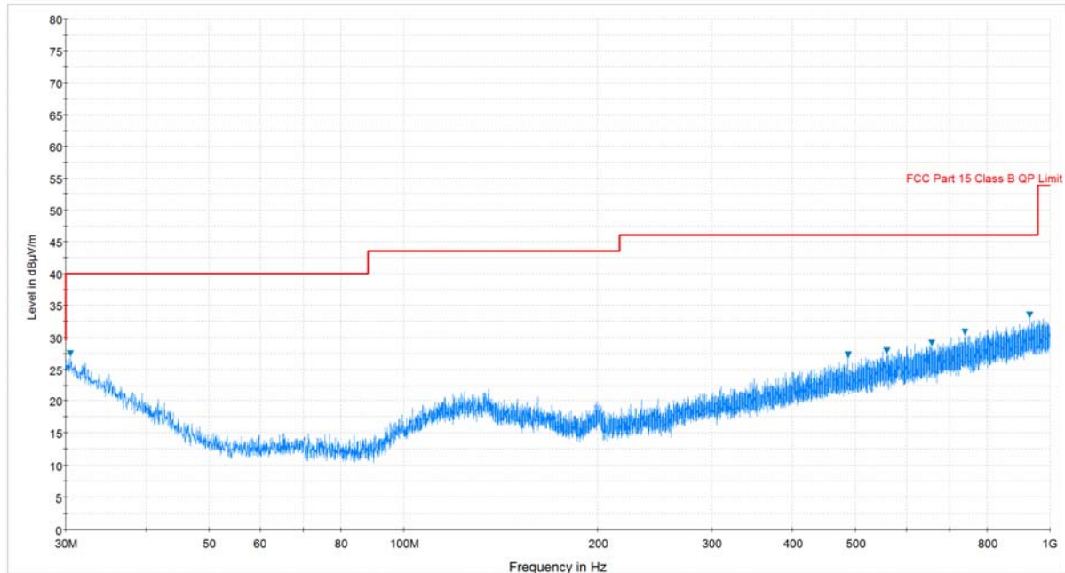
Plot 7-11. Radiated Spurious Plot below 1GHz (Pol. H)
