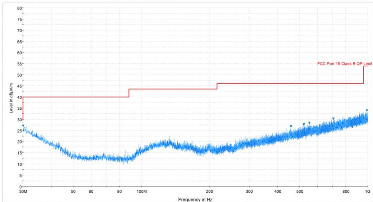
Plot 7-12. Radiated Spurious Plot below 1GHz (Pol. V)
