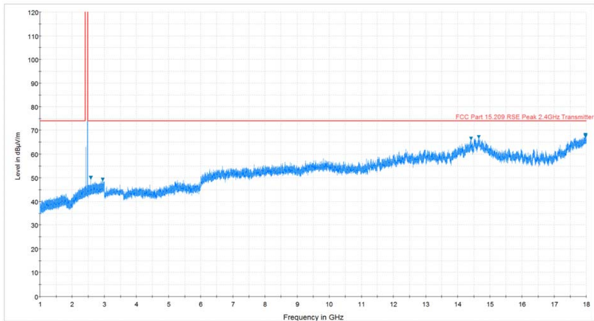
Plot 7-6. Radiated Spurious Plot above 1GHz (BT – Ch. 78, Ant. Pol. V)
