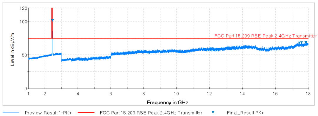
Plot 7-41. Radiated Spurious Plot above 1GHz (802.11b – Ch. 11, Ant. Pol. H)
