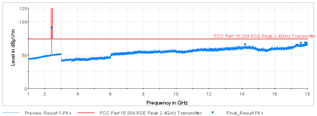
Plot 7-38. Radiated Spurious Plot above 1GHz (802.11b – Ch. 1, Ant. Pol. V)
