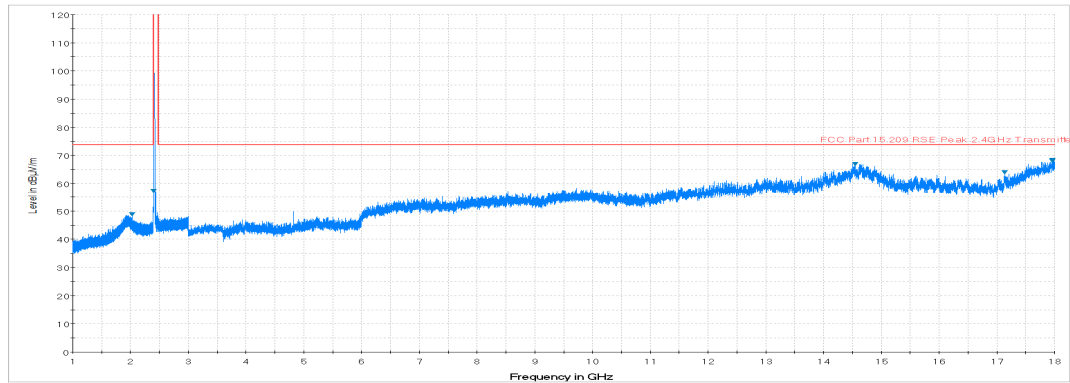
Plot 7-37. Radiated Spurious Plot above 1GHz (802.11b – Ch. 1, Ant. Pol. H)
