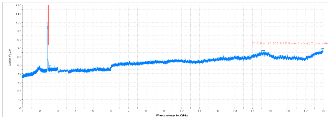
Plot 7-39. Radiated Spurious Plot above 1GHz (802.11b – Ch. 6, Ant. Pol. H)
