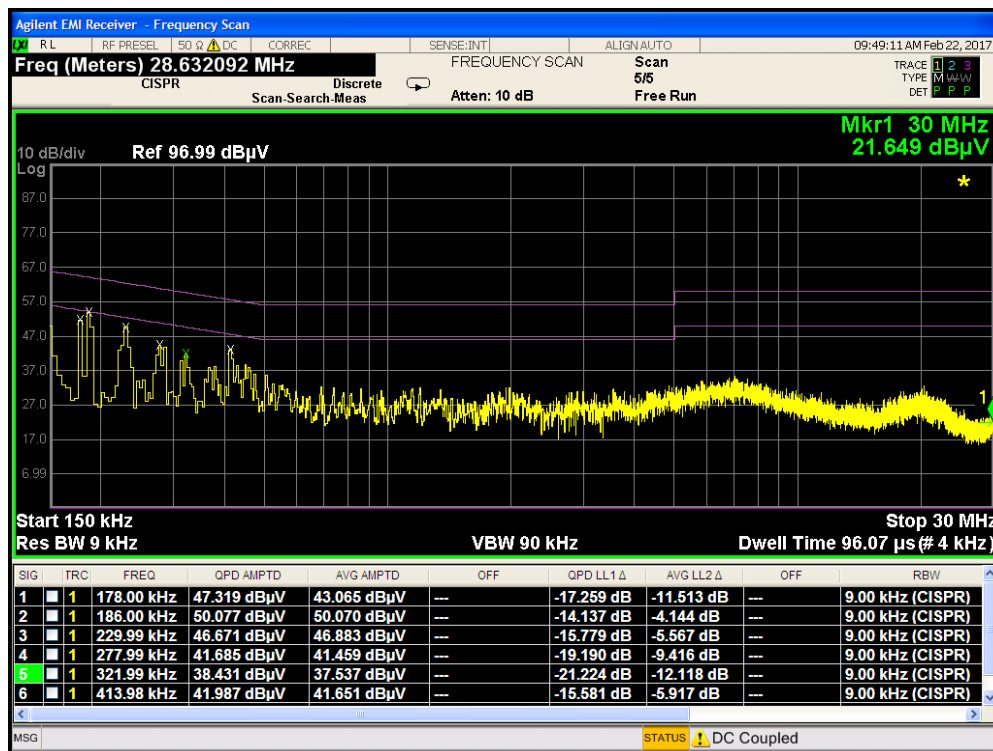
Plot 7-52. Line Conducted Plot with 802.11b (N)
