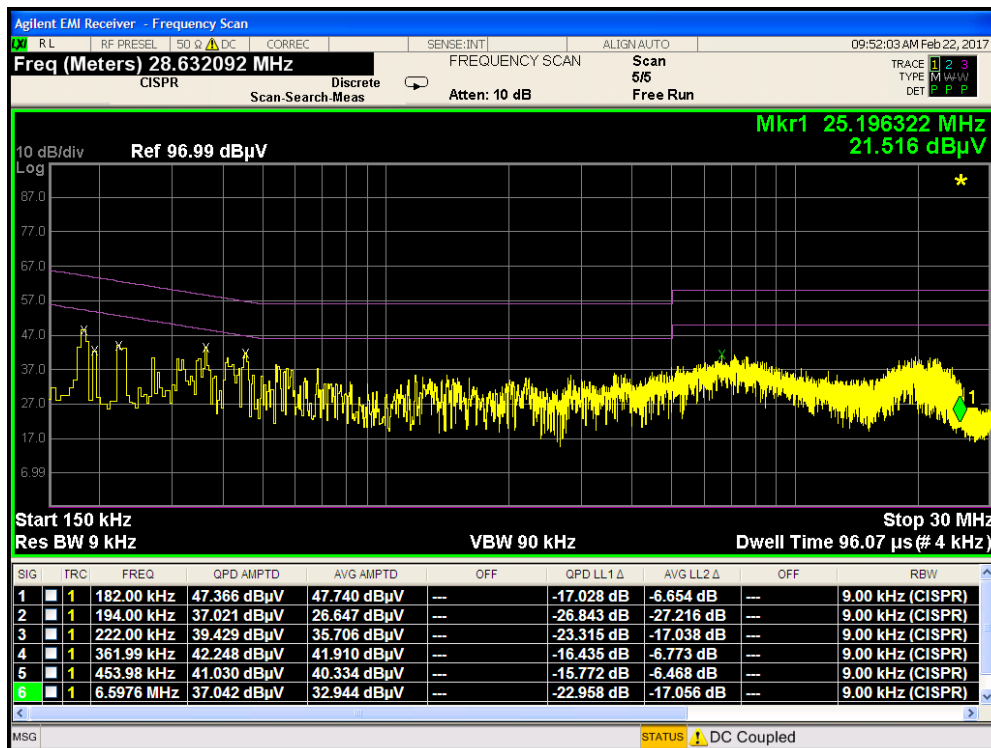
Plot 7-51. Line Conducted Plot with 802.11b (L1)
