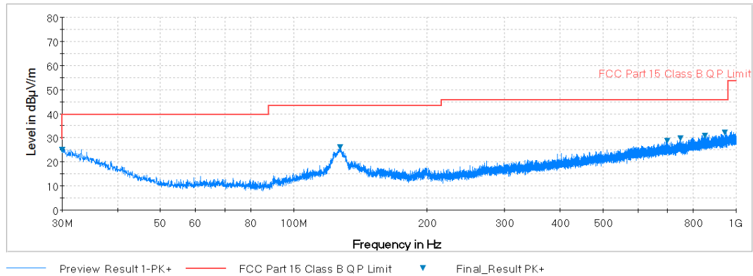
Plot 7-50. Radiated Spurious Plot below 1GHz (Pol. V)
