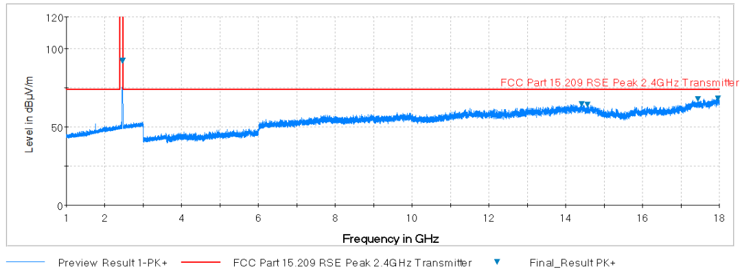
Plot 7-42. Radiated Spurious Plot above 1GHz (802.11b – Ch. 11, Ant. Pol. V)
