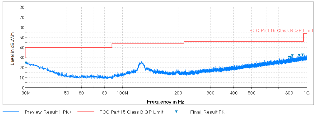
Plot 7-49. Radiated Spurious Plot below 1GHz (Pol. H)
