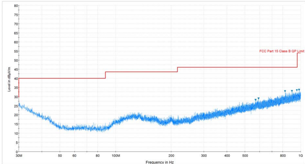
Plot 7-17. Radiated Spurious Plot below 1GHz (Pol. H)
