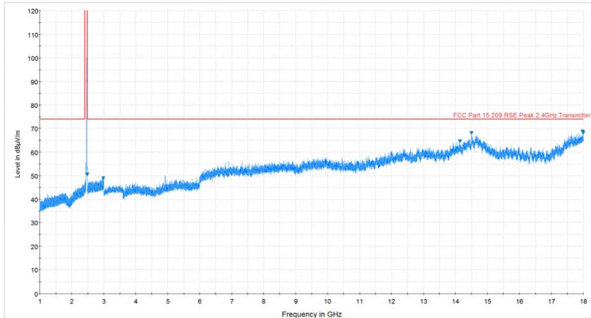
Plot 7-5. Radiated Spurious Plot above 1GHz (802.11b – Ch. 11, Ant. Pol. H)
