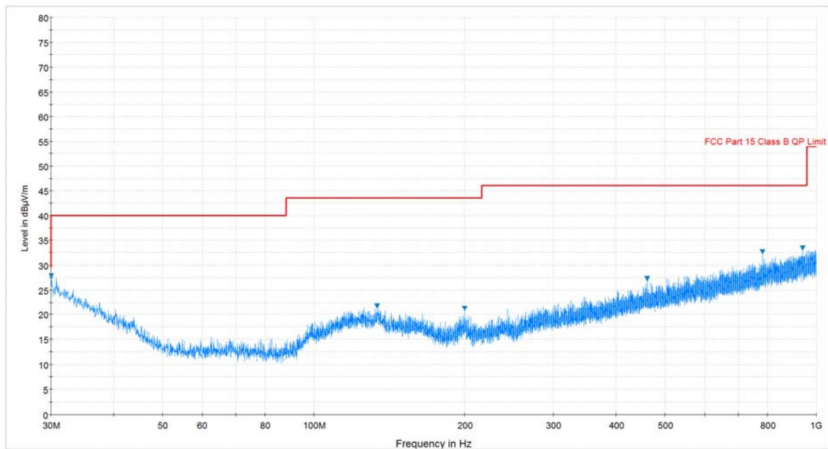
Plot 7-18. Radiated Spurious Plot below 1GHz (Pol. V)
