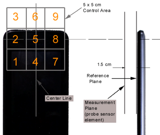
Figure 17-3 5x5 Scan grid above WD
