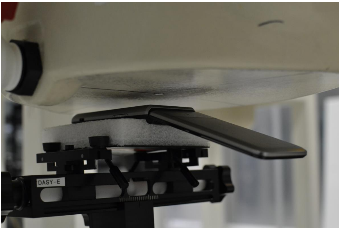
SAR Test Setup Photo 7 – Back Side in Open Position at 10 mm
