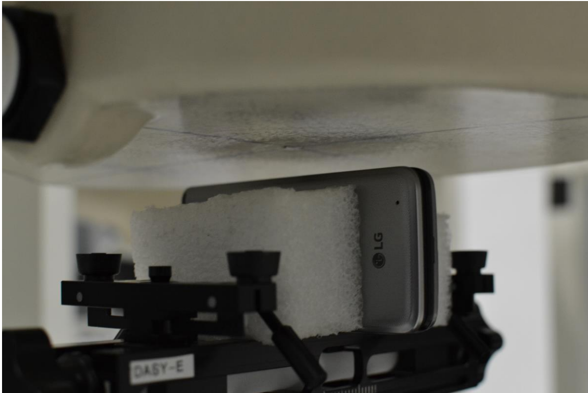
SAR Test Setup Photo 11 – Right Edge at 10 mm
