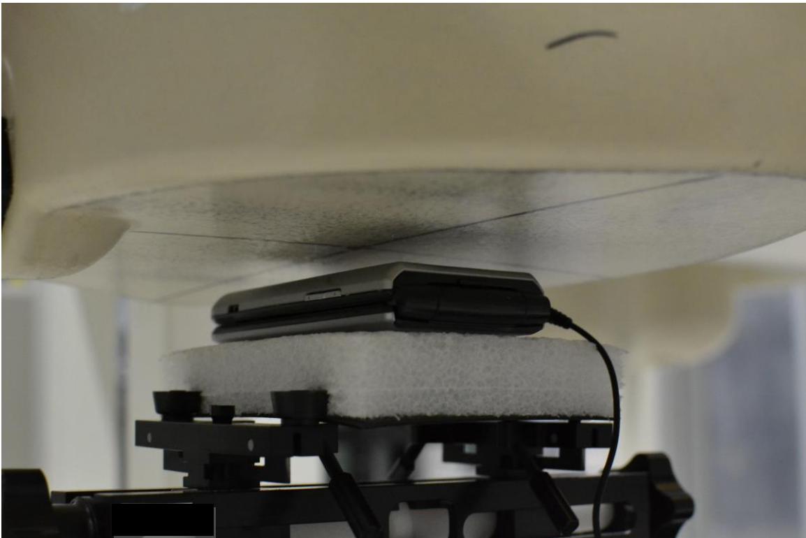
SAR Test Setup Photo 6 – Back Side with Headphones at 10 mm
