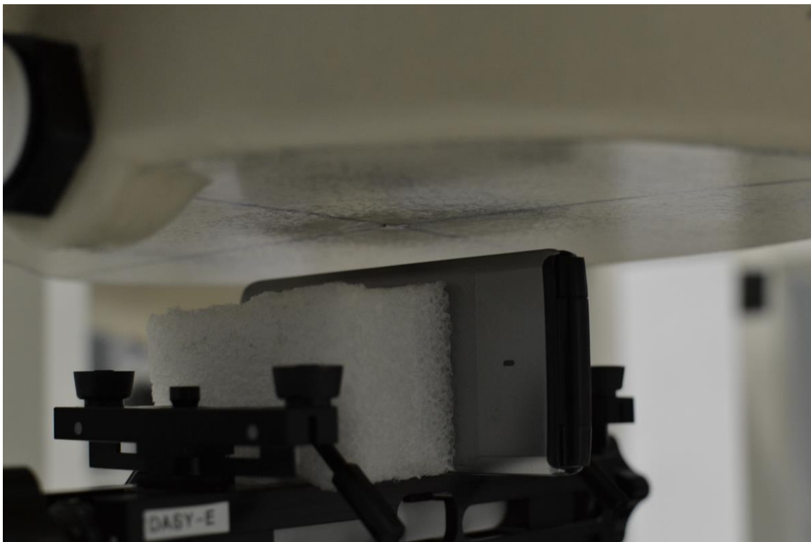
SAR Test Setup Photo 12 – Left Edge at 10 mm
