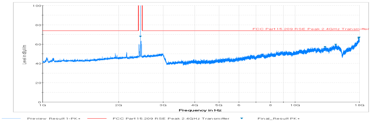
Plot 6-3. Radiated Spurious Plot above 1GHz (BT – Ch. 39, Ant. Pol. H)
