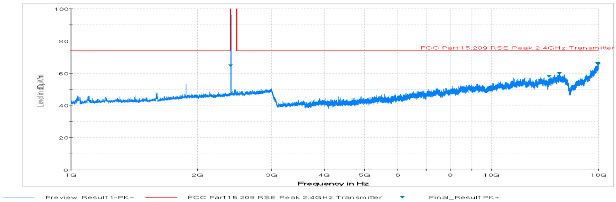
Plot 6-1. Radiated Spurious Plot above 1GHz (BT – Ch. 0, Ant. Pol. H)
