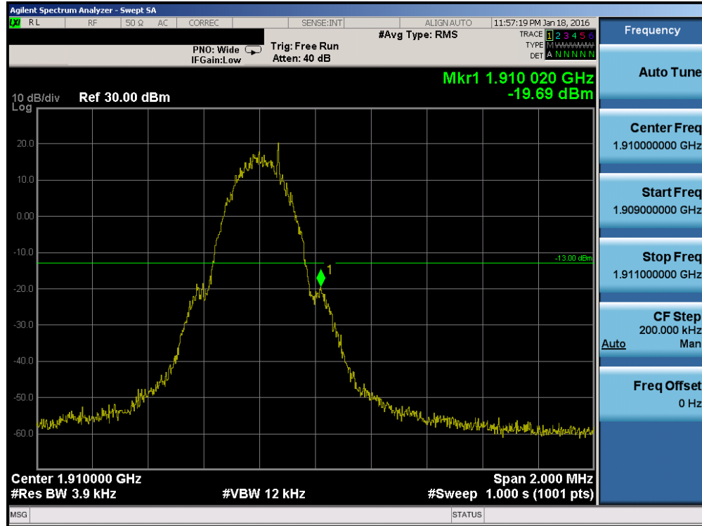
Plot 7-67. Band Edge Plot (PCS GSM Mode – Ch. 810)
