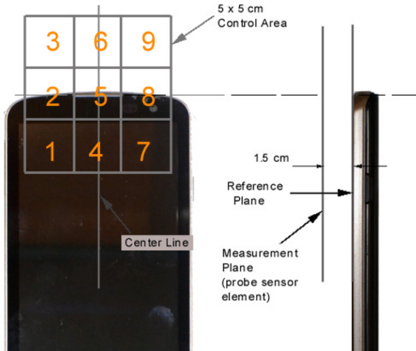
Figure 18-3 5x5 Scan grid above WD
