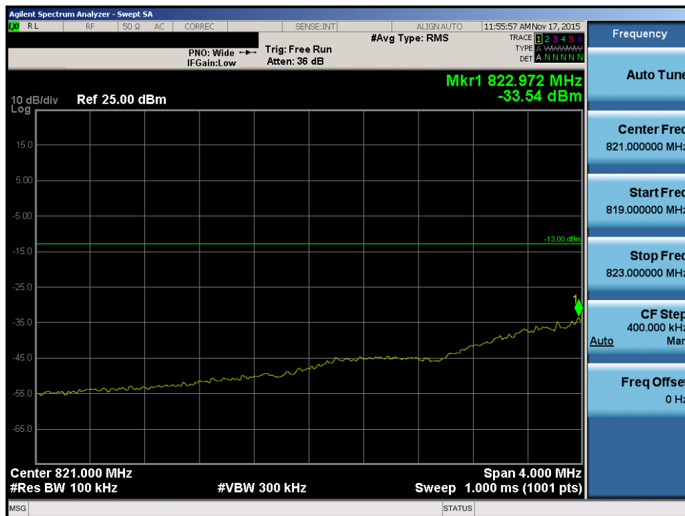
Plot 7-85. Lower Extended Band Edge Plot (Band 5 – 1.4MHz QPSK – RB Size 6)
