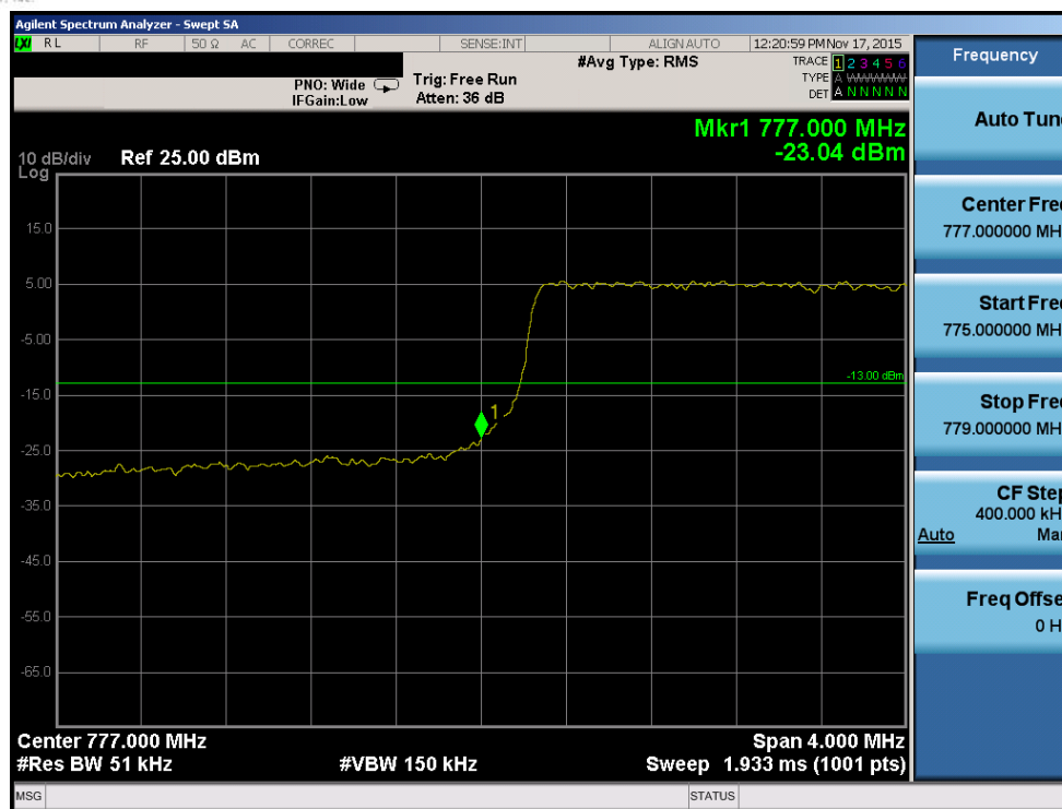
Plot 7-76. Lower Band Edge Plot (Band 13 – 5.0MHz QPSK – RB Size 25)
