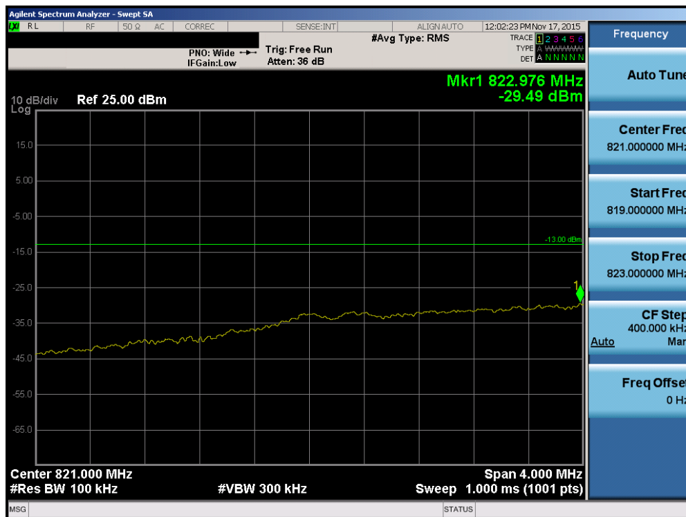
Plot 7-93. Lower Extended Band Edge Plot (Band 5 – 5.0MHz QPSK – RB Size 25)
