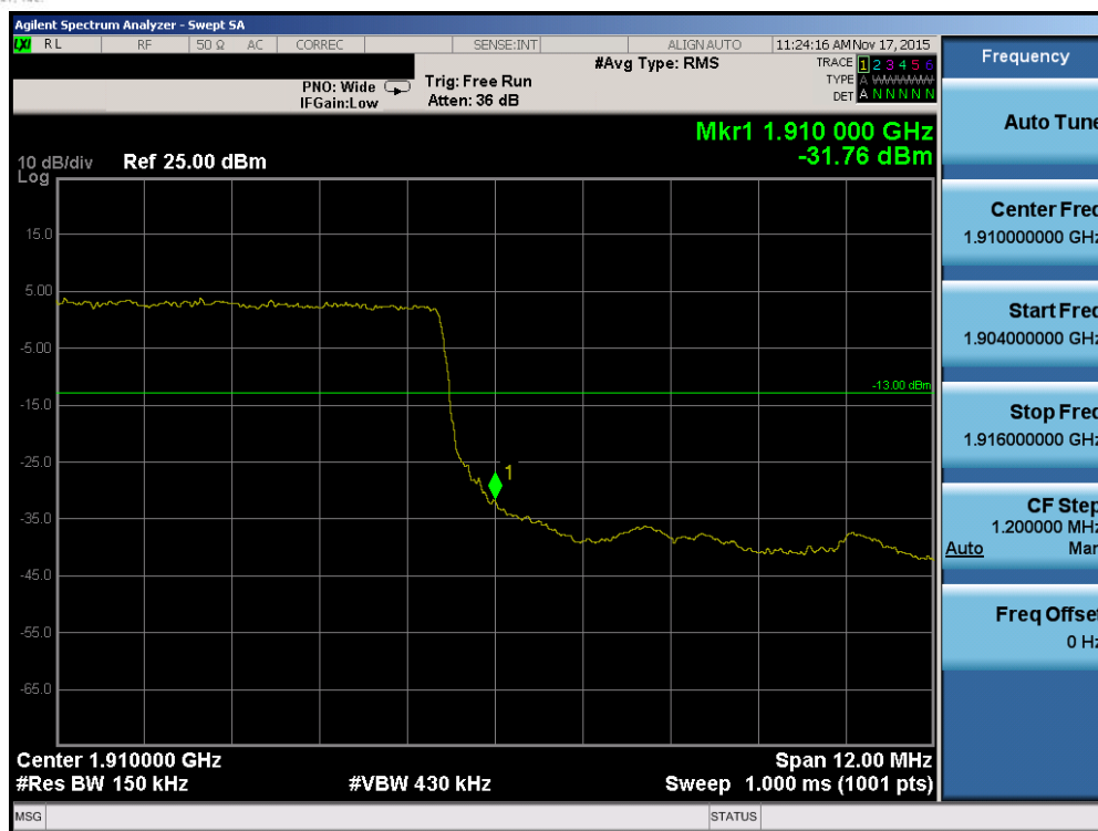
Plot 7-140. Upper Band Edge Plot (Band 2 – 15.0MHz QPSK – RB Size 75)
