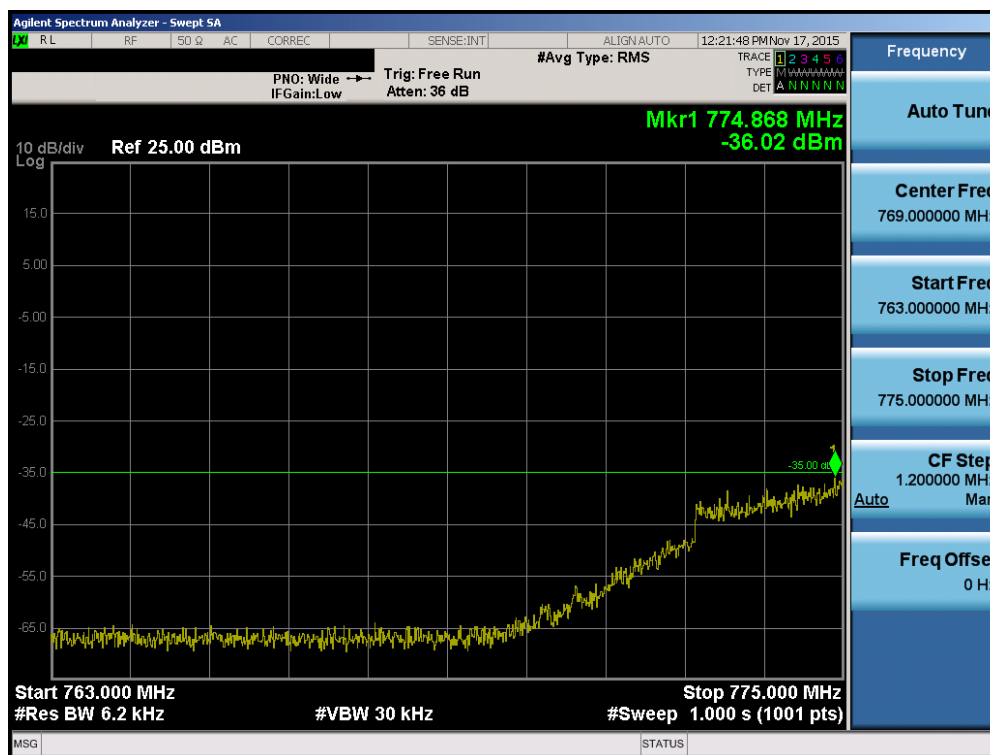
Plot 7-77. Lower Emission Mask Edge Plot (Band 13 – 5.0MHz QPSK – RB Size 25)
