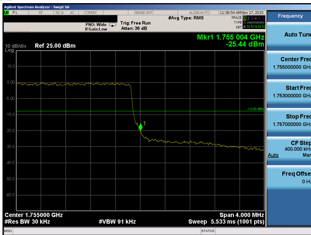
Plot 7-104. Upper Band Edge Plot (Band 4 – 3.0MHz QPSK – RB Size 15)
