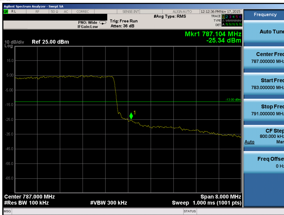
Plot 7-82. Upper Band Edge Plot (Band 13 – 10.0MHz QPSK – RB Size 50)
