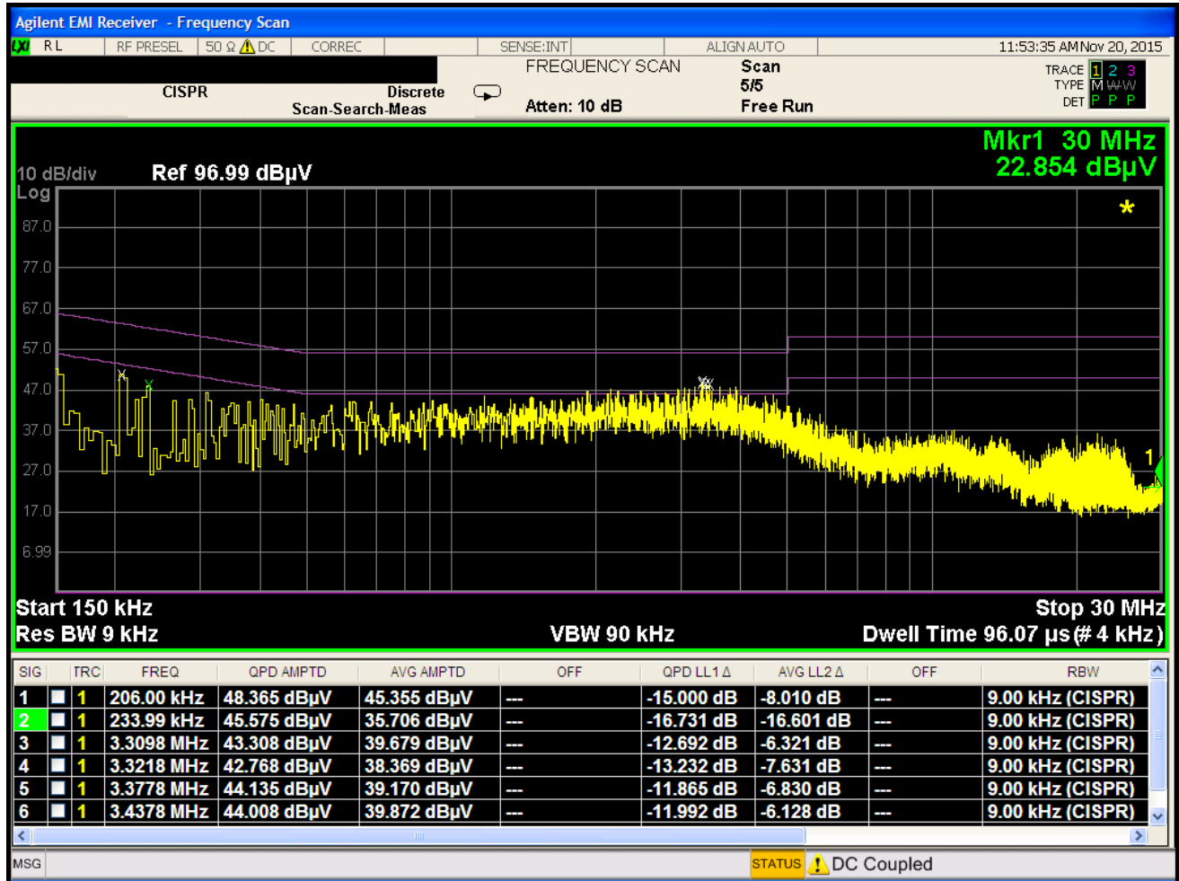
Plot 7-56. Line-Conducted Test Plot (L1) Additional AC Adapter EAY64329102
