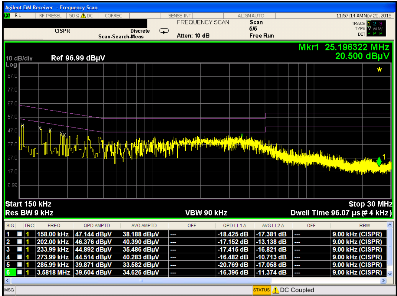
Plot 7-57. Line-Conducted Test Plot (N) Additional AC Adapter EAY64329102
