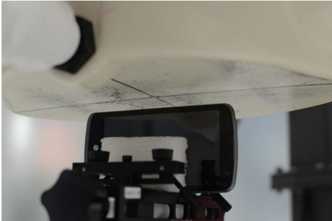
SAR Test Setup Photo 10: Left Edge 1.0 cm
