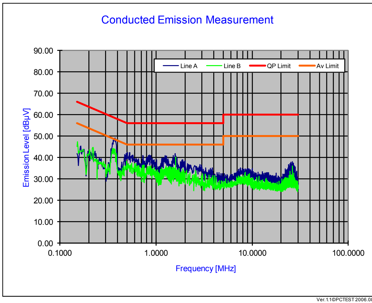
Plot 6-20. Line Conducted Plot with Bluetooth (LE)
