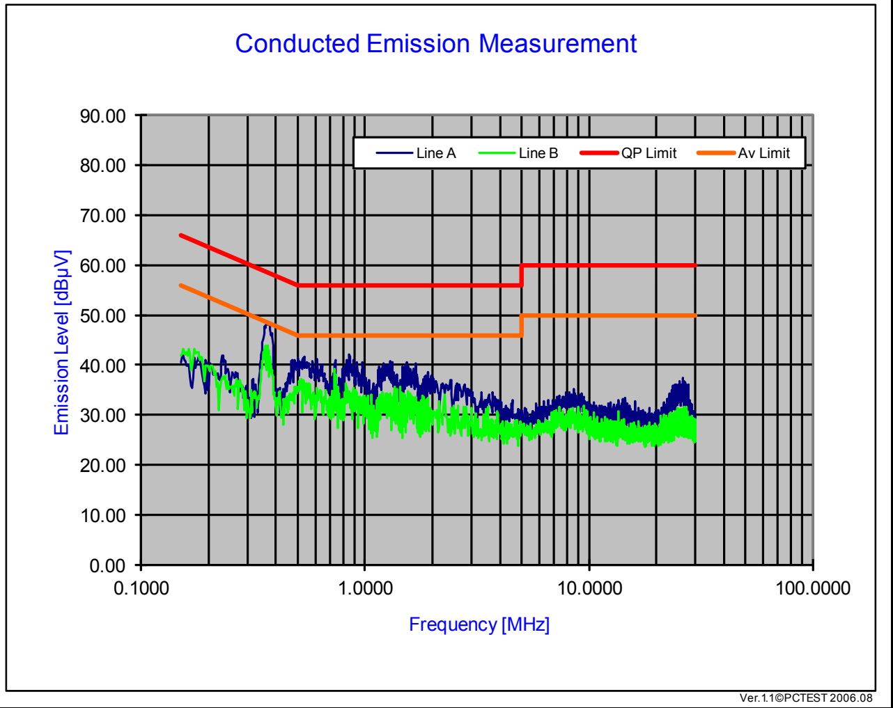
Plot 6-44. Line-Conducted Plot with Bluetooth
