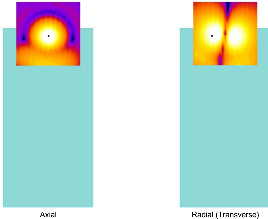
Figure 8-1 T-Coil Scan Overlay Magnetic Field Distributions
