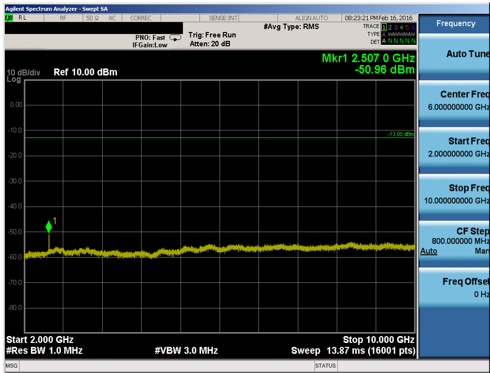
Plot 7-50. Conducted Spurious Plot (Cellular WCDMA Mode – Ch. 4183)
