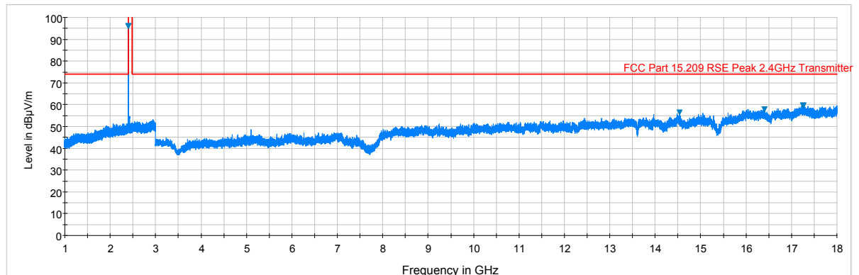
Plot 7-1. Radiated Spurious Plot above 1GHz (BT – Ch. 0, Ant. Pol. H)
