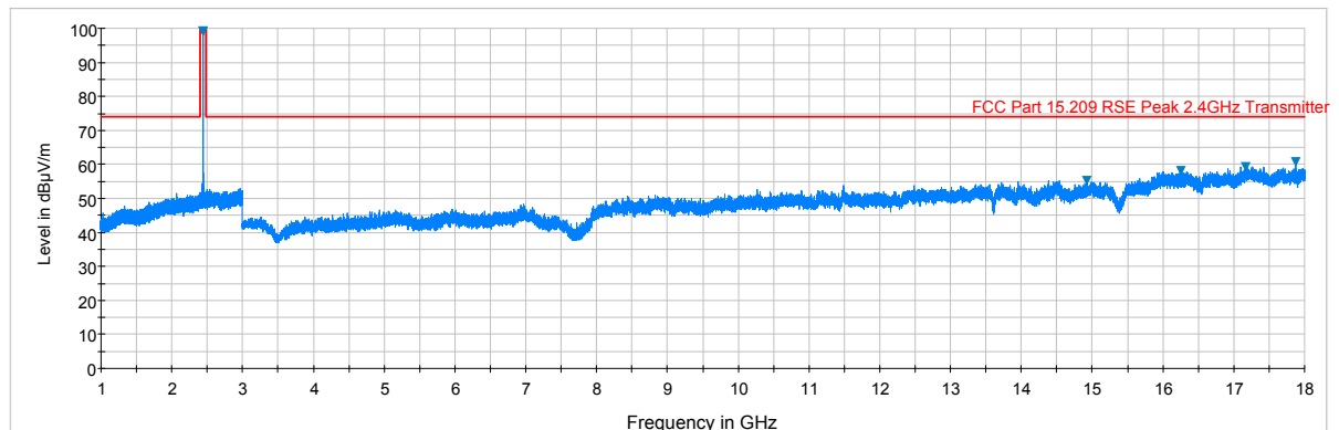
Plot 7-3. Radiated Spurious Plot above 1GHz (BT – Ch. 39, Ant. Pol. H)
