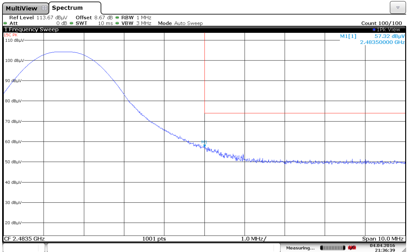
Plot 7-10. Radiated Restricted Upper Band Edge Measurement (Peak)
