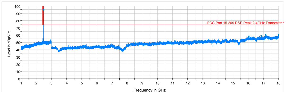
Plot 7-6. Radiated Spurious Plot above 1GHz (BT – Ch. 78, Ant. Pol. V)
