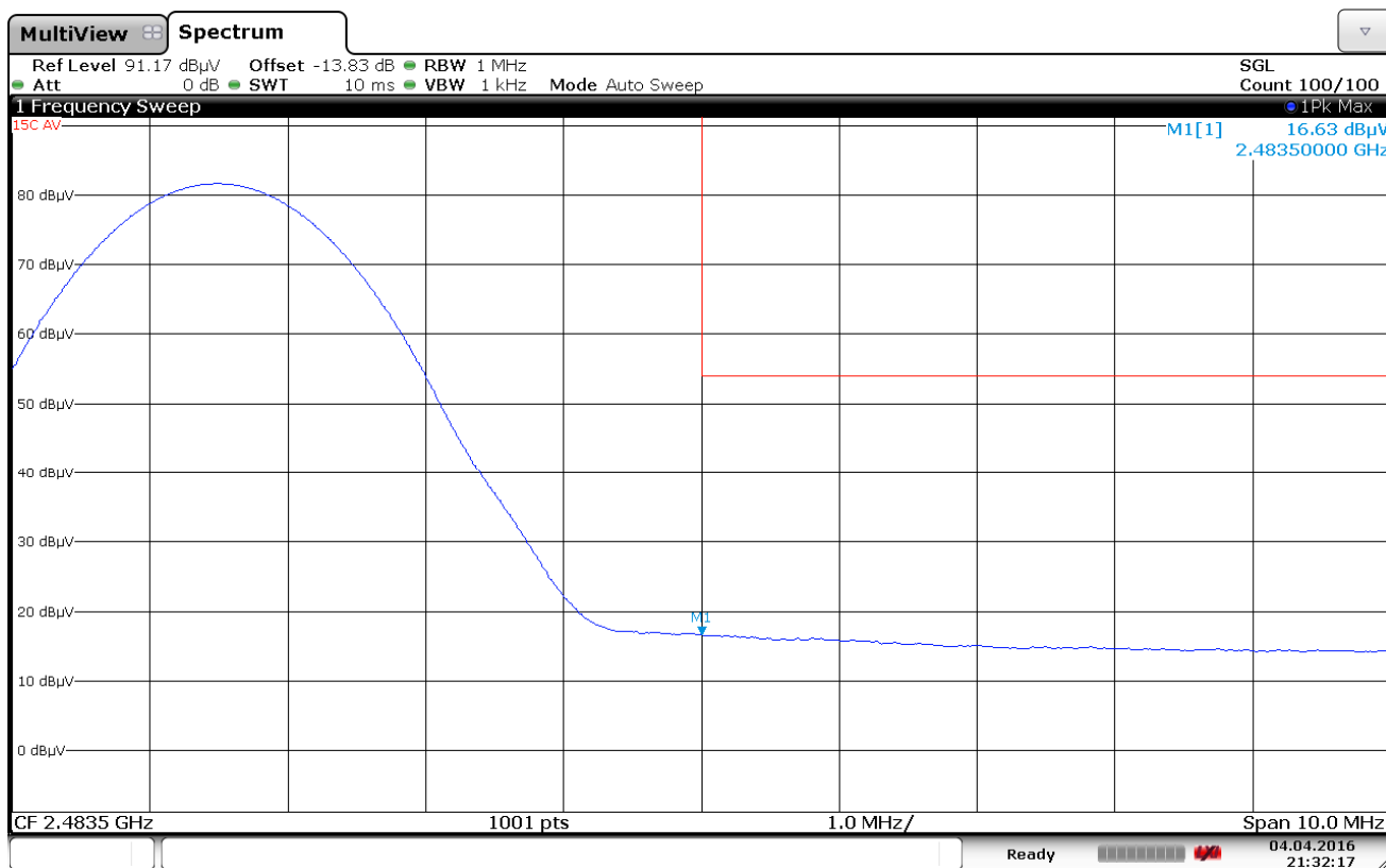
Plot 7-9. Radiated Restricted Upper Band Edge Measurement (Average)
