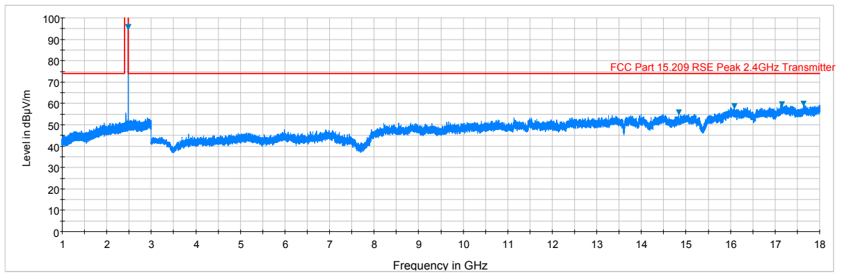
Plot 7-5. Radiated Spurious Plot above 1GHz (BT – Ch. 78, Ant. Pol. H)
