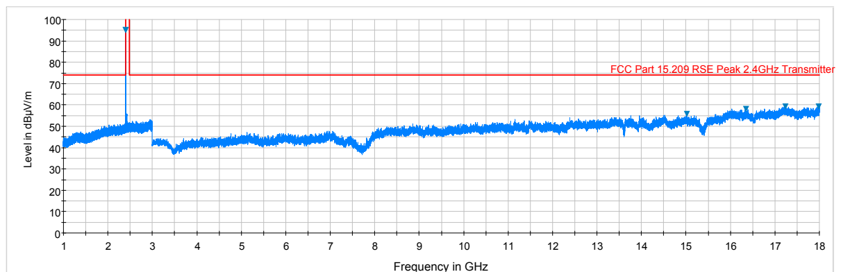
Plot 7-2. Radiated Spurious Plot above 1GHz (BT – Ch. 0, Ant. Pol. V)
