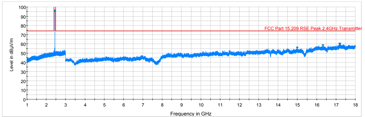
Plot 7-4. Radiated Spurious Plot above 1GHz (BT – Ch. 39, Ant. Pol. V)
