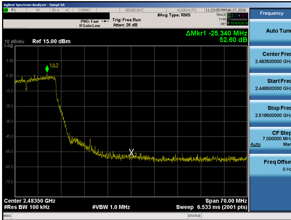
Plot 7-29. Band Edge Plot (802.11n (2.4GHz) – Ch. 9)
