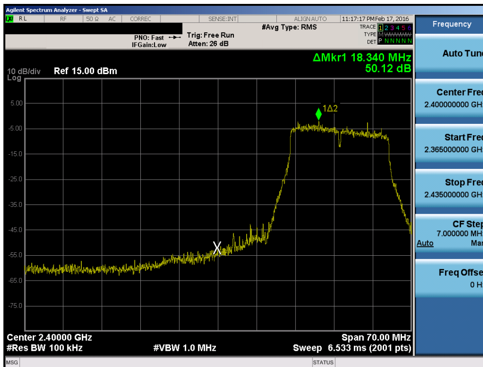
Plot 7-28. Band Edge Plot (802.11n (2.4GHz) – Ch. 3)
