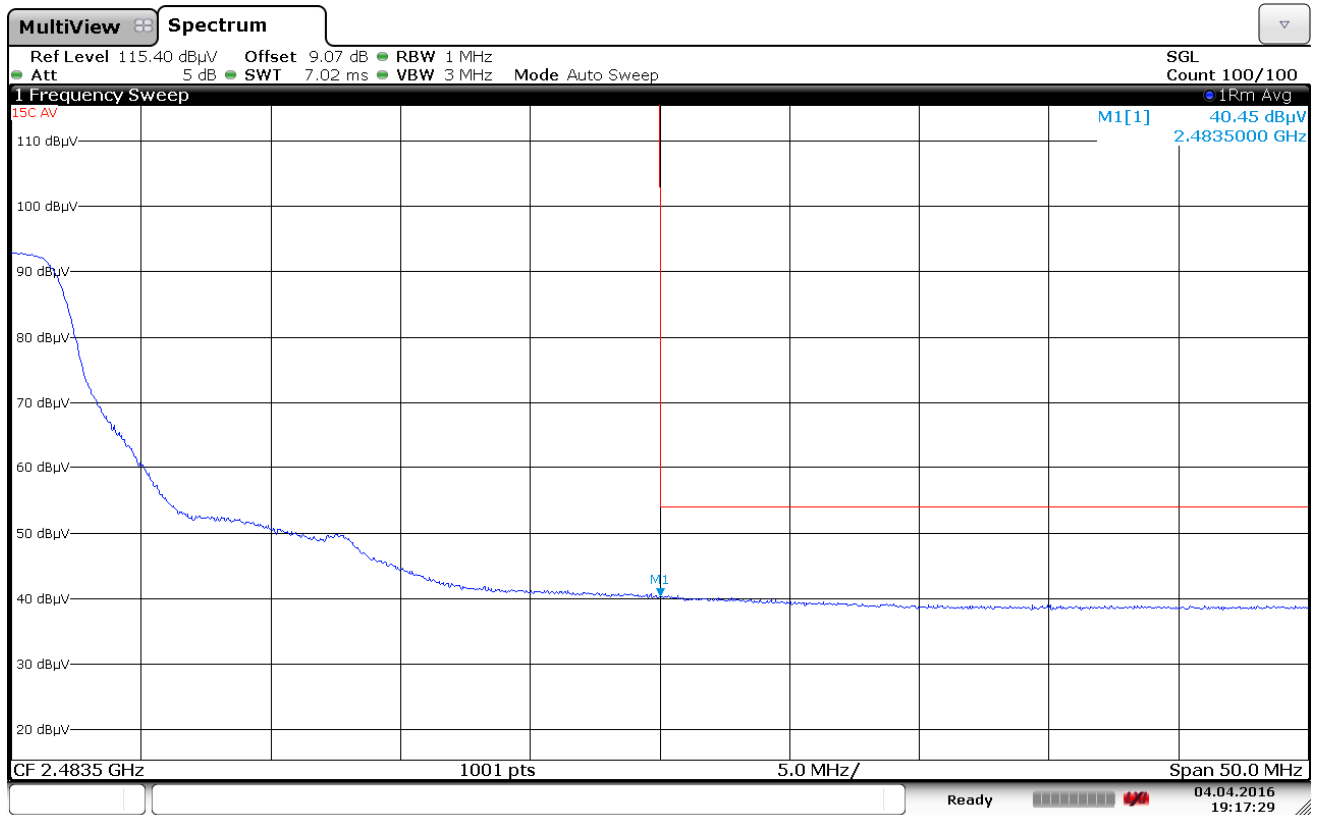
Plot 7-13. Radiated Restricted Upper Band Edge Measurement (Average)
