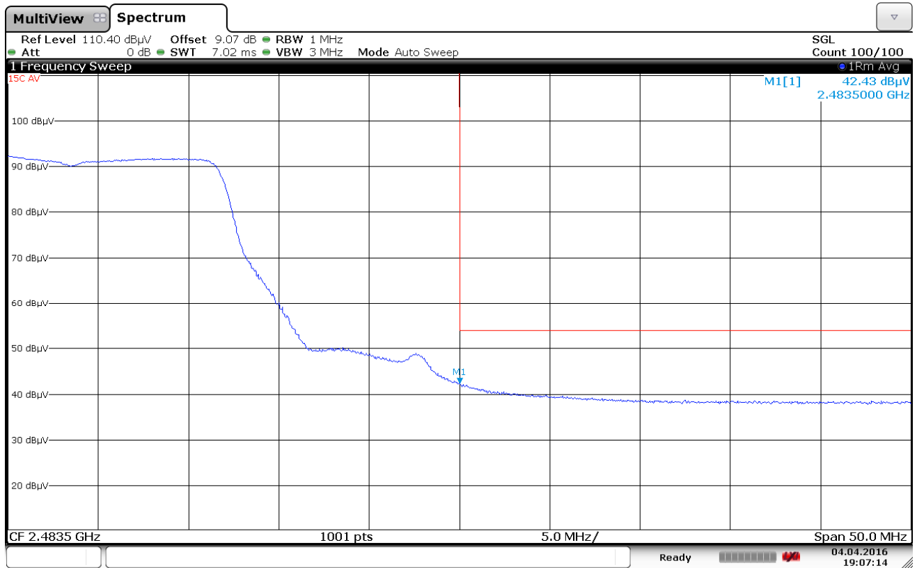
Plot 7-15. Radiated Restricted Upper Band Edge Measurement (Average)
