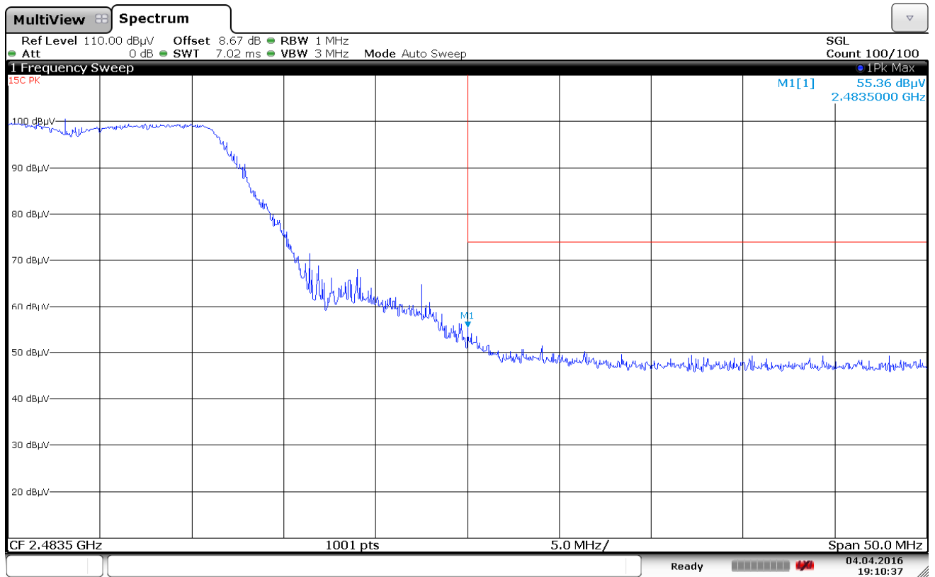
Plot 7-16. Radiated Restricted Upper Band Edge Measurement (Peak)
