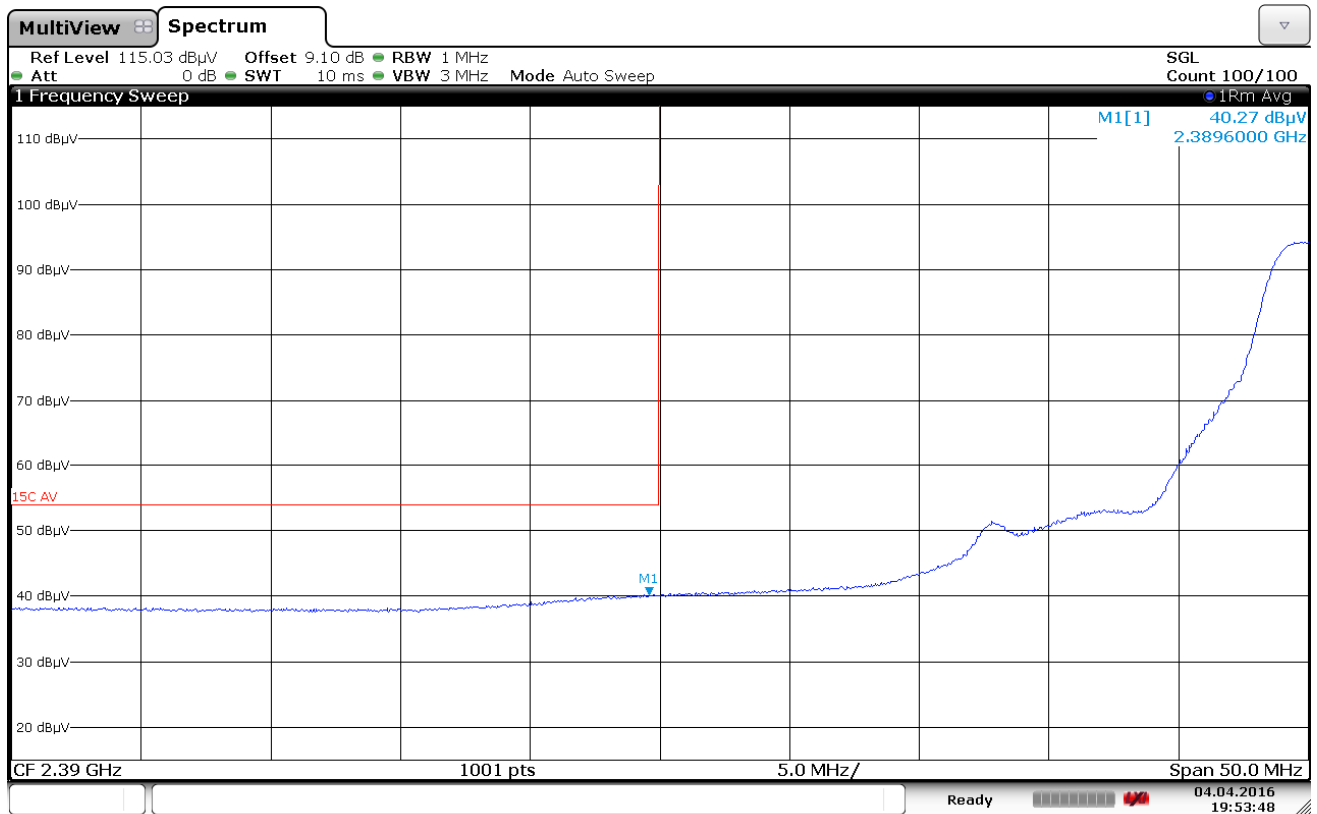
Plot 7-11. Radiated Restricted Lower Band Edge Measurement (Average)
