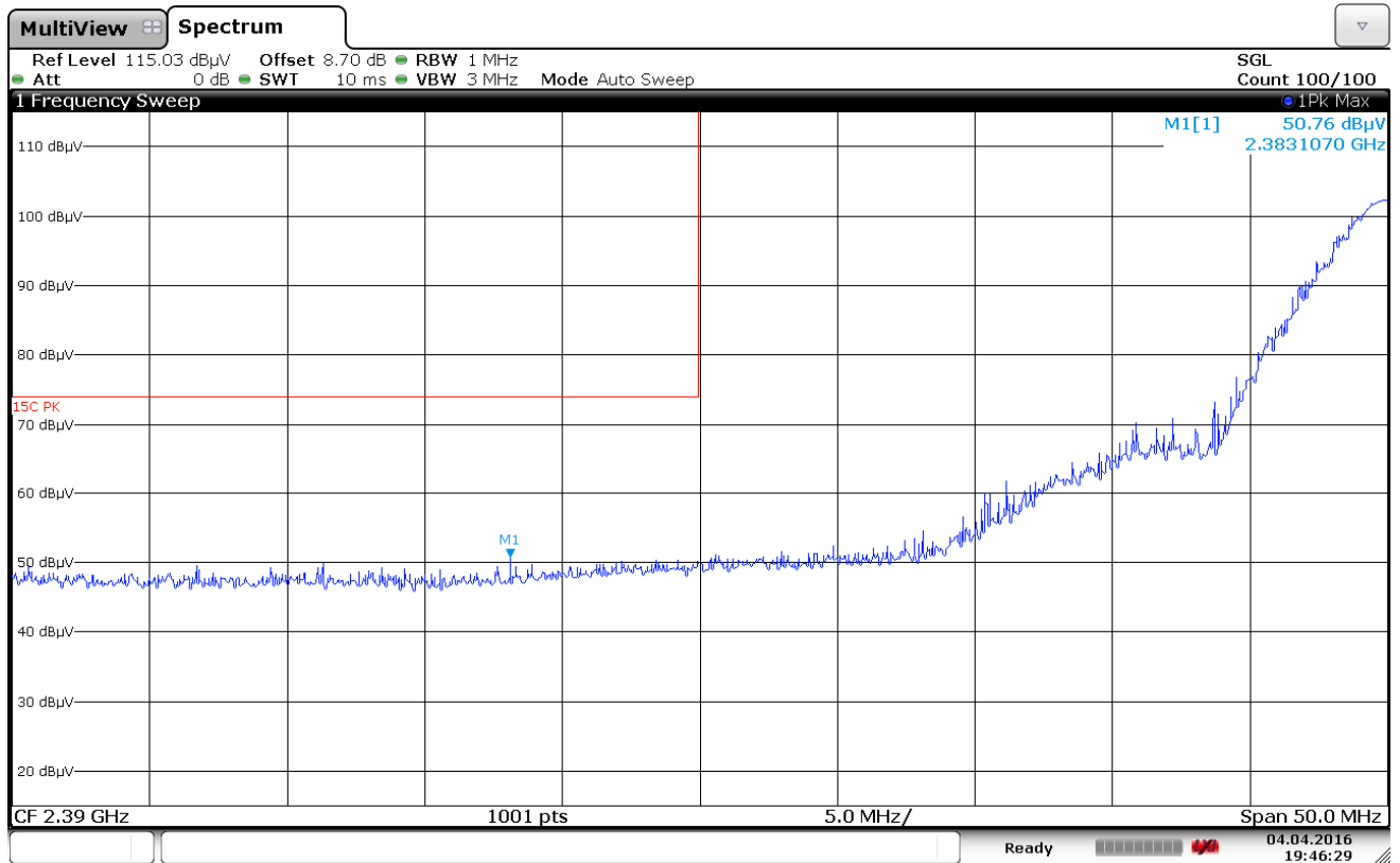
Plot 7-12. Radiated Restricted Lower Band Edge Measurement (Peak)
