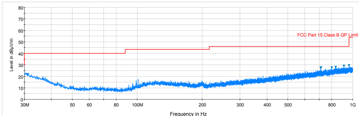
Plot 7-17. Radiated Spurious Plot below 1GHz (Pol. H)
