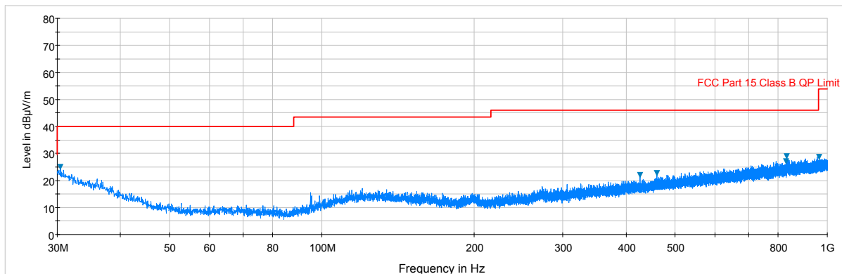
Plot 7-18. Radiated Spurious Plot below 1GHz (Pol. V)
