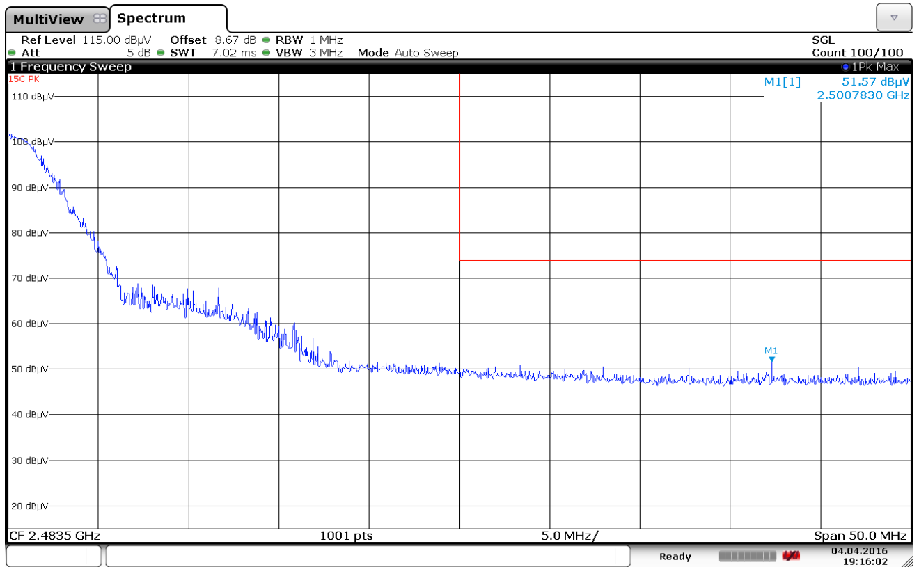
Plot 7-14. Radiated Restricted Upper Band Edge Measurement (Peak)
