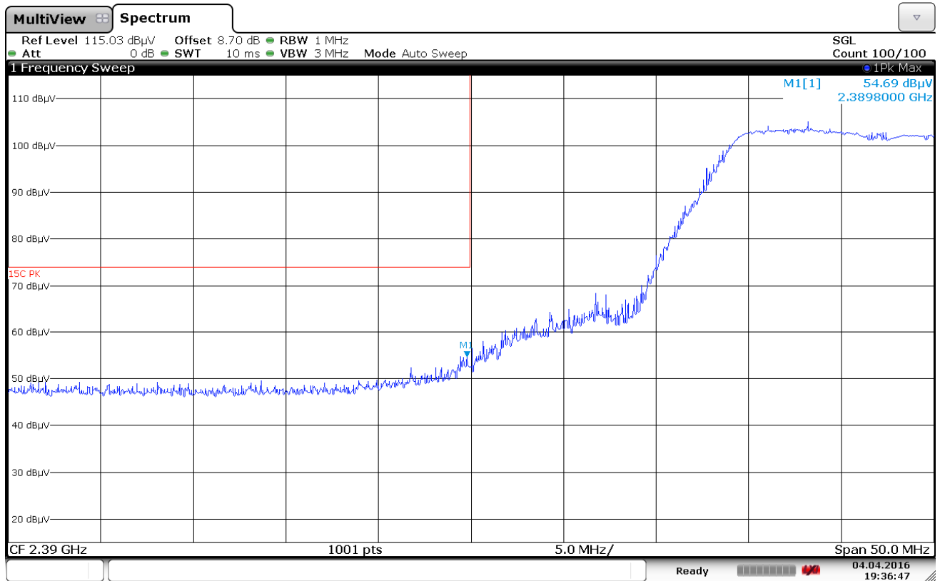
Plot 7-10. Radiated Restricted Lower Band Edge Measurement (Peak)
