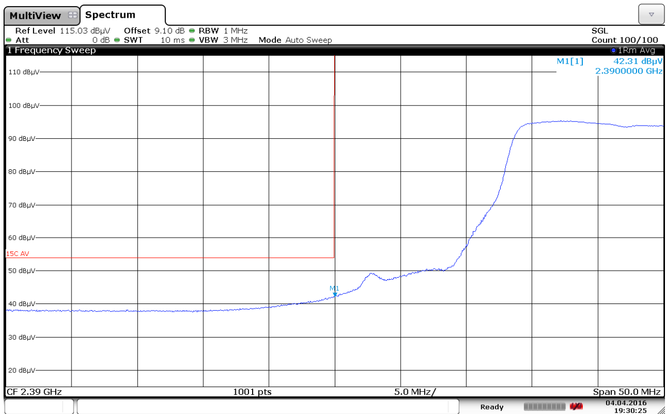
Plot 7-9. Radiated Restricted Lower Band Edge Measurement (Average)
