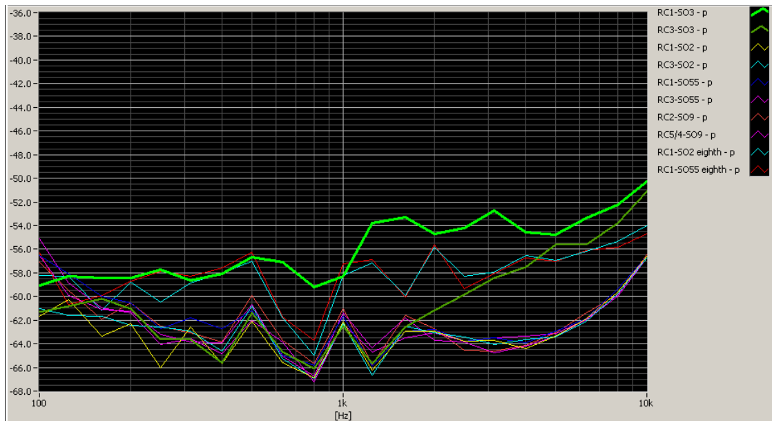
Figure 6-1 CDMA Audio Band Magnetic Noise
