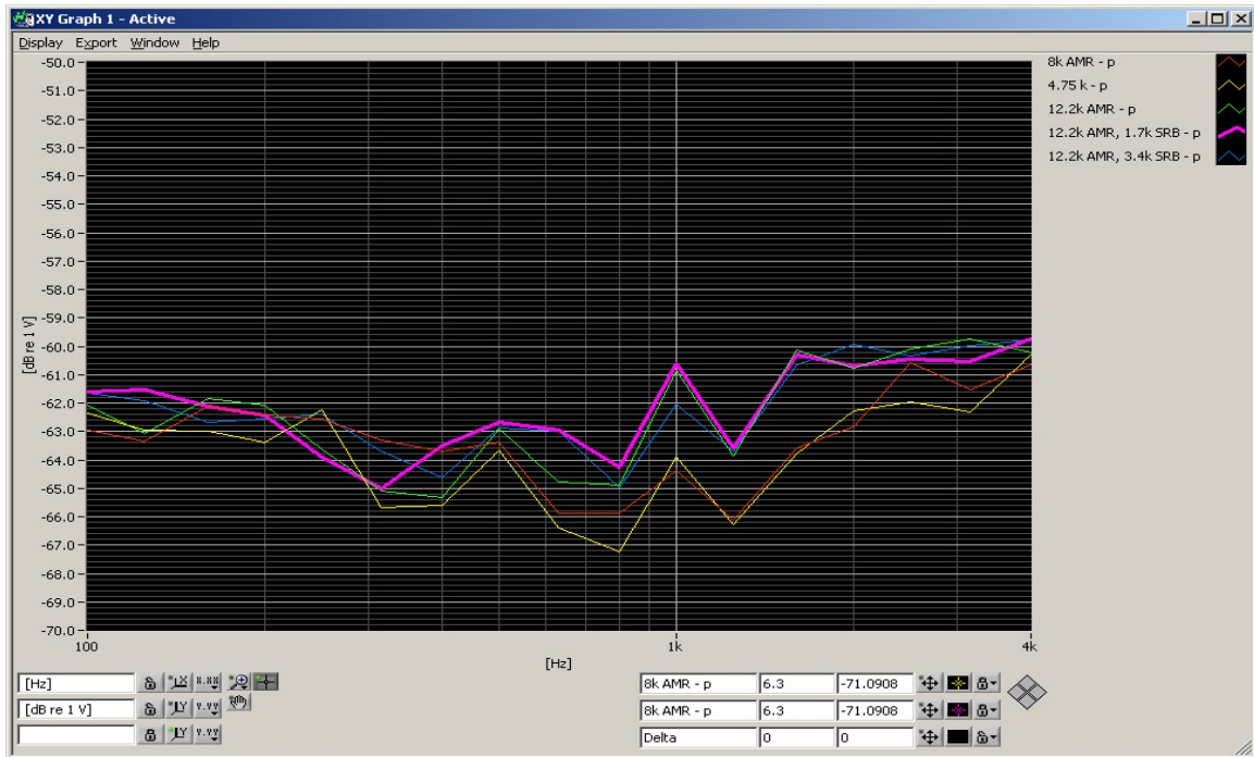
Figure 6-3 UMTS Audio Band Magnetic Noise
