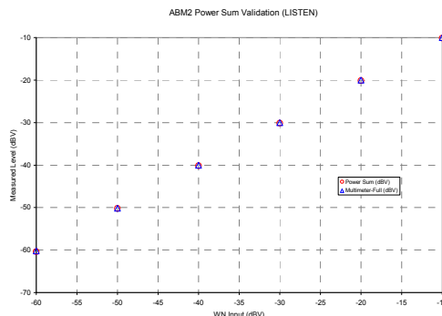
Figure 4-10 ABM2 Power Sum Validation
