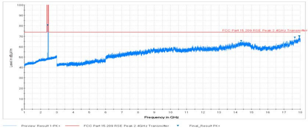
Plot 7-46. Radiated Spurious Plot above 1GHz (BT – Ch. 78, Ant. Pol. H)
