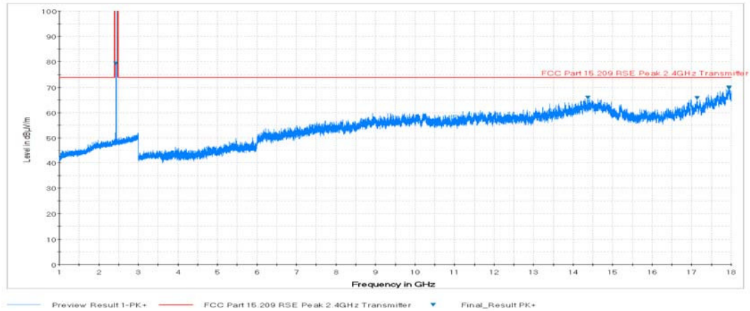
Plot 7-45. Radiated Spurious Plot above 1GHz (BT – Ch. 39, Ant. Pol. V)
