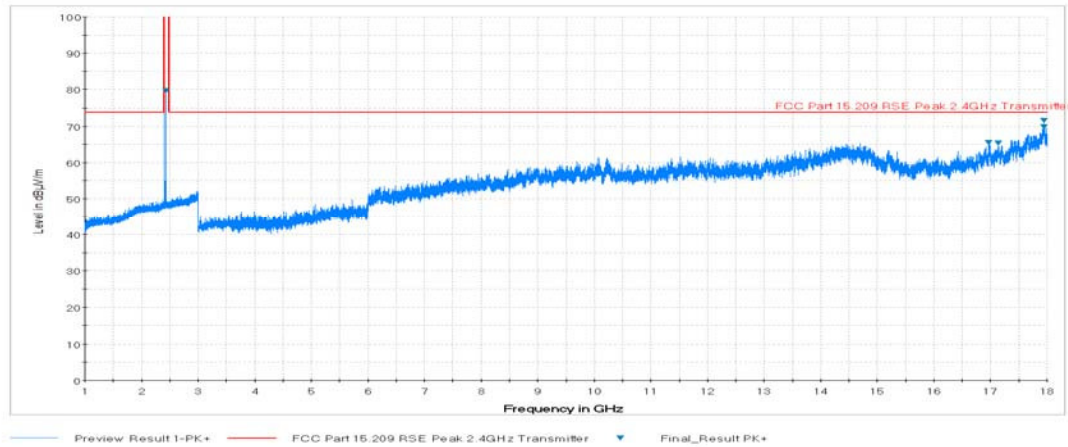
Plot 7-43. Radiated Spurious Plot above 1GHz (BT – Ch. 0, Ant. Pol. V)
