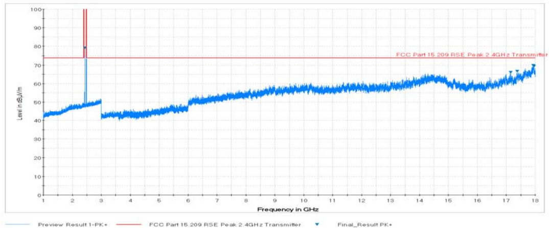
Plot 7-47. Radiated Spurious Plot above 1GHz (BT – Ch. 78, Ant. Pol. V)
