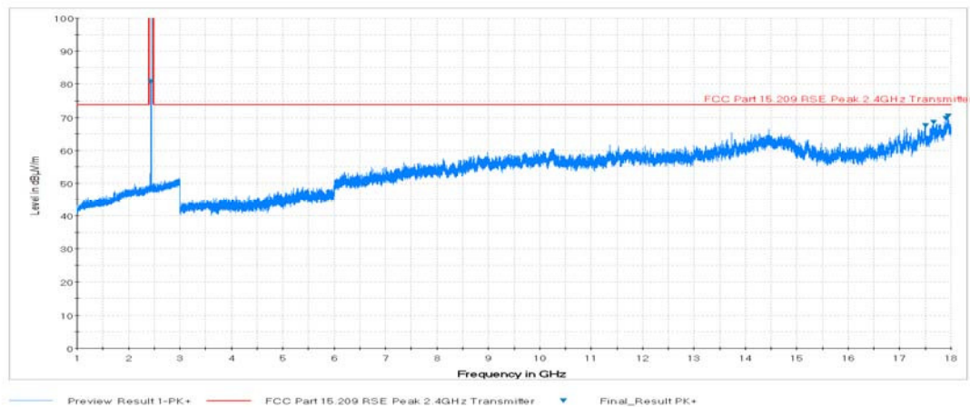
Plot 7-44. Radiated Spurious Plot above 1GHz (BT – Ch. 39, Ant. Pol. H)
