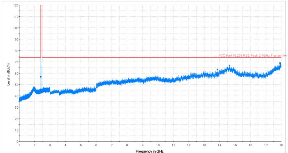
Plot 7-1. Radiated Spurious Plot above 1GHz (BT – Ch. 0, Ant. Pol. H)
