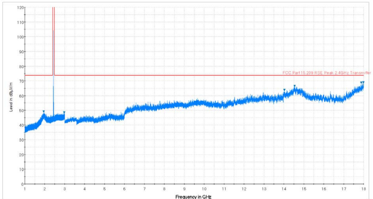
Plot 7-3. Radiated Spurious Plot above 1GHz (BT – Ch. 39, Ant. Pol. H)
