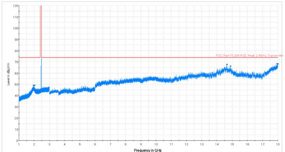
Plot 7-5. Radiated Spurious Plot above 1GHz (BT – Ch. 78, Ant. Pol. H)
