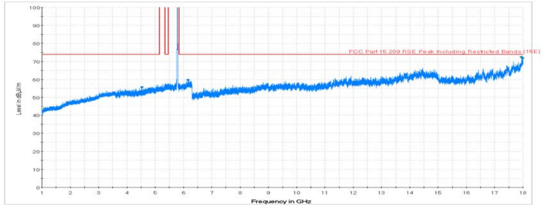
Plot 7-73. Radiated Spurious Plot above 1GHz (802.11a – U3 Ch. 157, Ant. Pol. H)
