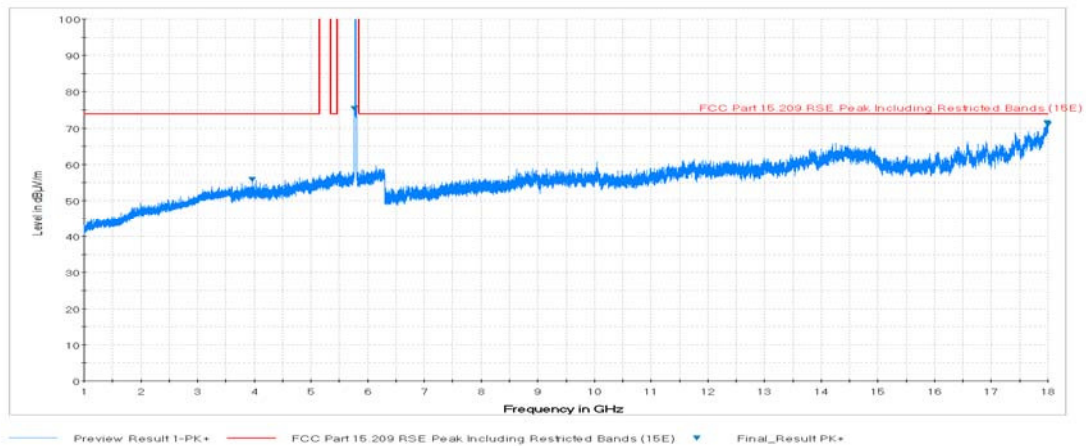
Plot 7-74. Radiated Spurious Plot above 1GHz (802.11a – U3 Ch. 157, Ant. Pol. V)
