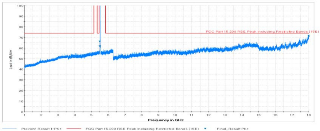
Plot 7-72. Radiated Spurious Plot above 1GHz (802.11a – U2C Ch. 116, Ant. Pol. V)
