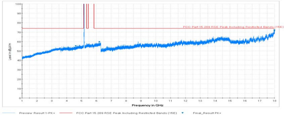
Plot 7-67. Radiated Spurious Plot above 1GHz (802.11a – U1 Ch. 40, Ant. Pol. H)
