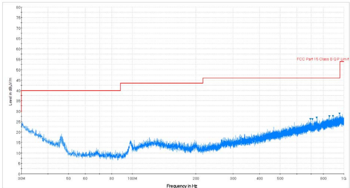
Plot 7-94. Radiated Spurious Plot below 1GHz (802.11a – U3 Ch. 157, Ant. Pol. V)
