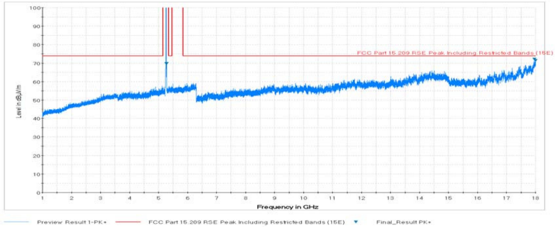
Plot 7-70. Radiated Spurious Plot above 1GHz (802.11a – U2A Ch. 56, Ant. Pol. V)
