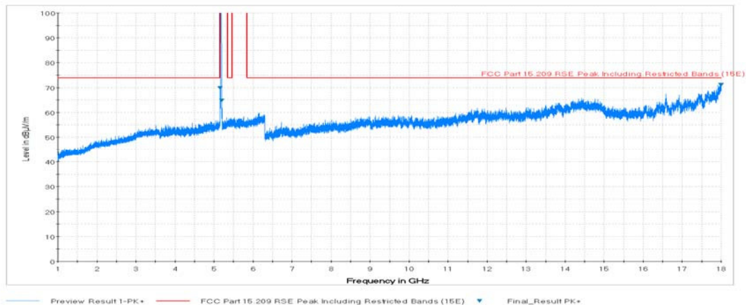
Plot 7-68. Radiated Spurious Plot above 1GHz (802.11a – U1 Ch. 40, Ant. Pol. V)
