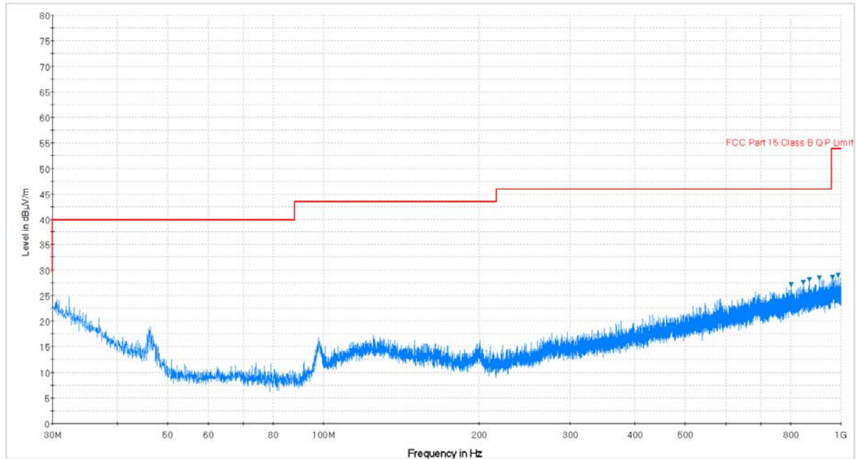
Plot 7-93. Radiated Spurious Plot below 1GHz (802.11a – U3 Ch. 157, Ant. Pol. H)
