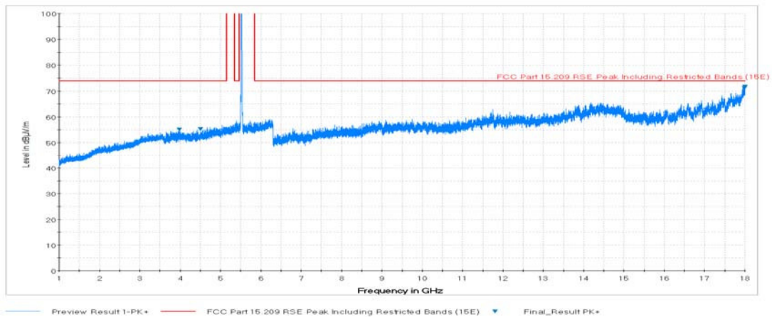
Plot 7-71. Radiated Spurious Plot above 1GHz (802.11a – U2C Ch. 116, Ant. Pol. H)
