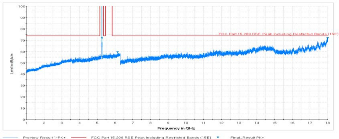
Plot 7-69. Radiated Spurious Plot above 1GHz (802.11a – U2A Ch. 56, Ant. Pol. H)
