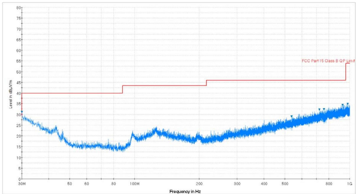
Plot 7-28. Radiated Spurious Plot below 1GHz (802.11a – U3 Ch. 157, Ant. Pol. V)
