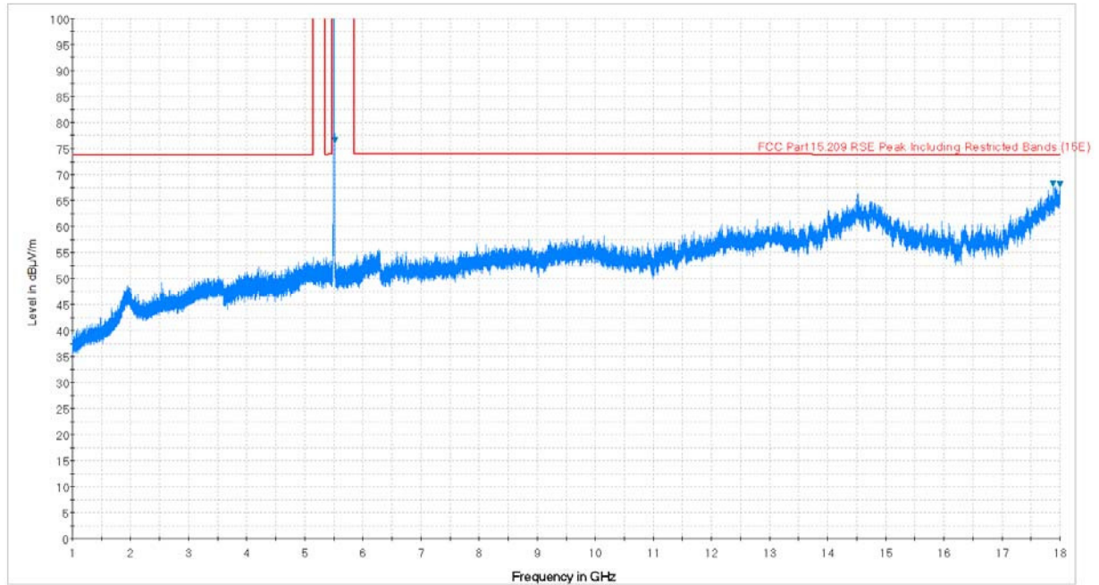
Plot 7-5. Radiated Spurious Plot above 1GHz (802.11a – U2C Ch. 116, Ant. Pol. H)
