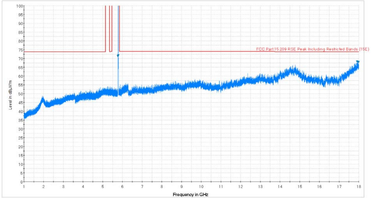
Plot 7-7. Radiated Spurious Plot above 1GHz (802.11a – U3 Ch. 157, Ant. Pol. H)
