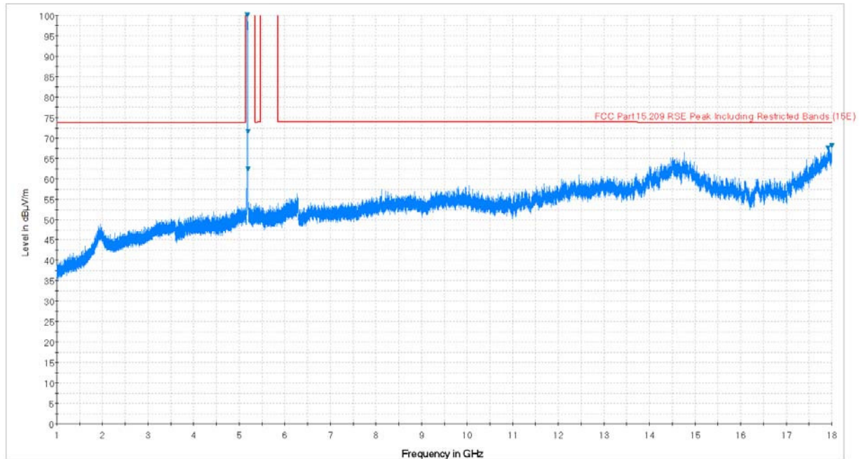
Plot 7-2. Radiated Spurious Plot above 1GHz (802.11a – U1 Ch. 40, Ant. Pol. V)
