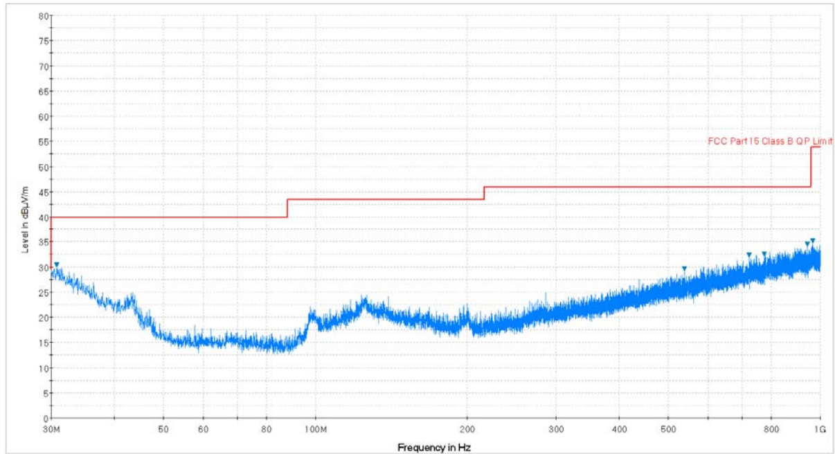
Plot 7-27. Radiated Spurious Plot below 1GHz (802.11a – U3 Ch. 157, Ant. Pol. H)
