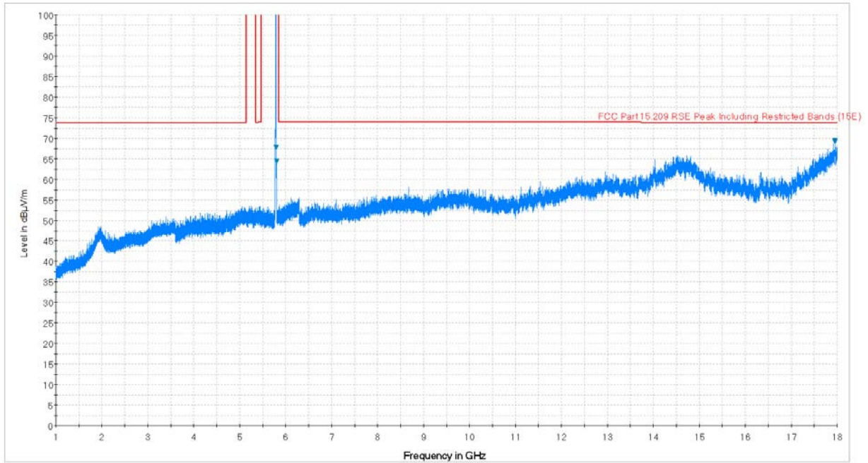
Plot 7-8. Radiated Spurious Plot above 1GHz (802.11a – U3 Ch. 157, Ant. Pol. V)
