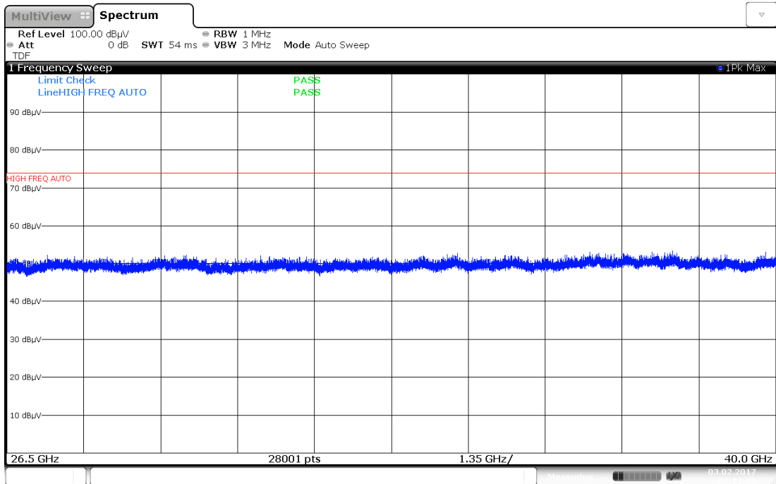
Plot 7-11. Radiated Spurious Plot 26.5GHz - 40GHz (802.11a – Ant. Pol. H)
