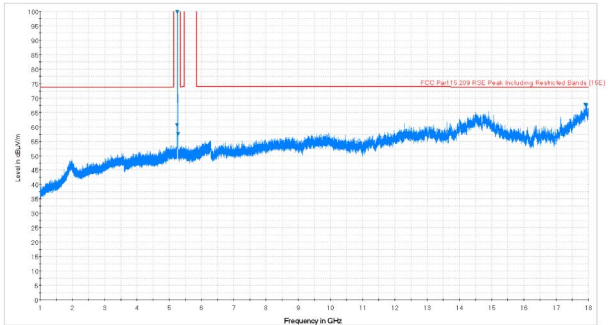
Plot 7-4. Radiated Spurious Plot above 1GHz (802.11a – U2A Ch. 56, Ant. Pol. V)
