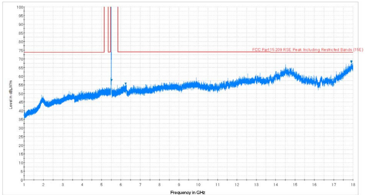
Plot 7-6. Radiated Spurious Plot above 1GHz (802.11a – U2C Ch. 116, Ant. Pol. V)
