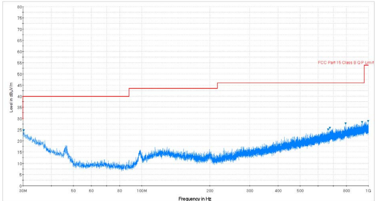
Plot 7-43. Radiated Spurious Plot below 1GHz (Pol. H)
