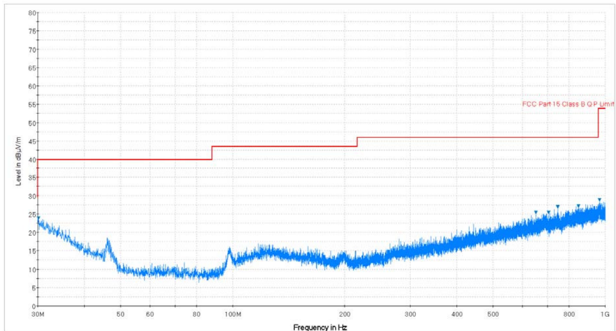
Plot 7-44. Radiated Spurious Plot below 1GHz (Pol. V)
