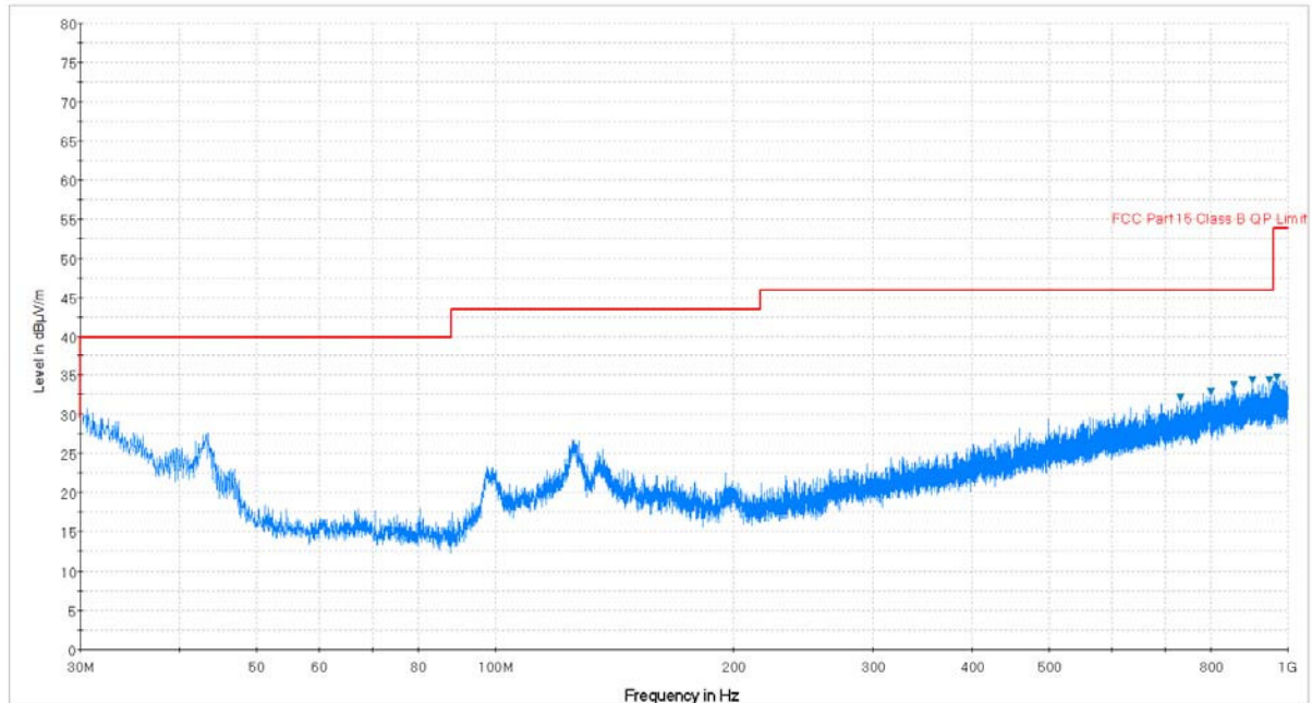
Plot 7-13. Radiated Spurious Plot below 1GHz (Pol. H)
