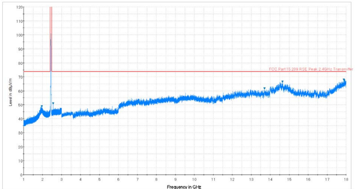
Plot 7-3. Radiated Spurious Plot above 1GHz (802.11b – Ch. 6, Ant. Pol. H)
