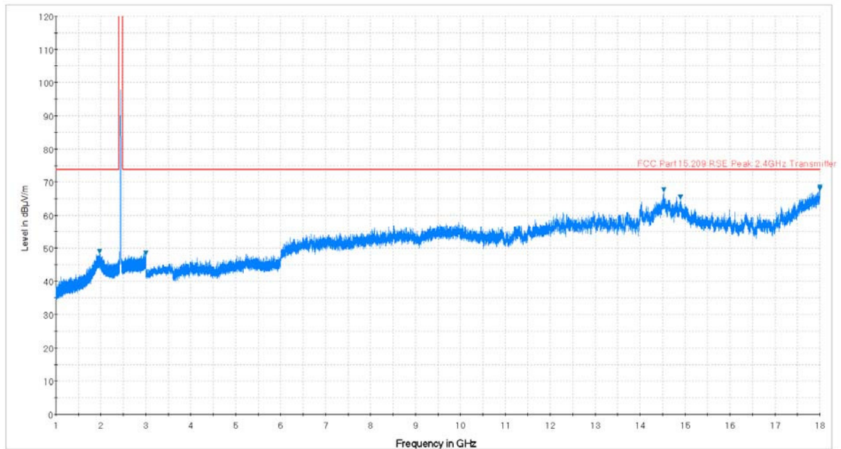
Plot 7-4. Radiated Spurious Plot above 1GHz (802.11b – Ch. 6, Ant. Pol. V)
