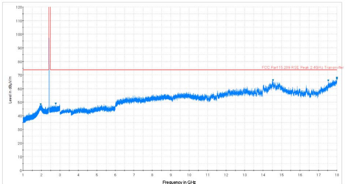
Plot 7-2. Radiated Spurious Plot above 1GHz (802.11b – Ch. 1, Ant. Pol. V)
