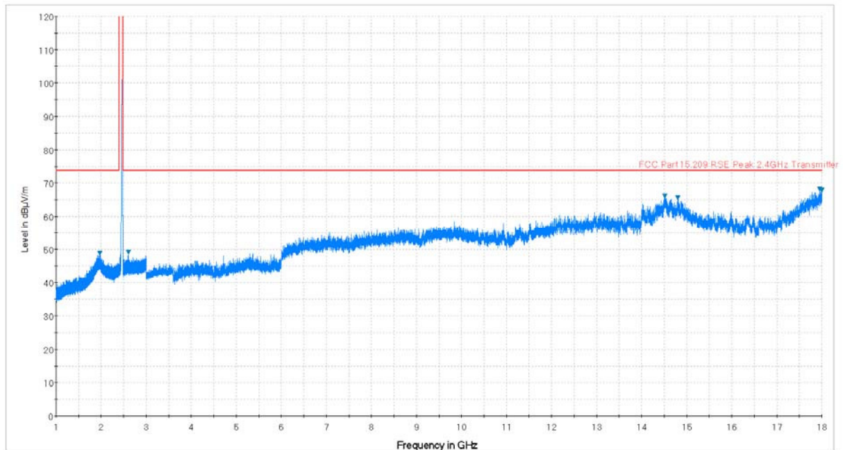
Plot 7-5. Radiated Spurious Plot above 1GHz (802.11b – Ch. 11, Ant. Pol. H)
