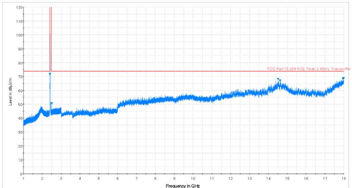
Plot 7-1. Radiated Spurious Plot above 1GHz (802.11b – Ch. 1, Ant. Pol. H)
