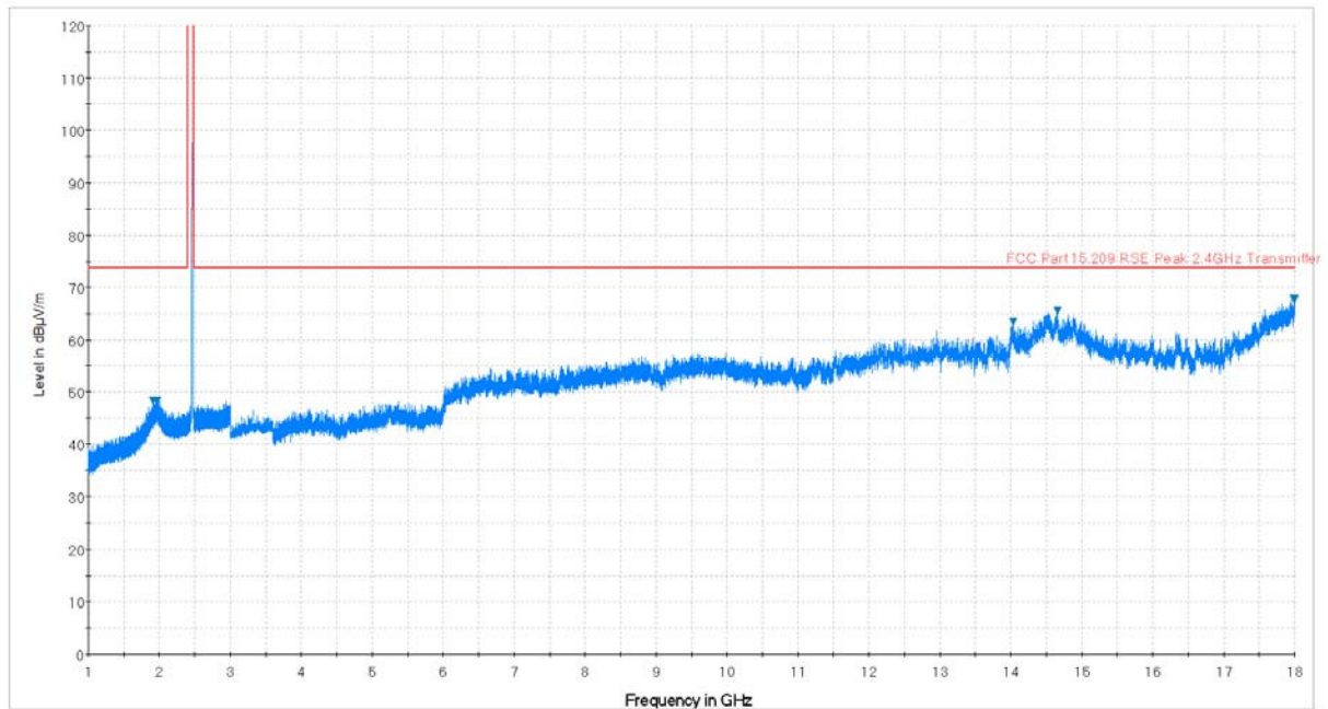
Plot 7-6. Radiated Spurious Plot above 1GHz (802.11b – Ch. 11, Ant. Pol. V)
