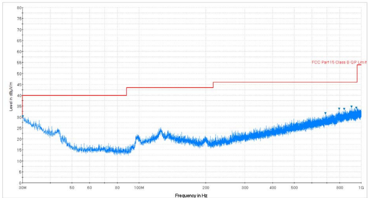
Plot 7-14. Radiated Spurious Plot below 1GHz (Pol. V)
