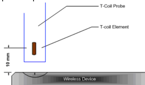
Figure 4-11 Measurement Distance
