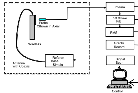
Figure 4-14 Audio Magnetic Field Test Setup
